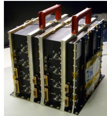
NASA Navigator SSV Receiver
