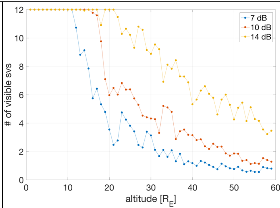
Number of satellites visible by altitude for different antenna gains
