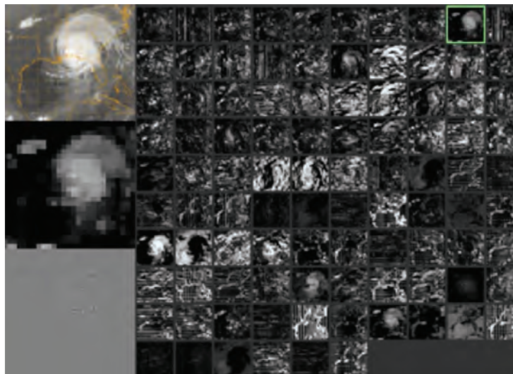
FIGURE 1. First convolution output for a GOES IR with hurricane. Top left: Inset is input image from NRL. Middle left: Example feature map for highlighted box (green).
