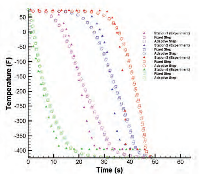
FIGURE 1. Transient temperature for the subcooled LH 2 for the driving pressure 111.69 psia at four stations.
