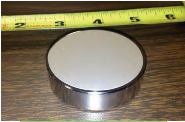
FIGURE 2. The first hybrid ceramic optic was produced on a 2-in-diameter flat. The low-frequency figure of the sample appeared to be negatively influenced by the shrinkage mismatch between the ceramic and electroformed NiCo, however.
