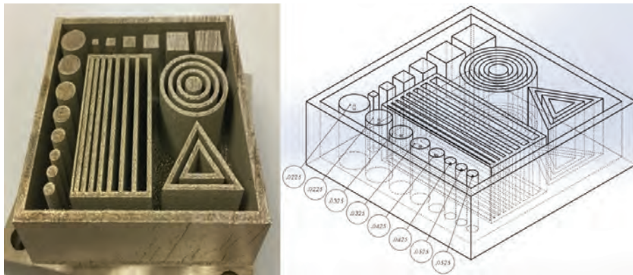
FIGURE 1. CAD model and SLM IN-718 build showing subsurface defects.
