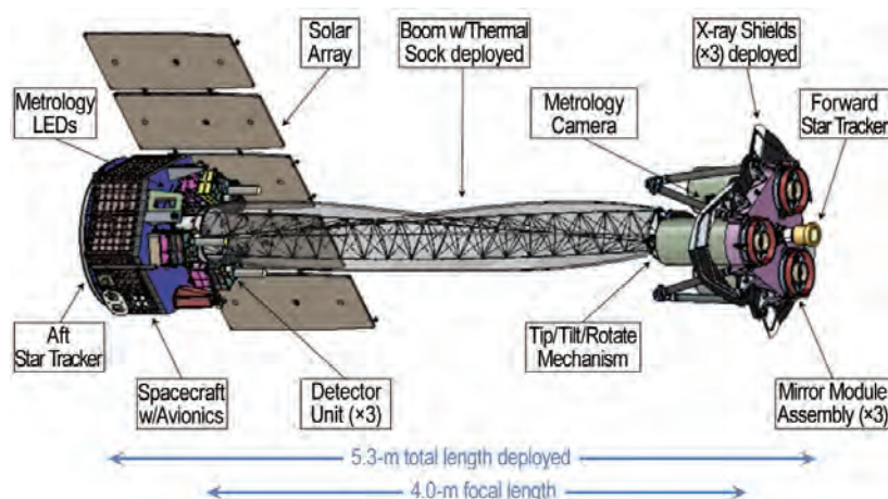
FIGURE 1. IXPE deployed.
