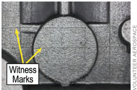
FIGURE 1. SLM component with witness marks.
