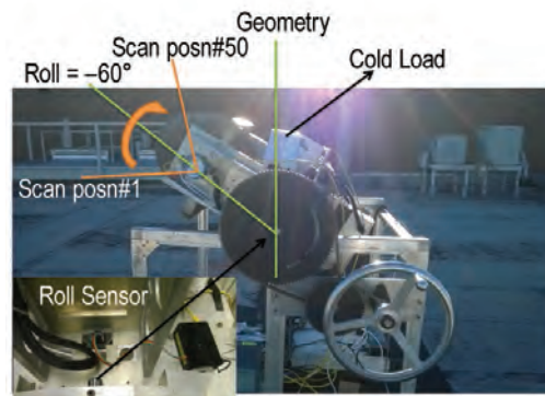
FIGURE 1. AMPR instrument in cart modified to rotate the instrument independently of azimuthal scan angle. Note the hand crank to accomplish the rotation. AMPR is rotated 60° from zenith, with scan range shown.
