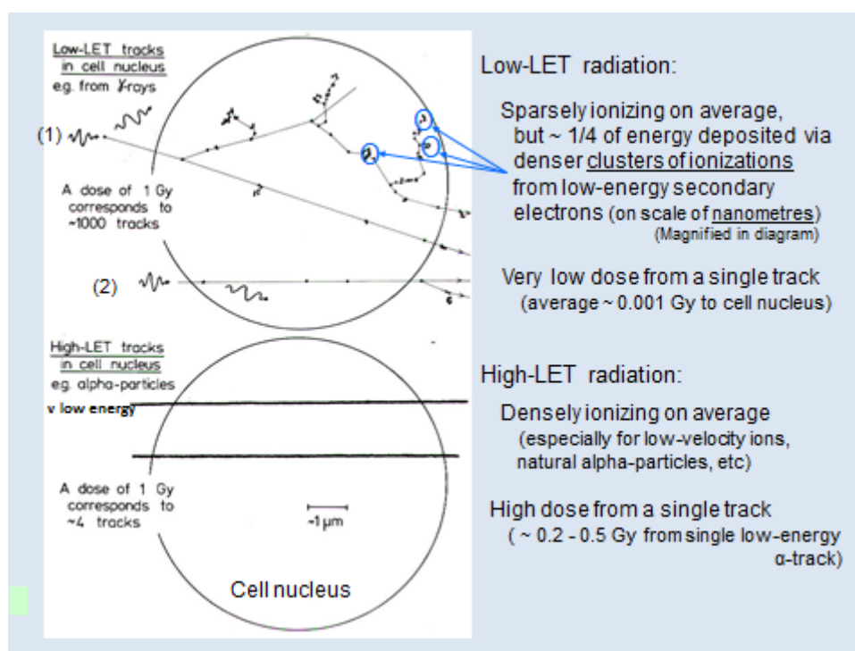
Figure 2a. Schematic diagram of two tracks of electrons from \gamma -ray interactions (upper portion) or of two low-energy alpha particles from radionuclide decay (lower part) passing through a cell nucleus of diameter 8 \mu\text{m} . (Adapted from Goodhead 1994.)
