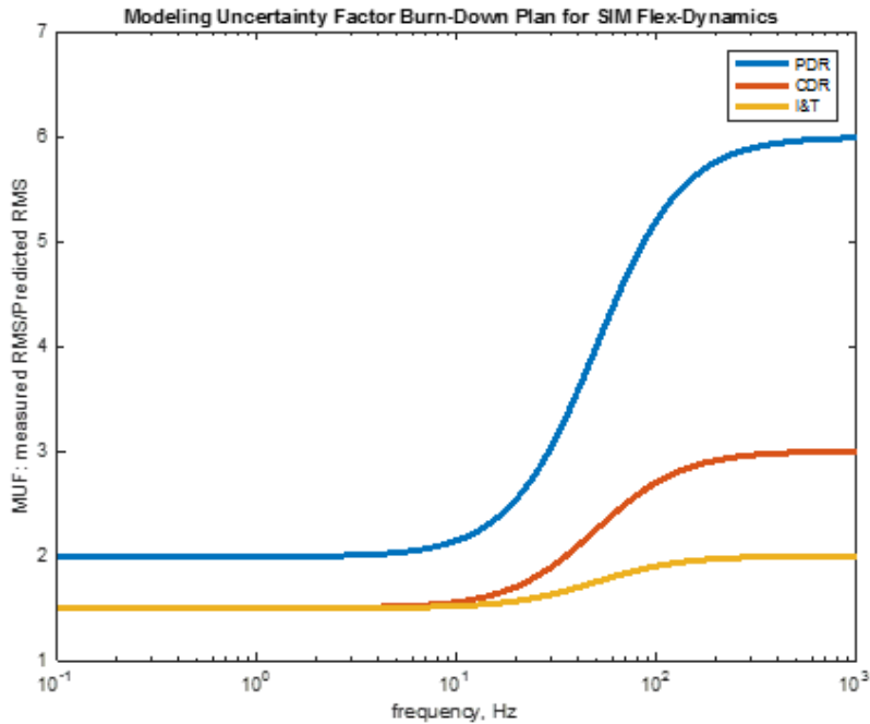
Figure 3. SIM flight system modeling uncertainty factors for flexible dynamics.
