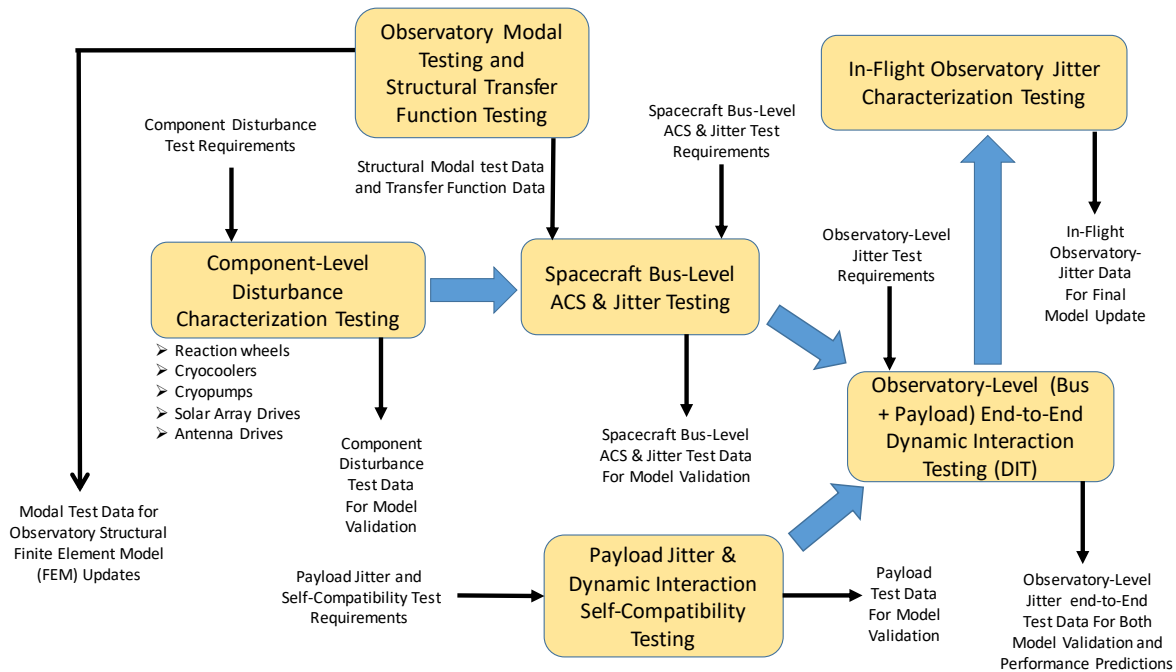
Figure 7. A recommended jitter testing campaign to support model validation and performance predictions.
