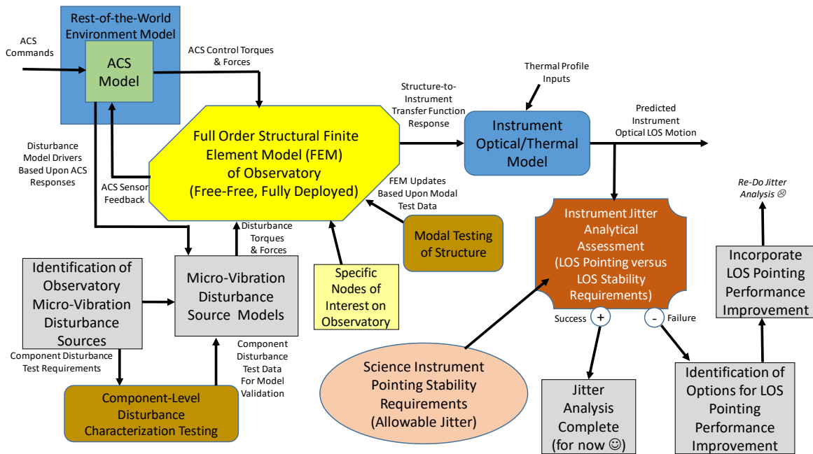
Figure 5. Typical high-level observatory micro-vibration (jitter) analysis process.
