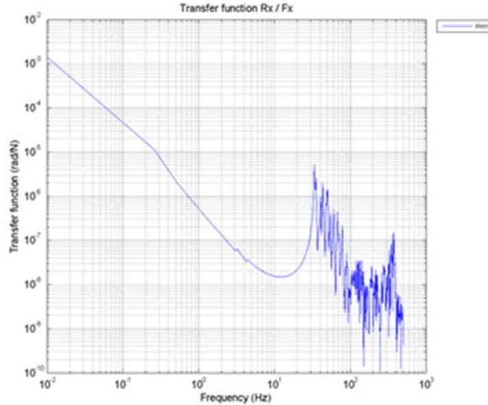
Figure 6. Representative example of a structural transfer function between a rw force component and a rotational component of an instrument LOS (from [36]).
