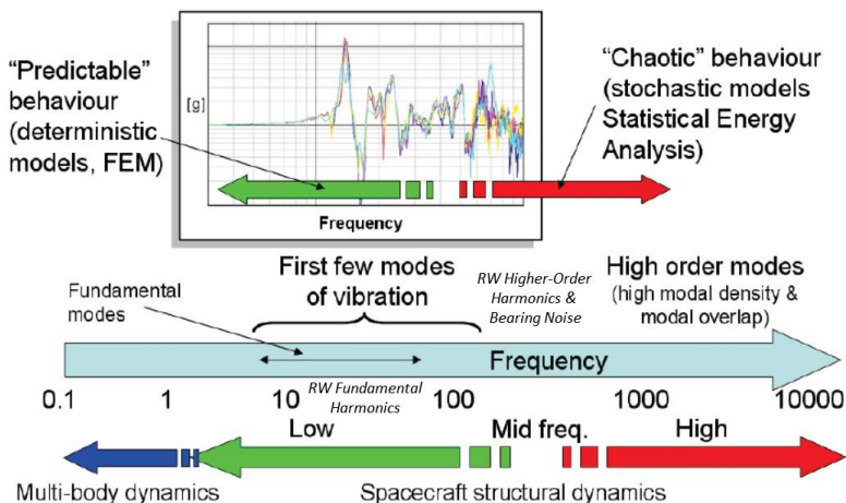
Figure 2. Spacecraft dynamic behavior and analysis methodologies over broad frequency range (from Ref. [1]).
