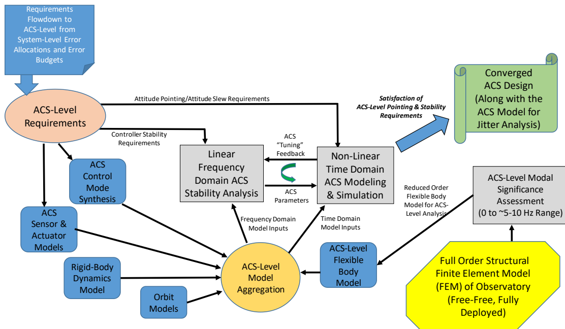
Figure 4. Typical high-level acs analysis and design process.
