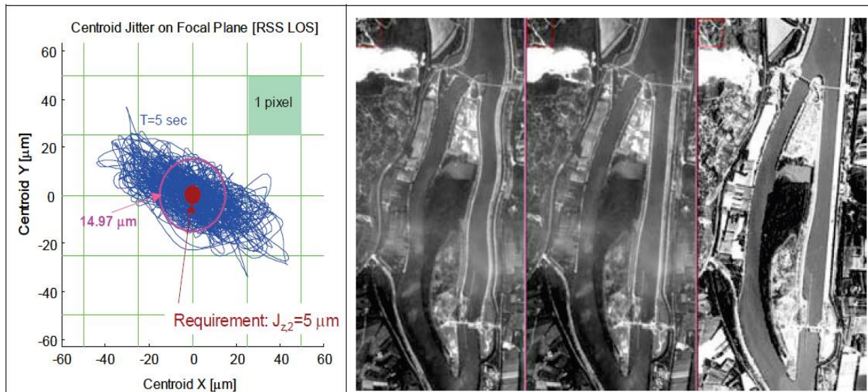
Figure 1. Example of LOS pointing errors and the resulting effects on image quality (from Ref. [1]).
