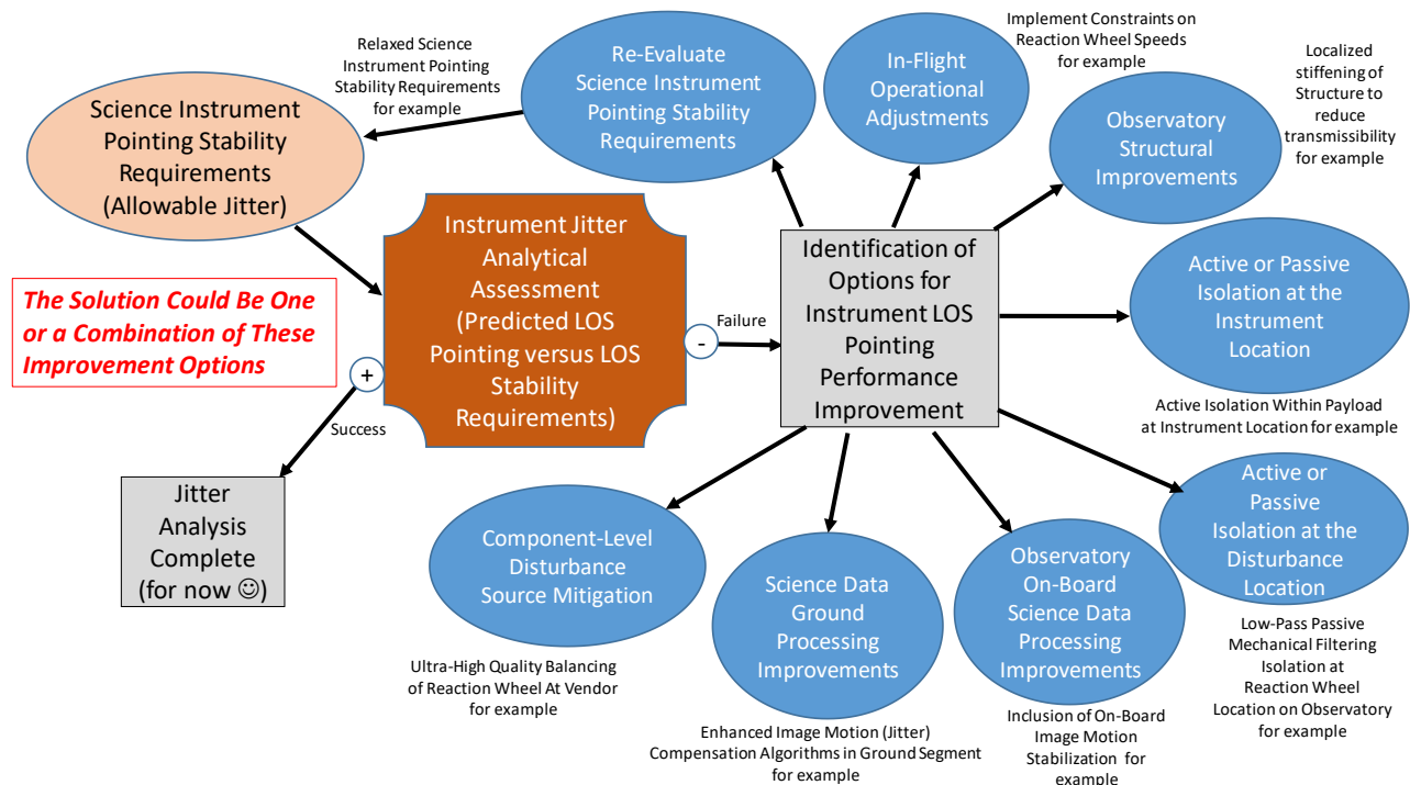
Figure 8. Possible options for improving instrument LOS jitter performance.
