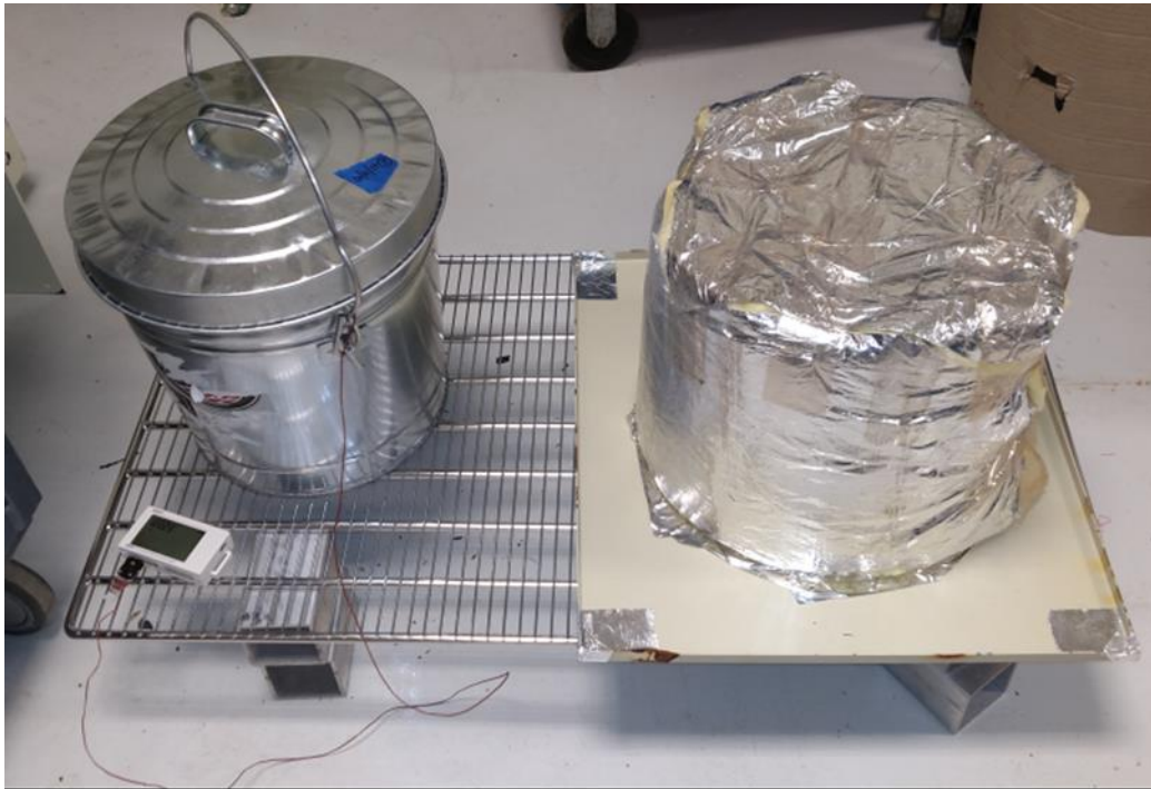
Figure 5: Thermal mass (left) and End cooler (right) concepts.
