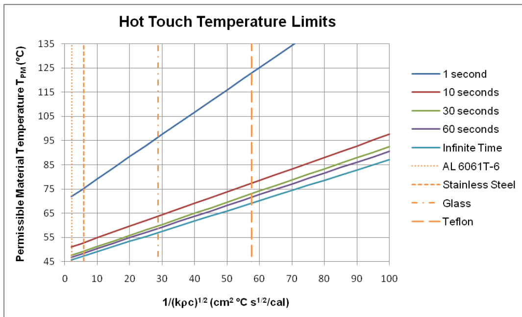
Figure Q.2.2V-1: Hot Temperature Limits
