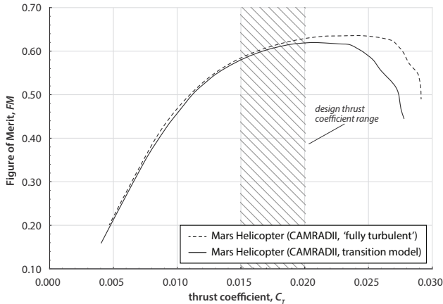
Figure 24. Figure of Merit versus thrust for \rho = 0.017 \text{ kg/m}^3 and T = -50^\circ\text{C} (Mars Condition 2)
