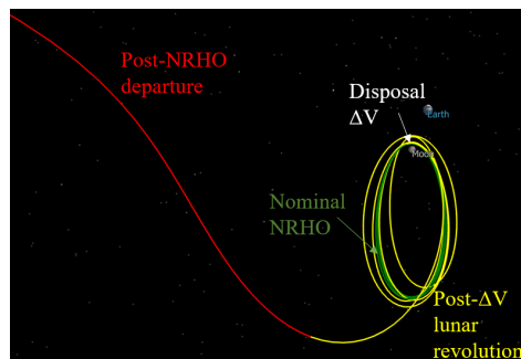
Figure 1: Sample NRHO disposal trajectory as viewed in the Earth-Moon rotating frame.
