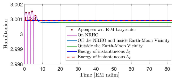
Figure 10: Energy history of the direct escape trajectory in the S - B_1 frame
