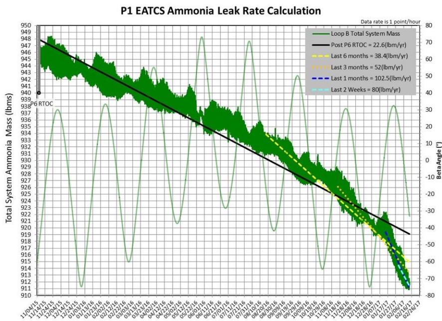
Figure 10: Leak trend data of the known ammonia leak through January 2017.
