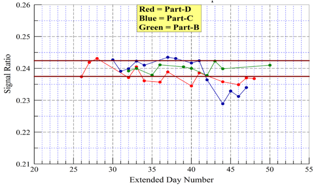
Figure 15. AT water vapor calibration ratio for the Part-B-D deployments. The X-axis is a simple means of plotting data from multiple deployments on one plot.
