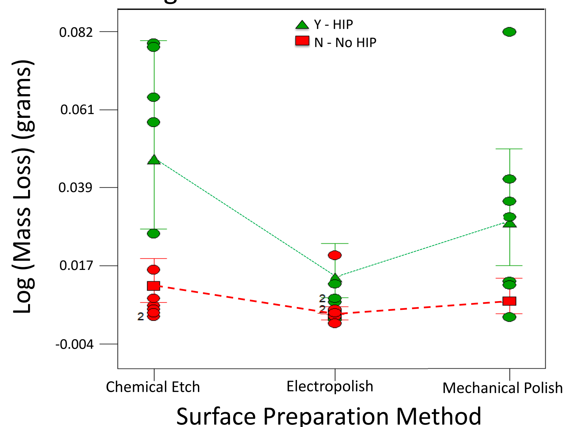
Figure 1. Results of a 30 test supersonic PI surface preparation experiment using only SLM IN718 comparing surface treatment and HIP at a static pressure of 1300 psia, and an average temperature of 562° F, and a single 200 μm aluminum ball.
