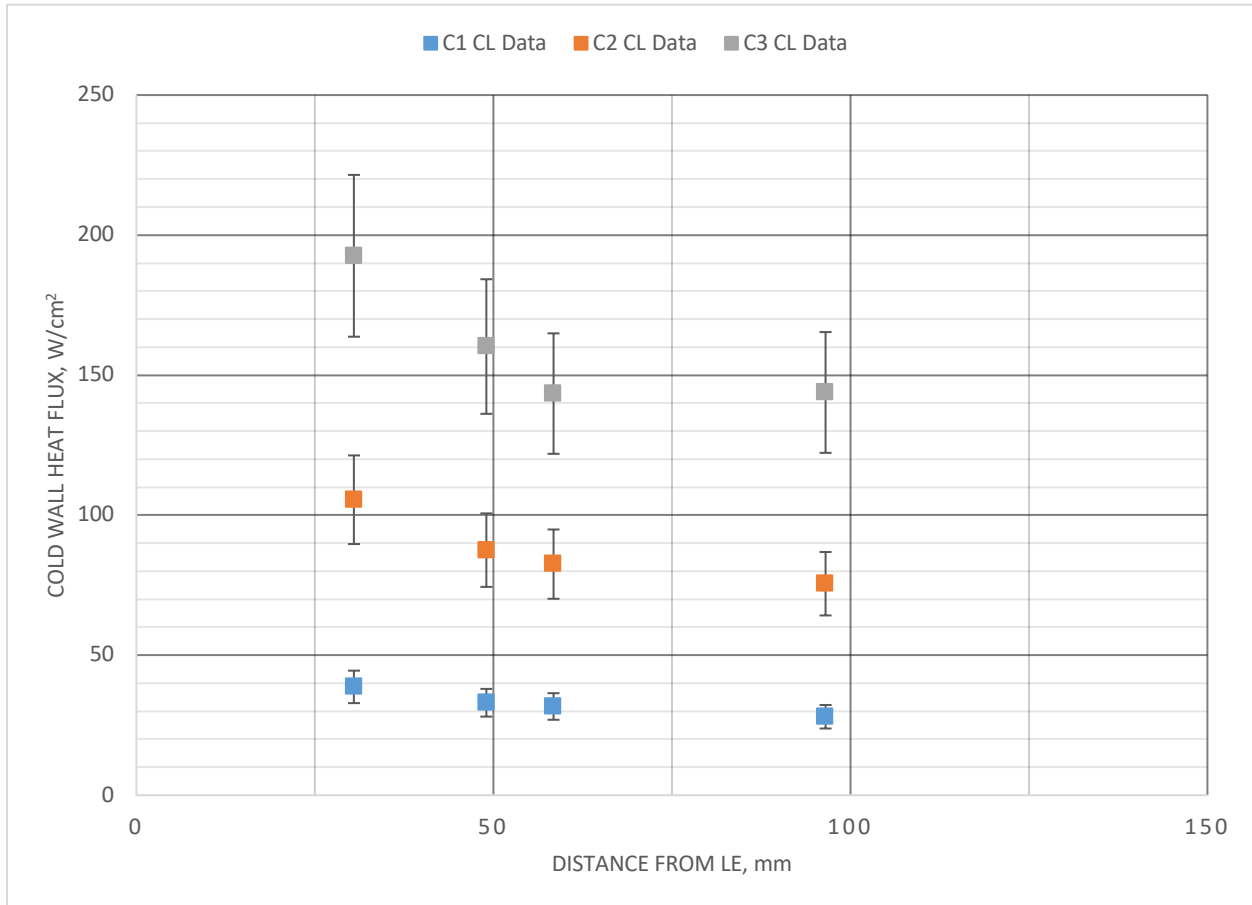
Figure 11. Convective calibration along centerline. Graphed results from Table 4. Error bars are ±15%.
