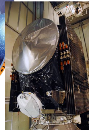
Dawn spacecraft
