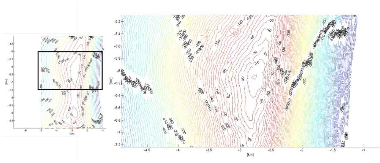
Figure 4.32. Zoom in of area around Point 1
