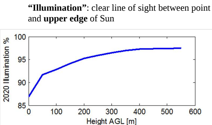
Figure 4.30. Point 1, best 65 m reflector location, and 2020 % of illumination for selected point as increases with height at that point.
