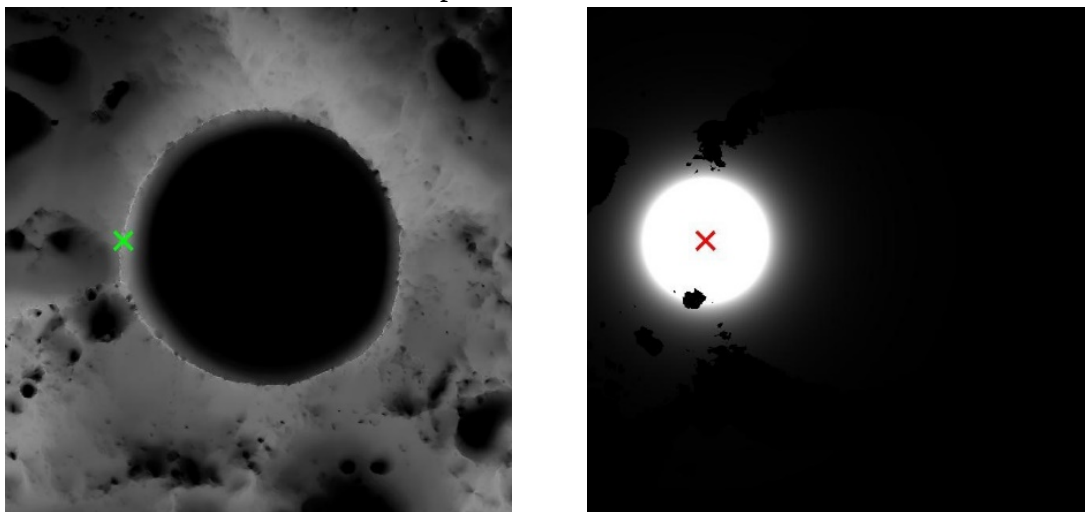
Figure 4.18. Location (left) and corresponding oasis map (right) for single reflector placed 775 meters above ground level at 89.7841°S 156.2906°W.
