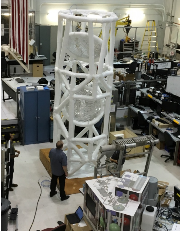
Figure 3.21. (Right) Tectoniks inflatable TransFormer scaled prototype in its fully inflated configuration in the NASA KSC Swamp Works Laboratory. The lander in the lower right of the photo is an ISRU lander mock-up containing a hopper lift system, soil dryer, water clean-up module, and umbilical to transfer the water to rovers.
