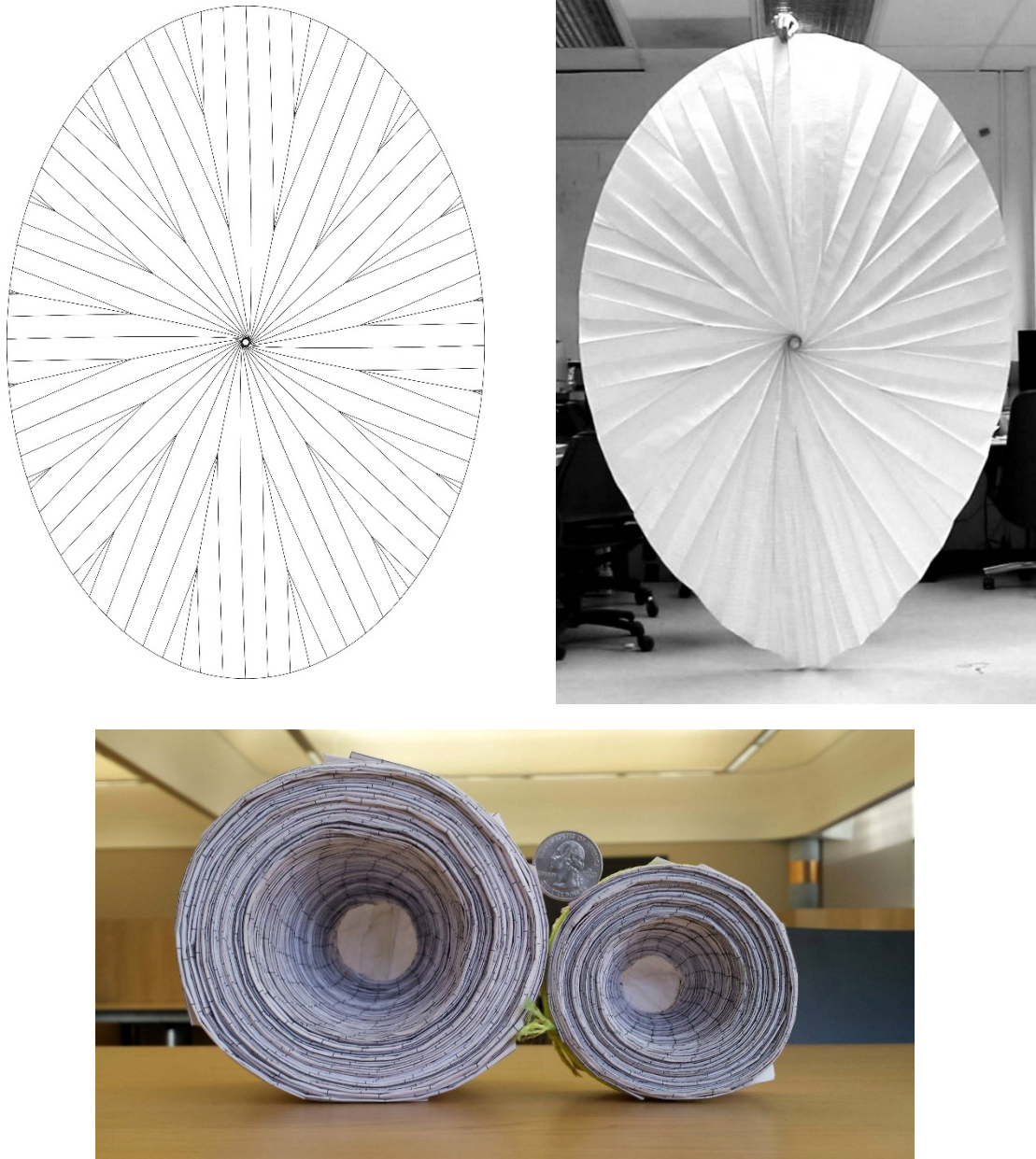
Figure 3.13. Crease pattern that stows to 1/40th of its longest dimension. A 1/16 scale model of an elliptic reflector was also folded demonstrate how it stows and deploys. Partially deployed origami ellipse (top) and same ellipse stowed (bottom). Ellipse is 106 cm × 183 cm.
