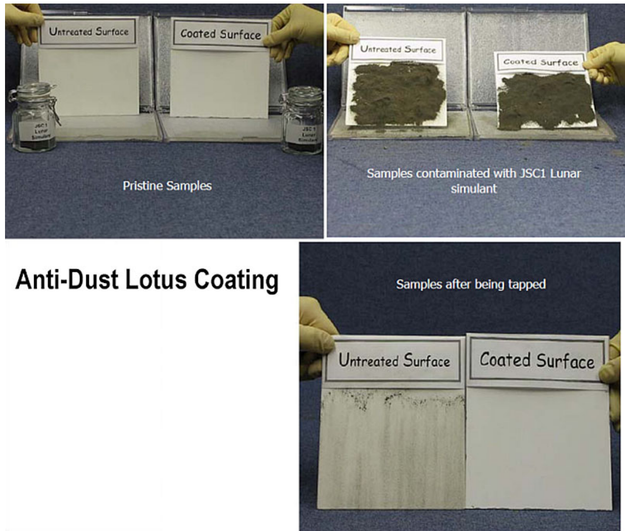
Figure 3.25. Anti-dust coating comparing untreated and treated surfaces of a pristine sample(top left), samples contaminated with JSC1 lunar simulant (top right) and samples after being tapped (bottom right). This demonstrates how anti-dust lotus coating can help protect surfaces.
