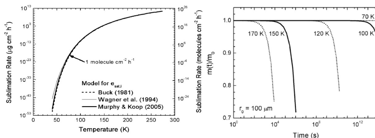
Figure 2.10. Ice sublimation rate vs. temperature, from http://www.nwra.com/resumes/andreas/publications/Icarus_Moon.pdf . Mass of ice as function of time (Andreas 2007).
