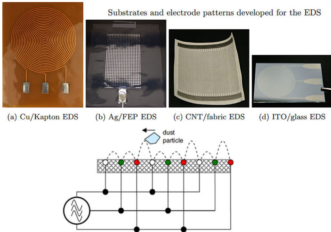
Figure 3.24. Various substrates and electrode patterns for developed EDS (top) and schematic depicting dust particle motion on a three phase EDS (bottom).
