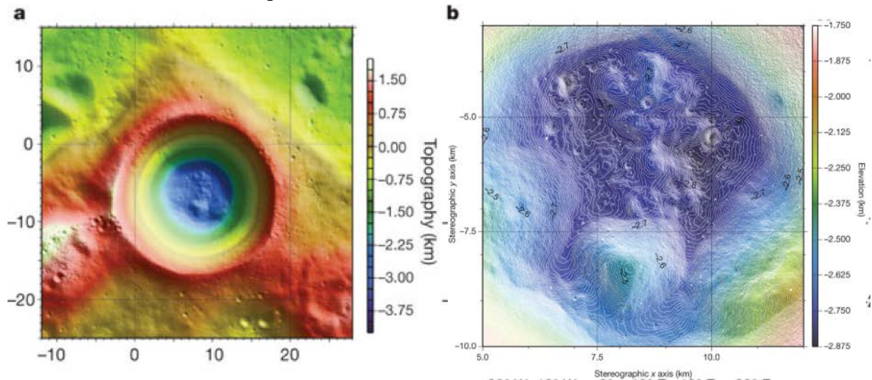
Figure 1.3. (a) Topography of SC sampled at 10-m spatial resolution; Elevations are contoured at 5-m intervals with colors indicating elevation with respect to 1,737.4 km. (b) a more detailed view of the topography of Shackleton's floor, which highlights the irregularly distributed deposits and numerous small craters (Bryant 2010)
