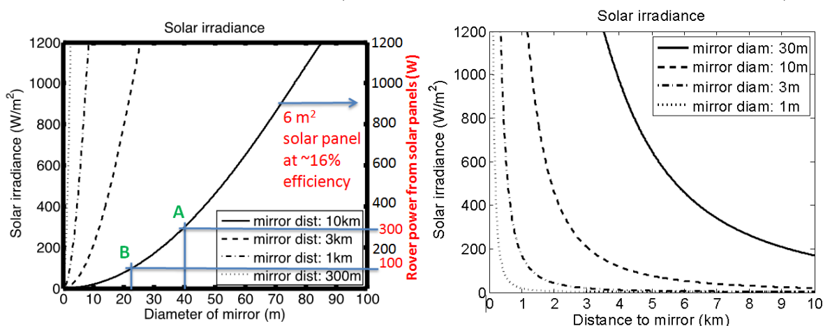
Figure 3.6. Solar irradiance vs. distance to mirror (left). Solar irradiance vs diameter of mirror (right).
