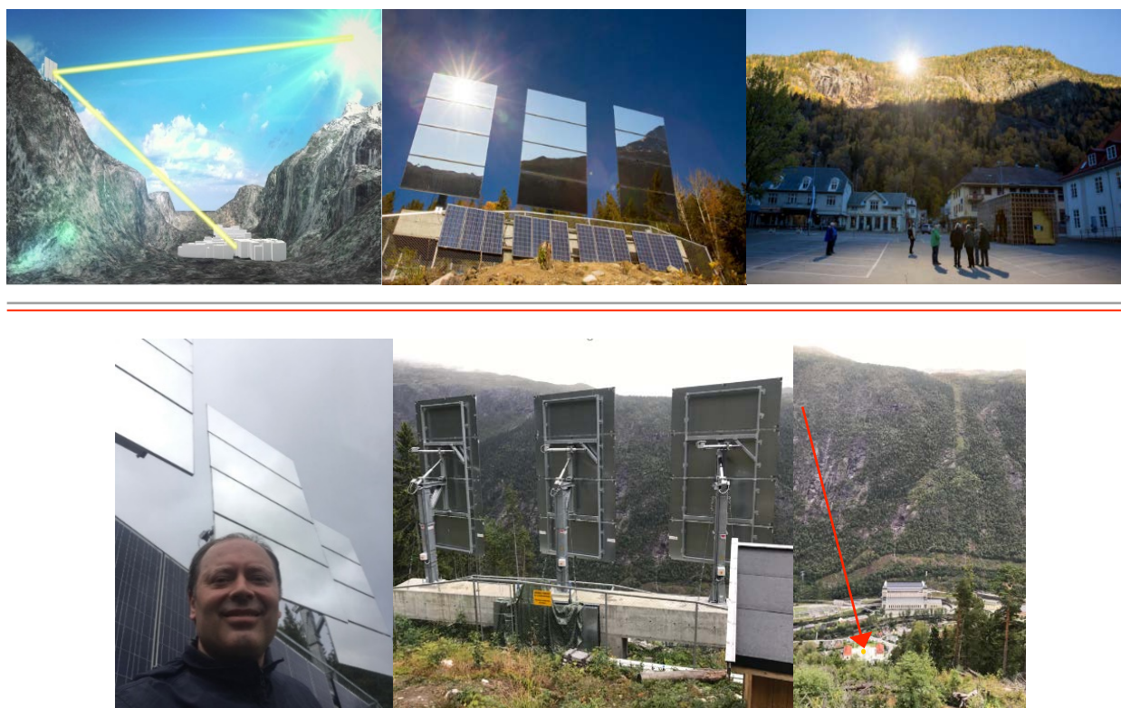
Figure 1.7. Top row: Heliostats illuminating towns in deep valley at Rjukan, Norway. Bottom row: NIAC Fellow Stoica, after a hike at Rjukan, next to the mirrors; back of mirrors and location where sunrays are redirected in town plaza, at ~700 m away from the mirrors.
