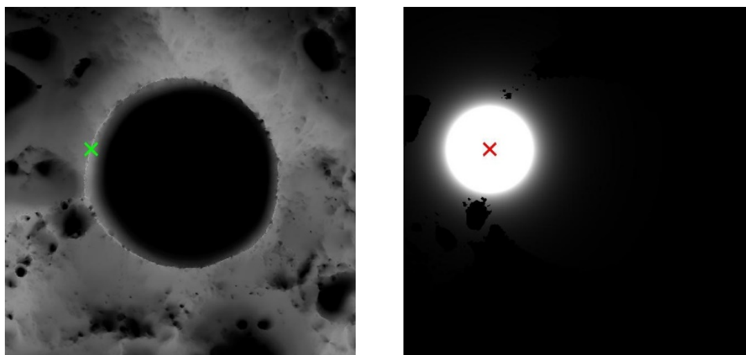
Figure 4.19. Location (left) and corresponding oasis map (right) for single reflector placed 775 meters above ground level at 89.8522°S 151.2430°W.
