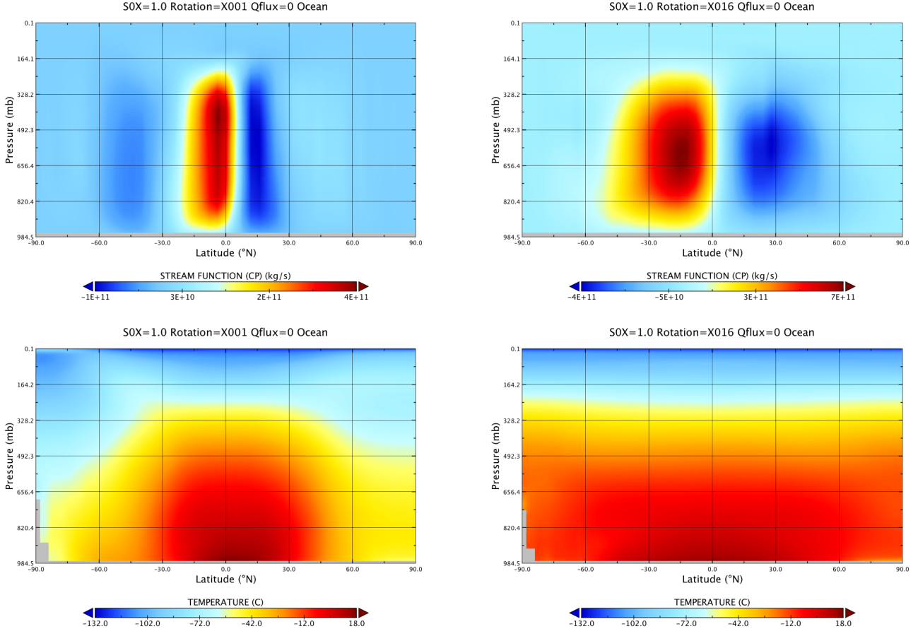
Figure 9. Top panels: model stream function diagnostic showing increase in Hadley Cell size and decrease in number from Rotations X001 to X016. Bottom panels: The increase in the size of the Hadley cell transports more heat to higher latitudes. This effect is seen in the latitudinal temperature differences between X001 and X016. This is also seen in the decrease in the amount of high latitude Sea Ice (Ocean Ice Fraction) in Figure 5 in the lower left panel between the X001 and X016 simulations for the same insolation (in this case S0X=1.0 ).
