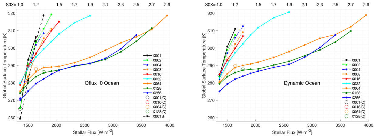
Figure 1. Global mean surface temperature for ROCKE-3D as a function of insolation at different rotation periods for thermodynamic ocean simulations (a, left) and dynamic fully coupled ocean (b, right). Solid curves and dots show results from the baseline model at 10% increments above the modern Earth insolation value and 20% increments above S0X=1.5. Open circles are for sensitivity tests with no vertical transport of convective condensate. The dashed curve is for an alternate model version with the same physics but using different settings of free parameters to adjust the model to global radiative balance.
