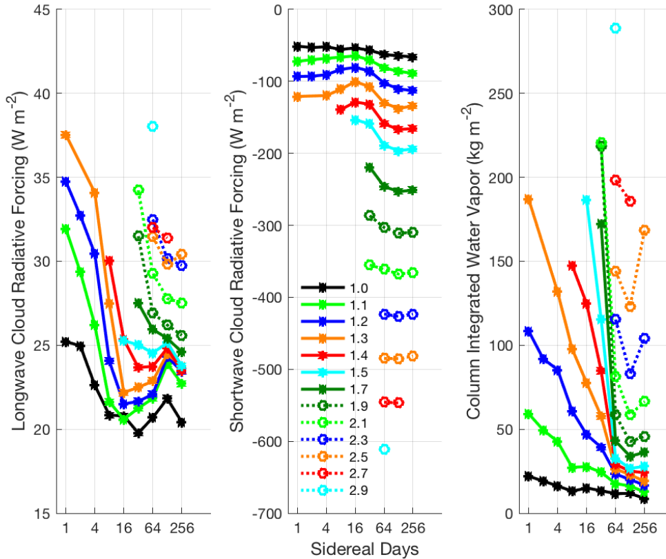
Figure 11. (Left) Longwave Cloud Radiative Forcing (CRF), (center) Shortwave CRF, and (right) column integrated water vapor as a function of rotation period for the dynamic ocean simulations for different S0X values.
