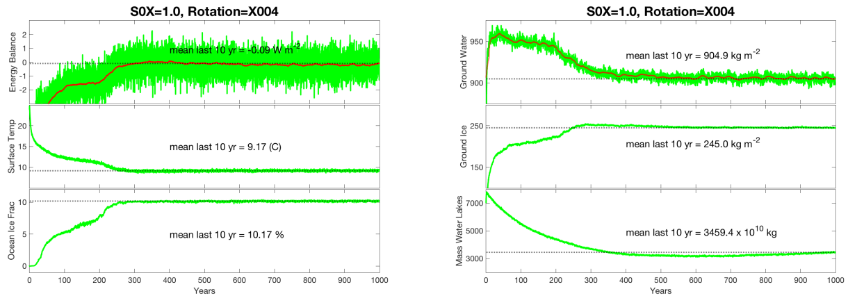
Figure 13. S0X=1.0 with sidereal day length set to 4 days (X004). Left (a) from top to bottom y-axes are net radiative balance in \text{W m}^{-2} , surface temperature in Celsius, and ocean ice fraction in total percentage of ocean area. Right (b) from top to bottom y-axes are total global ground water amounts in \text{kg m}^{-2} , total ground ice in \text{kg m}^{-2} and the total mass of water in lakes and rivers in kg.
