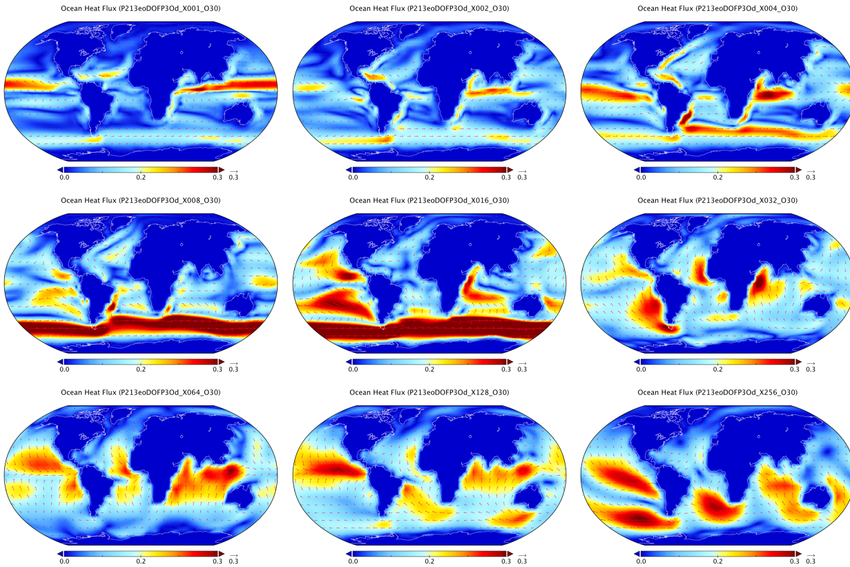
Figure 7. Meridional plus zonal ocean heat flux ( \sqrt{\text{Meridional}^2 + \text{Zonal}^2} ) in units of 10^{15} Watts. These are 9 runs at fixed insolation of S_0X=1.2 from sidereal length of day = X001 (1 x Earth), all the way up to X256 sidereal days in length.
