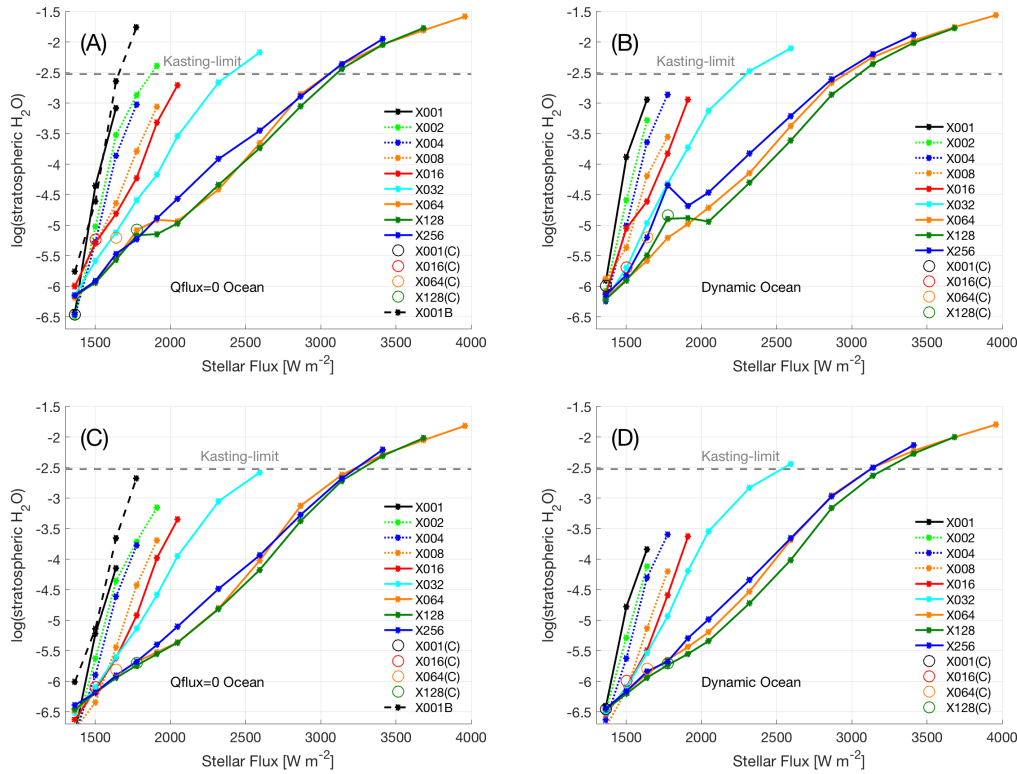
Figure 12. Stratospheric water vapor content for Q-flux=0 ocean runs (A/C, left) and Dynamic Ocean runs (B/D, right). Y-axis is the \log_{10} of the specific humidity at 0.1 hPa for \text{H}_2\text{O}/\text{Air} (kg/kg). A & B are values for the grid cell with the largest value at the highest layer in each simulation whereas C & D are the mean at the highest layer.
