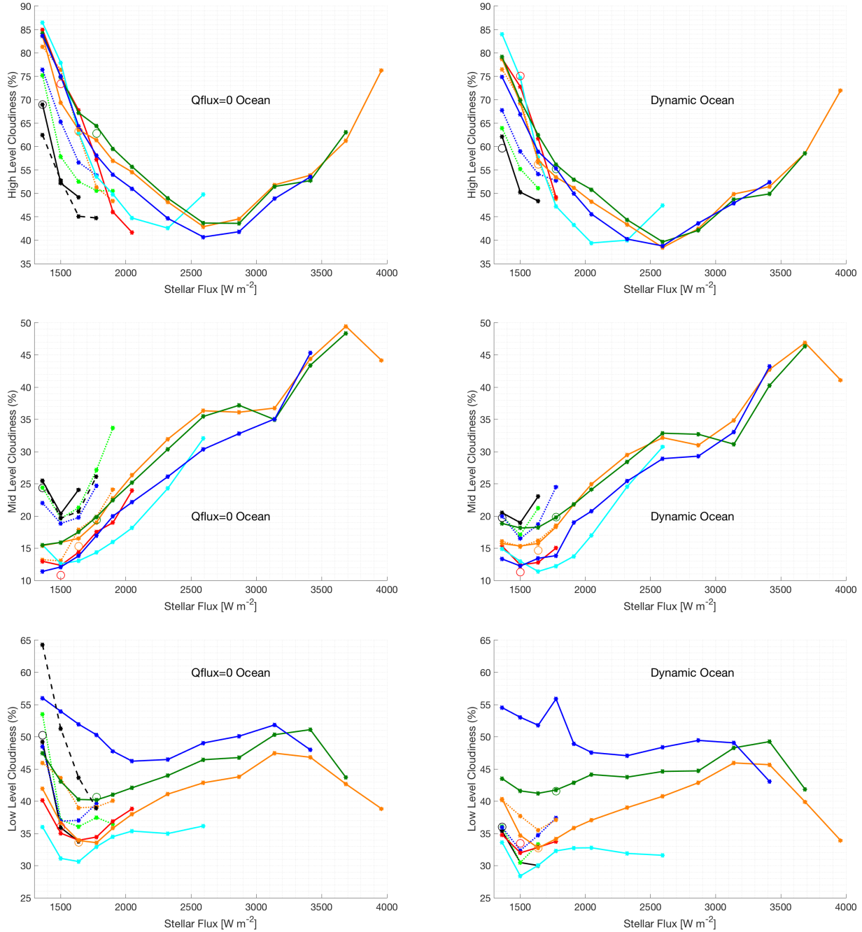
Figure 6. Cloud Fractions at highest level (top), middle level (middle) and bottom level (bottom) for Q-flux=0 (left) and Dynamic Ocean runs (right). Note: the y-axes have different values from top to bottom.
