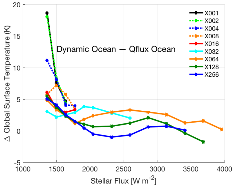
Figure 2. Global mean surface temperature differences when subtracting the Q-flux=0 mean temperature from that of the dynamic ocean.
