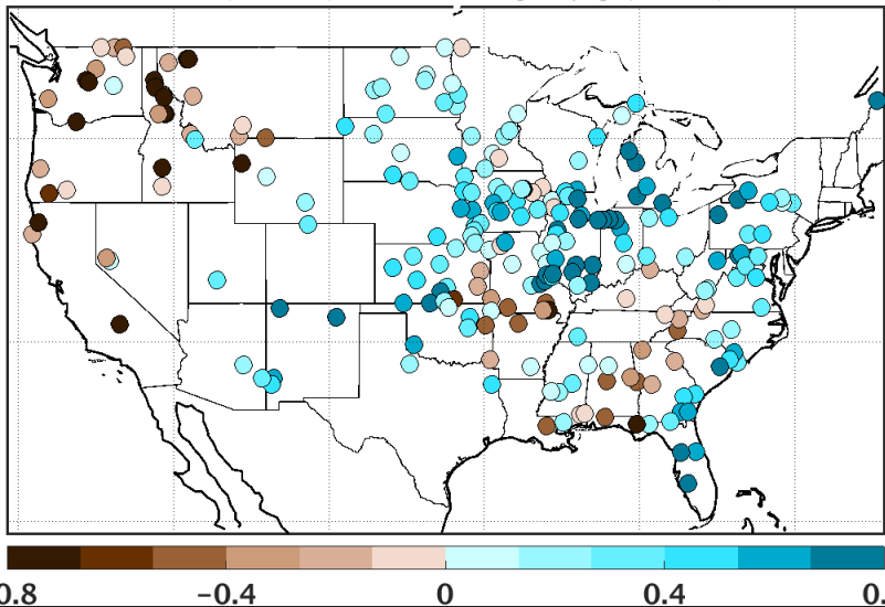
LDAS Runoff v. USGS Streamflow Apr - Sep (2015 - 2017) \Delta absBias (OL4001-OL4002) mean = -0.12[mm/d] (N=239)
