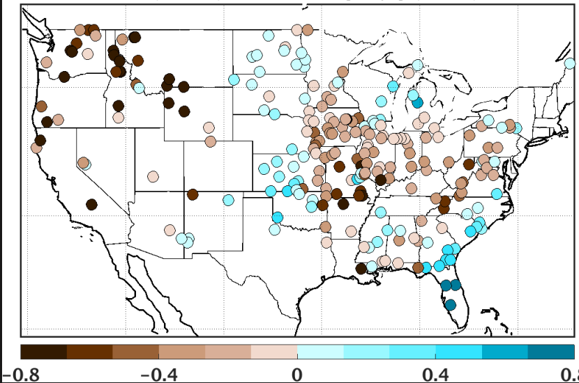
LDAS Runoff v. USGS Streamflow Apr - Sep (2015 - 2017) \Delta absBias (Vv4030-OL4001) mean = 0.006[mm/d] (N=239)
