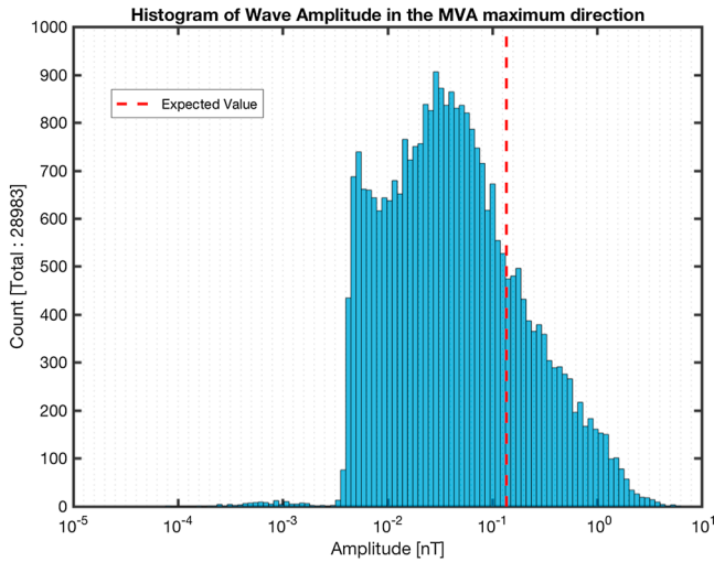
Figure 12. Histogram of the amplitude in the maximum MVA coordinate of the MVA subintervals where \omega_{rf} > \omega_{LH} . The expected value obtained by the probability density function fitted to the data is shown. The fitted probability density function is not shown because it was not estimated for the logarithm of the data. MVA = minimum variance analysis.
