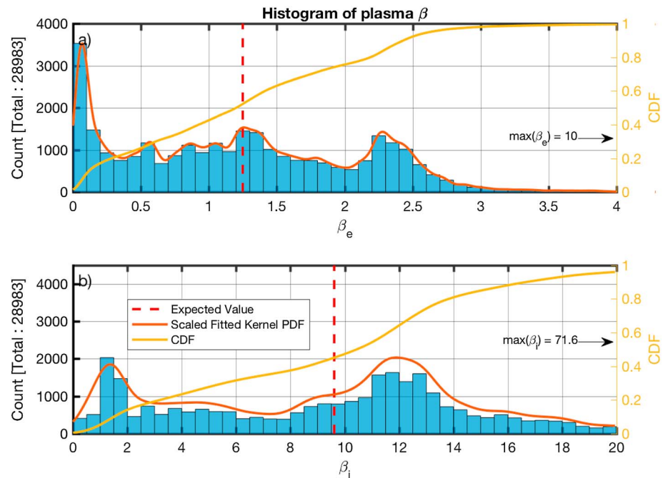
Figure 14. Histograms of the calculated plasma beta for the electrons (panel a) and ions (panel b) for the minimum variance analysis subintervals for which \omega_{rf} > \omega_{LH} . The estimated scaled fitted PDF and the CDF are also shown in red and yellow, respectively. The calculated average is shown by the dashed vertical red line. CDF = cumulative density function; PDF = probability density function.
