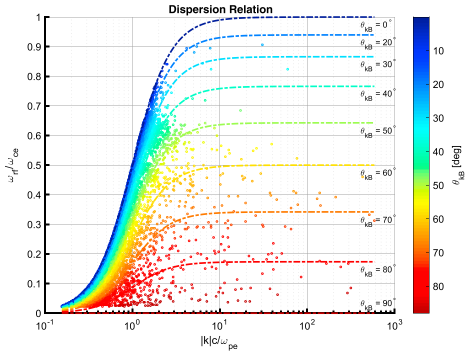
Figure 9. Dispersion relation for the 30,636 minimum variance analysis intervals where \omega_{rf} > \omega_{LH} . The circles are the points of the individual minimum variance analysis subintervals. The dashed lines show the calculated dispersion for a given \theta_{kB} angle.
