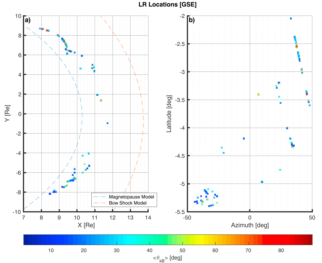
Figure 5. Locations of observed LR emissions by the Magnetospheric Multiscale 3 on 18 different dates from 16 October 2015 to 13 January 2016. The 1,738 locations shown are the ones where the minimum variance analysis eigenvalues were considered good. The x - y positions of the spacecraft at the time of observation are shown in panel a, along with a model magnetopause (blue dashed line) and model bow shock (red dashed line). In panel b the latitude versus the azimuth angle of the position of the observed LR is shown. The points in both panels follow the same color coding for the angle between the background magnetic field and the average propagation direction of each LR interval observed ( \langle \theta_{kB_0} \rangle ). LR = lion roar.
