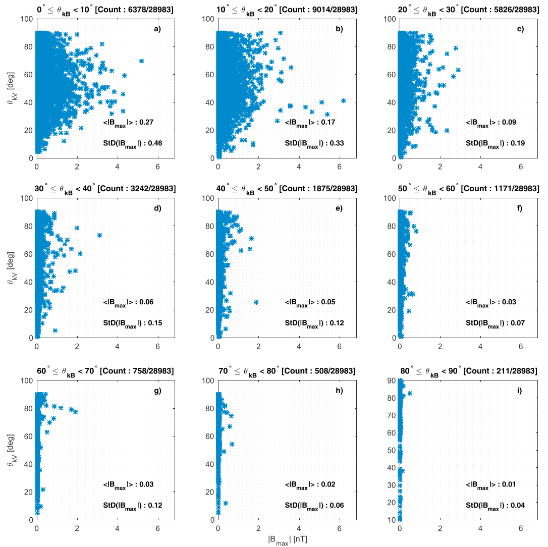
Figure 13. (a–i) Plots of \theta_{kV} against the amplitude in the maximum minimum variance analysis coordinate of the minimum variance analysis subintervals where \omega_{rf} > \omega_{LH} . In each panel emissions with the \theta_{kB} range are shown. The mean ( \langle |B_{max}| \rangle ) and the standard deviation ( StD(|B_{max}|) ) for each interval of \theta_{kB} are also shown.
