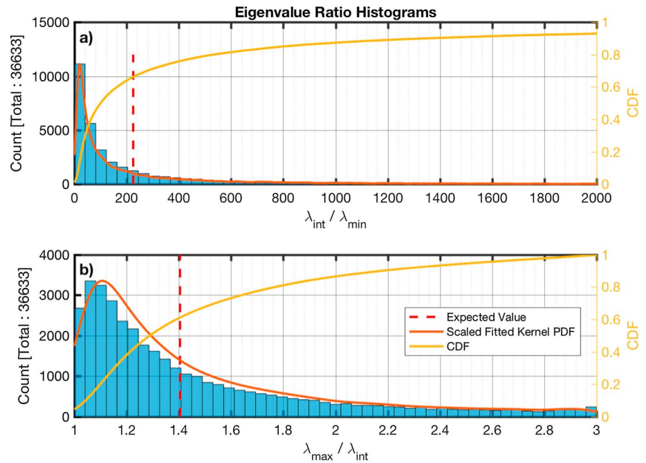
Figure 8. Histograms of the eigenvalue ratios of the intermediate to minimum (panel a) and the maximum to intermediate (panel b) minimum variance analysis components. The estimated scaled fitted PDF and the CDF are also shown in red and yellow, respectively. The calculated average is shown by the dashed vertical red line. CDF = cumulative density function; PDF = probability density function.
