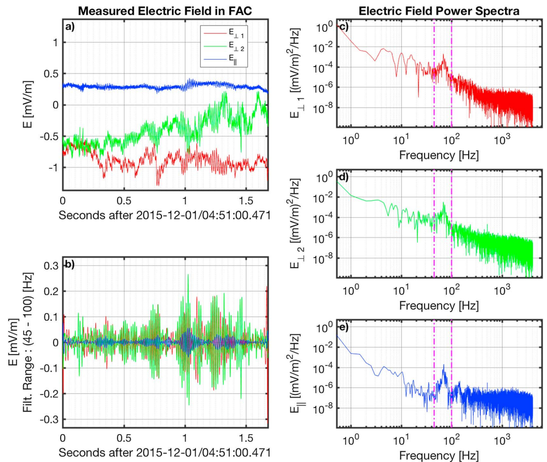
Figure 2. Electric field measurements of an example lion roar. The measured electric field in FAC is shown in panel a. The band-pass ([45–100] Hz) filtered signal of the emission is shown in panel b. Panels c–e show the power spectrum for each of the three electric field components E_{\perp 1} , E_{\perp 2} , and E_{\parallel} , respectively. The vertical magenta lines in panels c–e denote the frequency band of the emission as identified by the power spectra. FAC = field-aligned coordinates.
