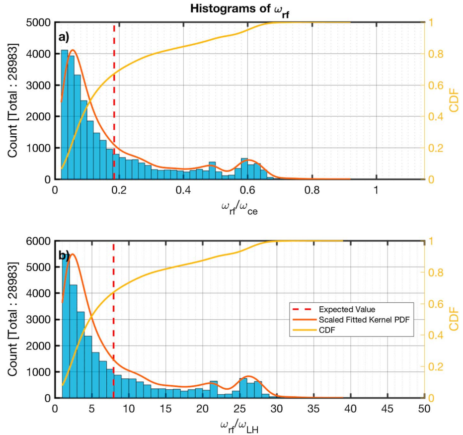
Figure 10. Histograms of the ratios of the rest frame frequency peak ( \omega_{rf} ) identified to the electron cyclotron (panel a) and the lower hybrid frequency (panel b), for each minimum variance analysis subinterval. The estimated scaled fitted PDF and the CDF are also shown in red and yellow, respectively. The calculated average is shown by the dashed vertical line. CDF = cumulative density function; PDF = probability density function.
