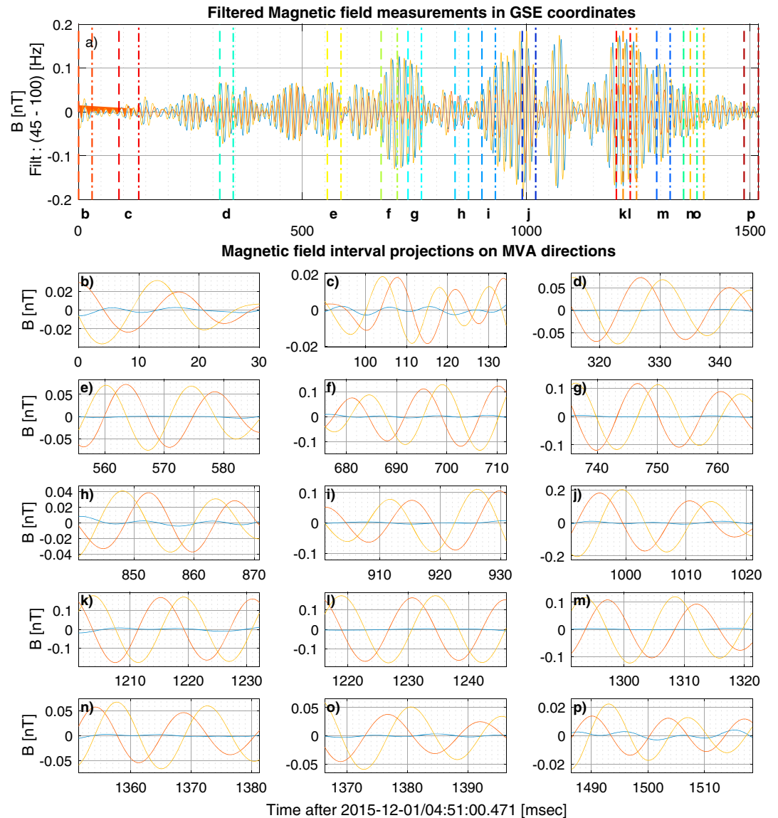
Figure 3. Filtered magnetic field measurements in GSE coordinates (a) for the example emission on 1 December 2015. The magnetic field projections on the MVA directions for each interval (b–p). The minimum, intermediate, and maximum directions are shown in blue, red, and orange, respectively. MVA = minimum variance analysis.
