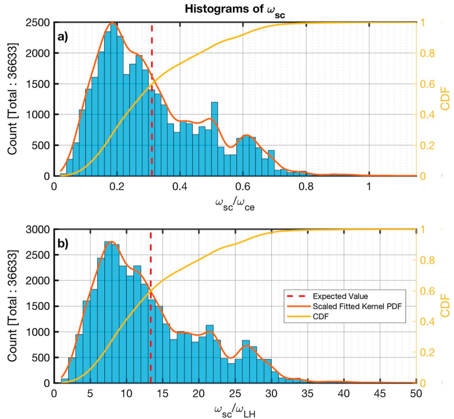
Figure 6. Histograms of the ratios of the spacecraft frame frequency peak ( \omega_{sc} ) identified to the electron cyclotron (panel a) and the lower hybrid frequency (panel b), for each minimum variance analysis subinterval. The estimated scaled fitted PDF and the CDF are also shown in red and yellow, respectively. The calculated average is shown by the dashed vertical red line. CDF = cumulative density function; PDF = probability density function.
