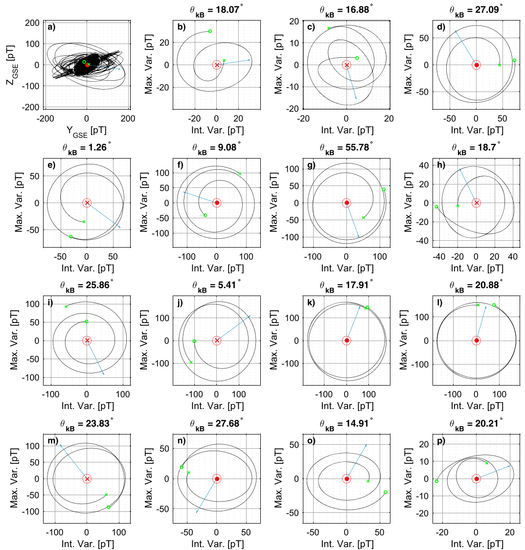
Figure 4. (a–p) Hodograms of the magnetic field maximum and intermediate components for the individual minimum variance analysis intervals of the lion roar example. The blue arrow shows the direction of the background magnetic field ( \mathbf{B}_0 ) projected onto the plane of the maximum and intermediate minimum variance analysis direction. The direction of the minimum variance is shown in the origin of the plots with a dot/cross mark.
