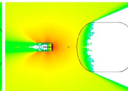
Example of Radiation Flux with External Shield
