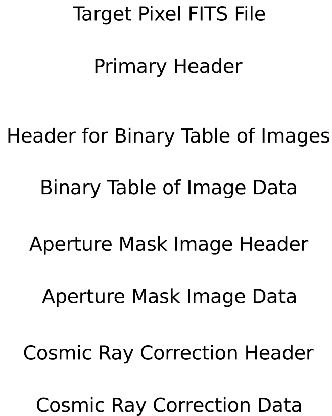
Figure 2: Target pixel FITS file composition
