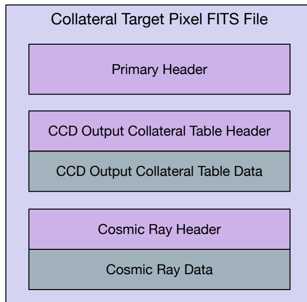
Figure 4: Collateral target pixel FITS file composition
