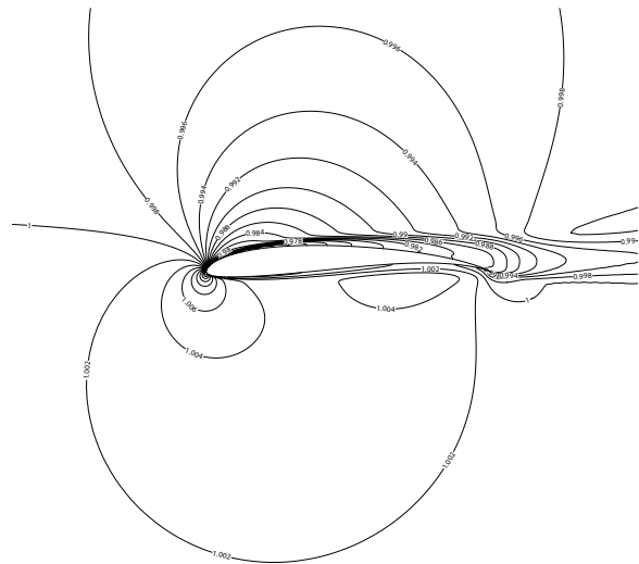
Figure F3. Non-dimensional density contours, \rho/\rho_\infty for Station 3, Mars Condition 2 ( r/R = 0.30 , \alpha = 4.82 , M = 0.22 )
