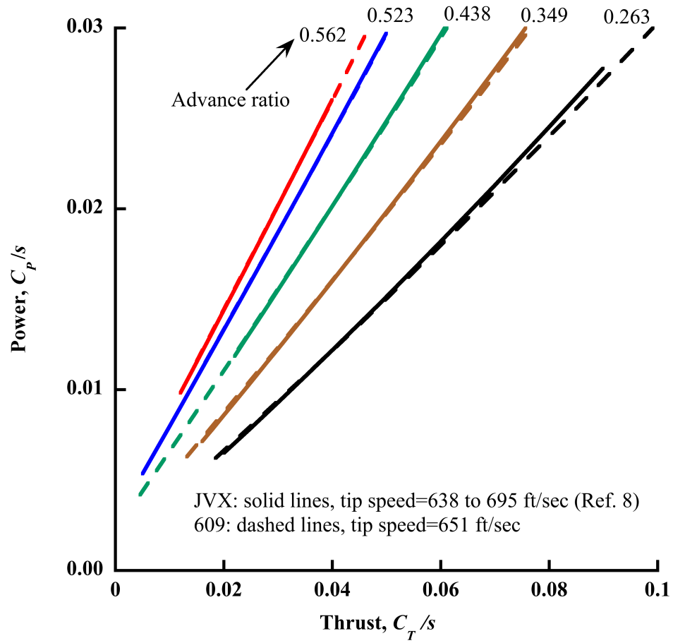
Fig. 4b. Reality check, JVX and 609 predicted forward flight power comparison.
