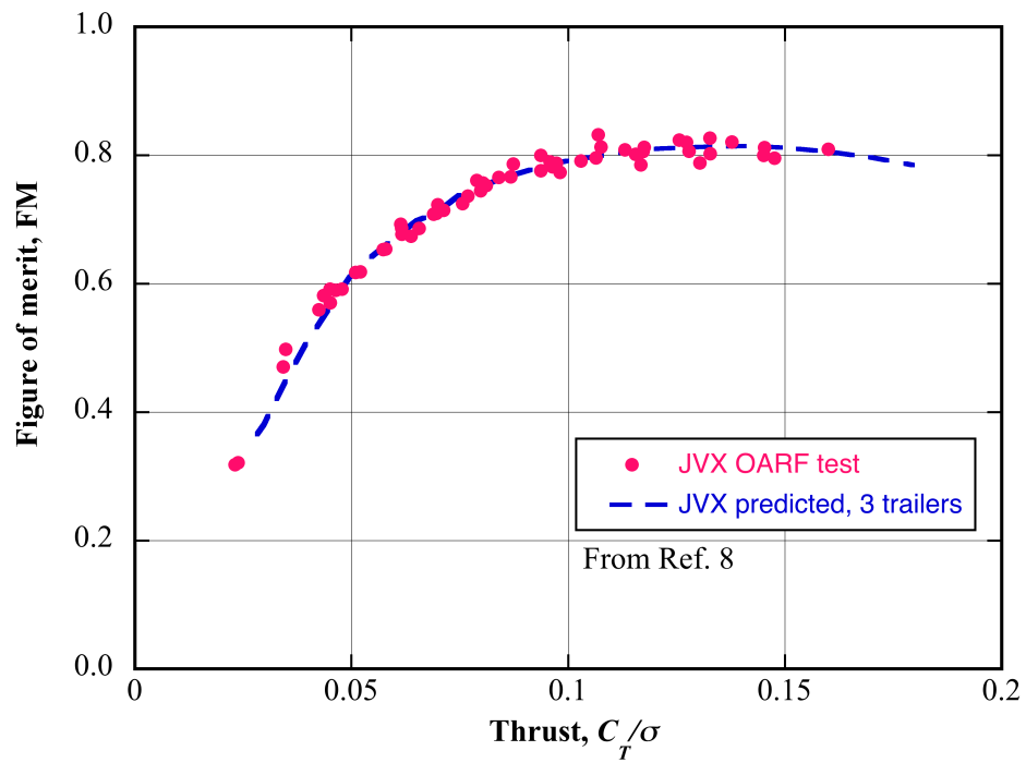
Fig. 3a. JVX figure of merit correlation (Ref 8).
