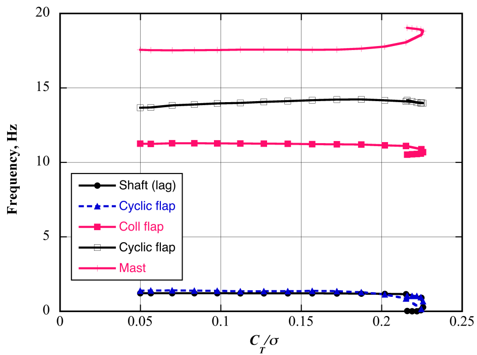
Fig. 8b. Predicted TTR/609 hover frequencies vs. thrust, 0-deg yaw, 569 rpm.
