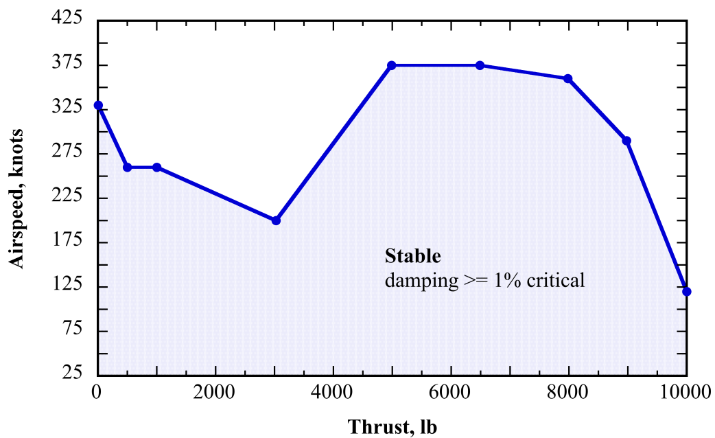
Fig. 11a. Predicted TTR/609 helicopter mode (axial and edgewise flow) 1% damping stability envelope, 90-deg yaw, 569 rpm (rap test modal data).
