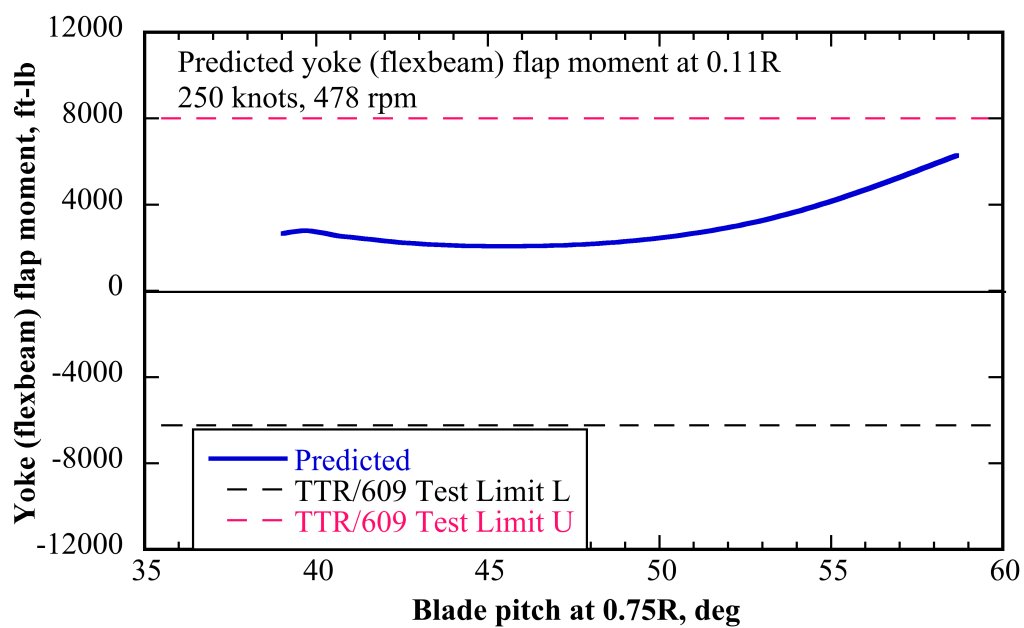
Fig. 6e. Predicted 609 cruise (axial flow) yoke flap moment vs. collective, 0-deg yaw, 250 knots, 478 rpm.
