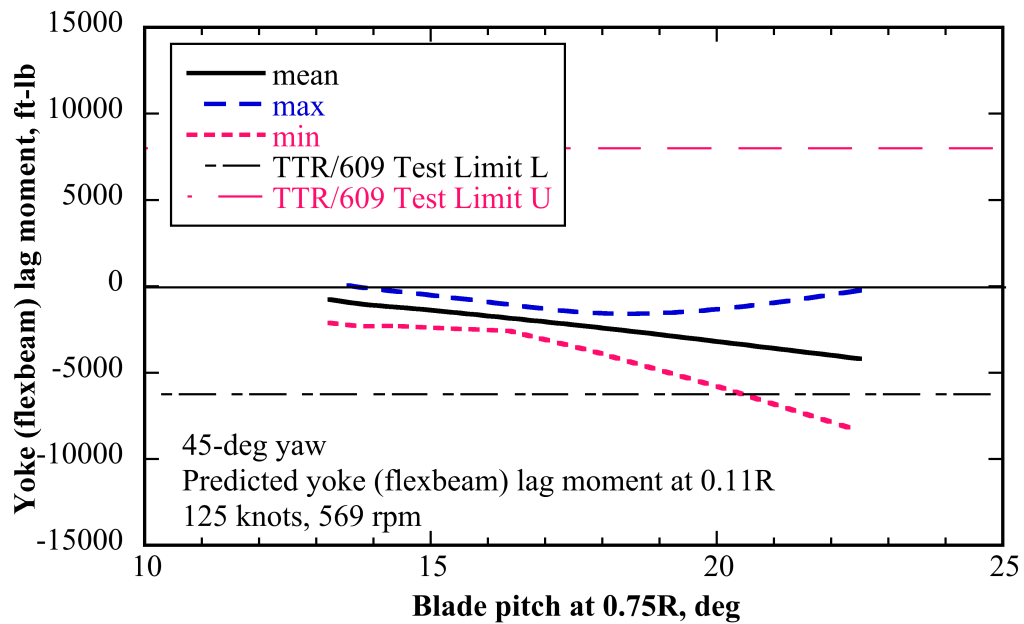
Fig. 7f. Predicted 609 conversion (axial and edgewise flow) yoke lag moment vs. collective, 45-deg yaw, 125 knots, 569 rpm.
