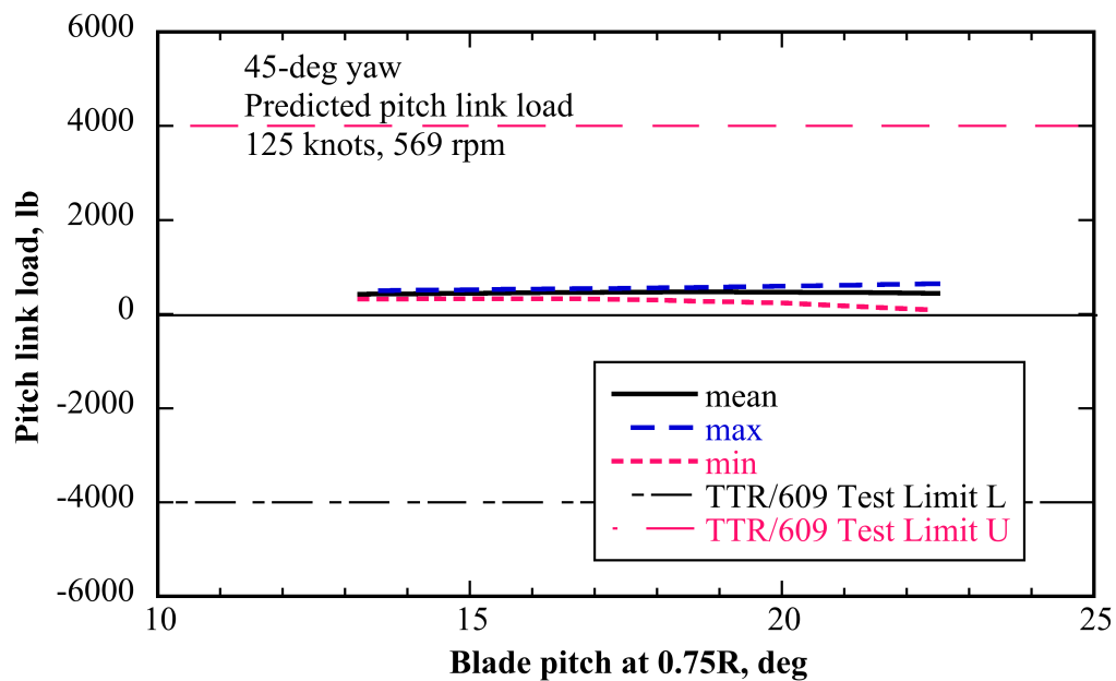
Fig. 7c. Predicted 609 conversion (axial and edgewise flow) pitch link load vs. collective, 45-deg yaw, 125 knots, 569 rpm.
