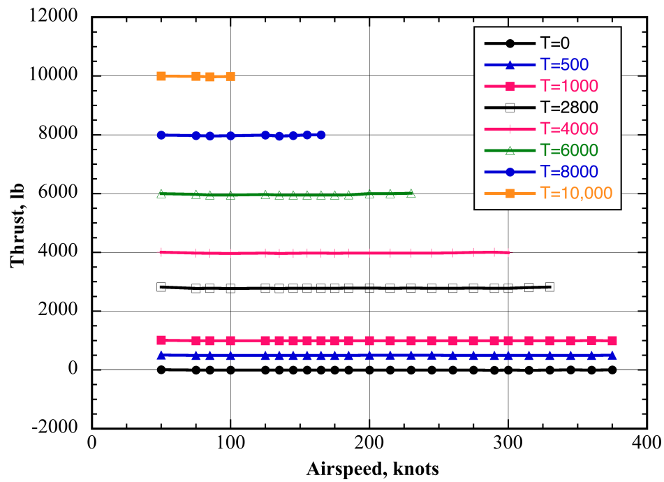
Fig. 10a. Predicted TTR/609 conversion (axial and edgewise flow) trim thrust vs. airspeed, 45-deg yaw, 569 rpm.
