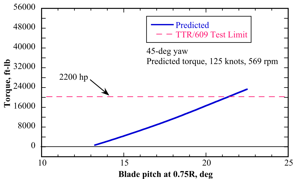
Fig. 7b. Predicted 609 conversion (axial and edgewise flow) torque vs. collective, 45-deg yaw, 125 knots, 569 rpm.
