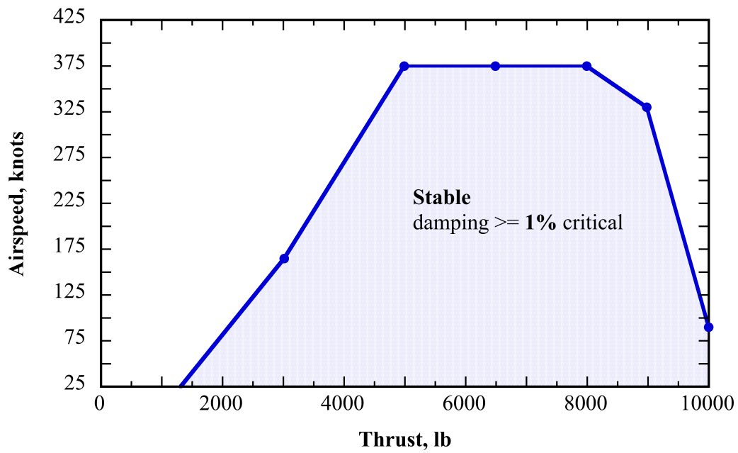
Fig. 11b. Predicted TTR/609 helicopter mode (axial and edgewise flow) 1% damping stability envelope, 90-deg yaw, 569 rpm (shake test modal data).
