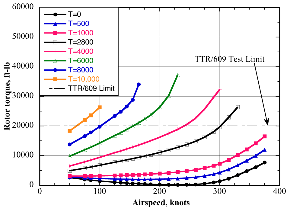
Fig. 10b. Predicted TTR/609 conversion (axial and edgewise flow) torque vs. airspeed, 45-deg yaw, 569 rpm.
