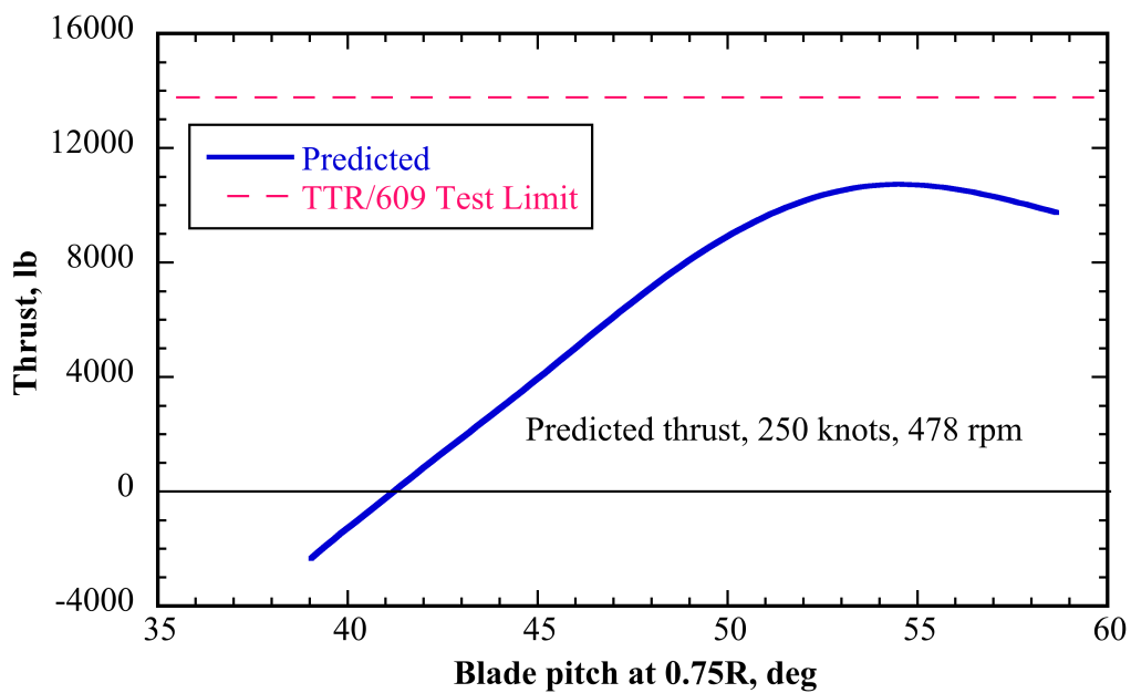
Fig. 6a. Predicted 609 cruise (axial flow) thrust vs. collective, 0-deg yaw, 250 knots, 478 rpm.
