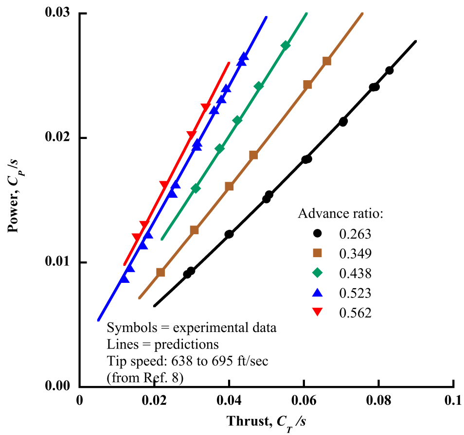
Fig. 4a. J VX forward flight power correlation (Ref. 8).
