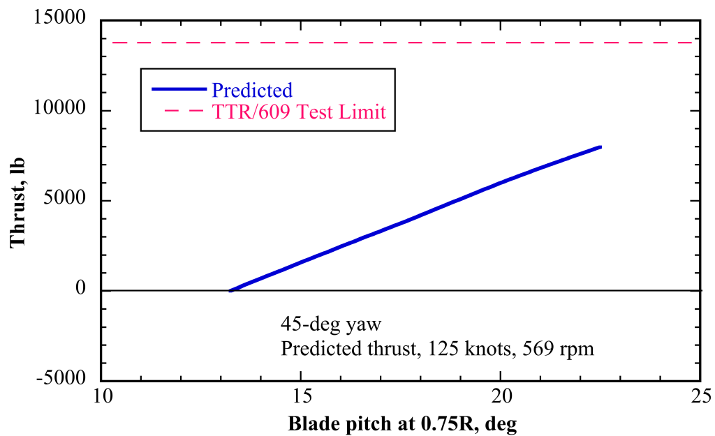
Fig. 7a. Predicted 609 conversion (axial and edgewise flow) thrust vs. collective, 45-deg yaw, 125 knots, 569 rpm.
