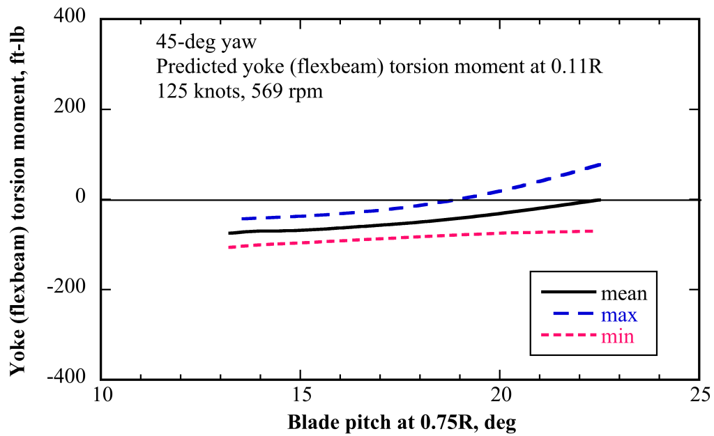
Fig. 7d. Predicted 609 conversion (axial and edgewise flow) yoke torsion moment vs. collective, 45-deg yaw, 125 knots, 569 rpm.
