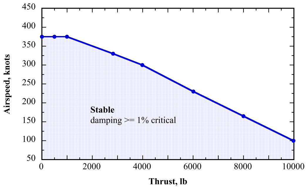
Fig. 10e. Predicted TTR/609 conversion (axial and edgewise flow) 1% damping stability envelope, 45-deg yaw, 569 rpm (rap test modal data).
