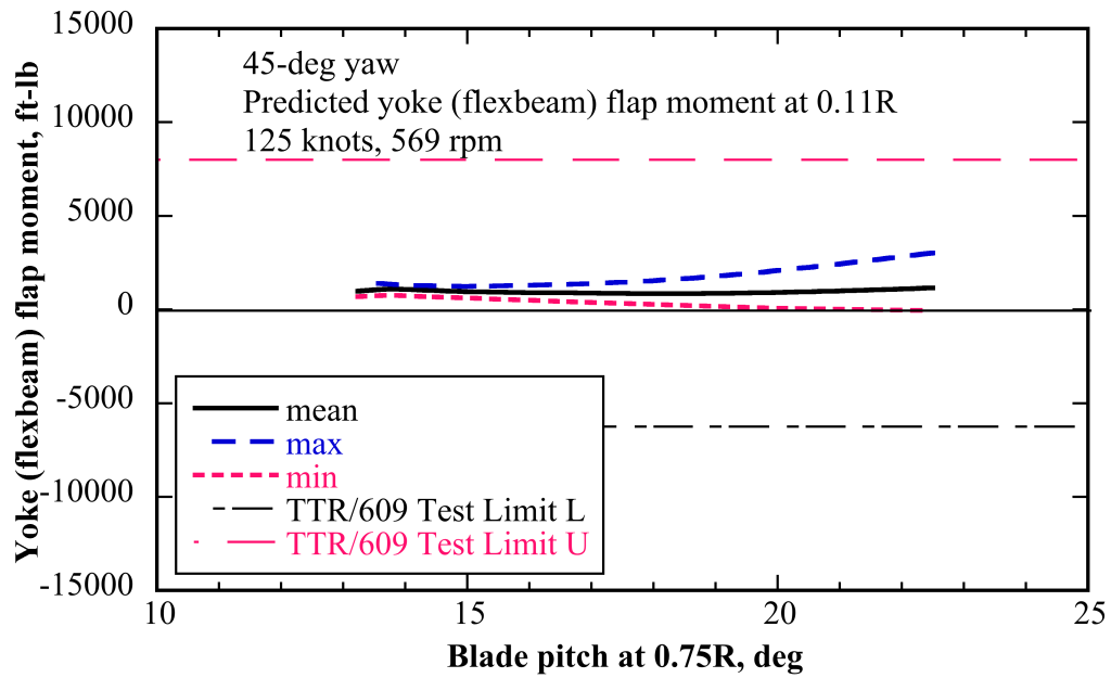
Fig. 7e. Predicted 609 conversion (axial and edgewise flow) yoke flap moment vs. collective, 45-deg yaw, 125 knots, 569 rpm.
