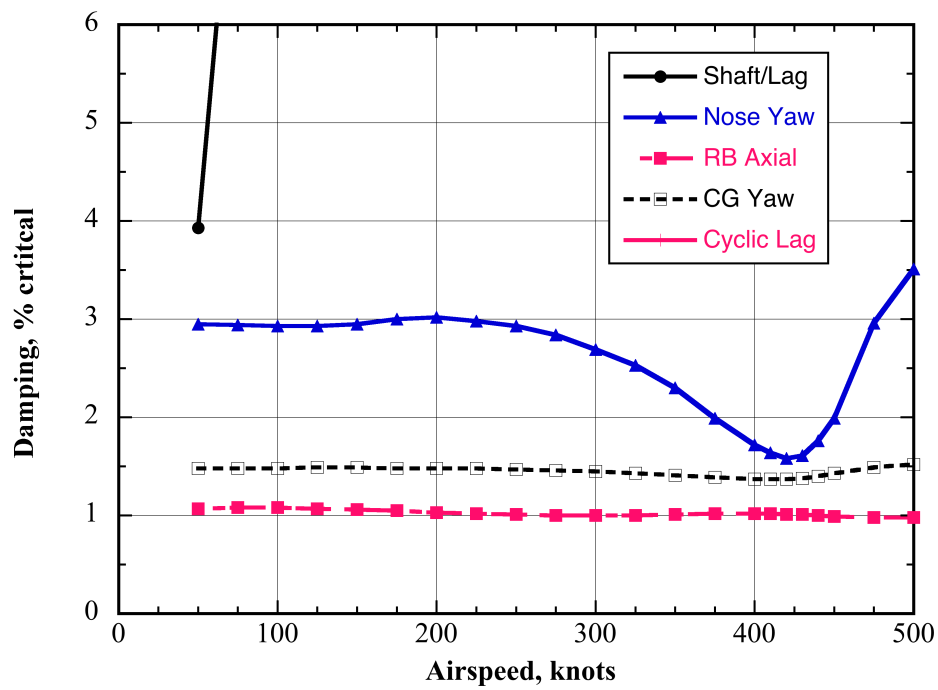
Fig. 9a. Predicted TTR/609 cruise (axial flow) damping vs. airspeed, 0-deg yaw, 0 power, 478 rpm.
