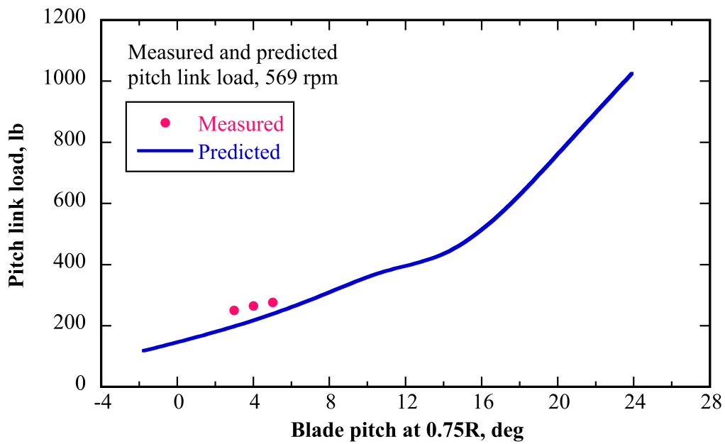
Fig. 5c. 609 hover pitch link load vs. collective, 569 rpm.
