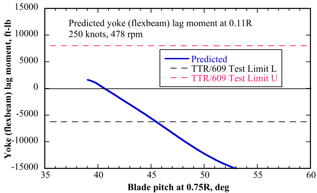
Fig. 6f. Predicted 609 cruise (axial flow) yoke lag moment vs. collective, 0-deg yaw, 250 knots, 478 rpm.
