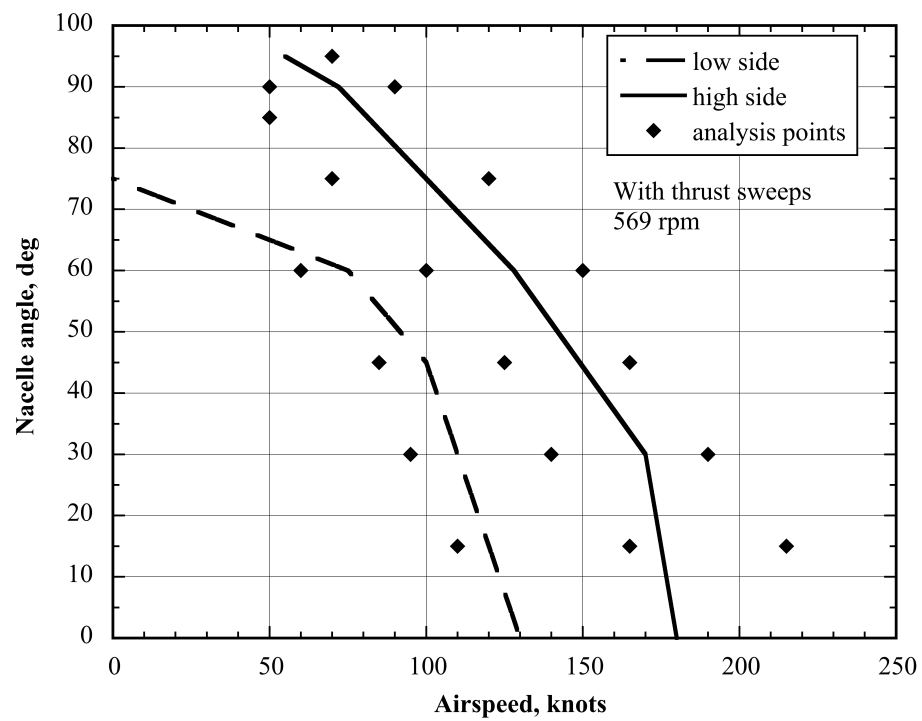
Fig. 2. Approximate AW609 conversion corridor (Refs. 7 and 9) and current pre-test 609 rotor analysis points, 569 rpm.
