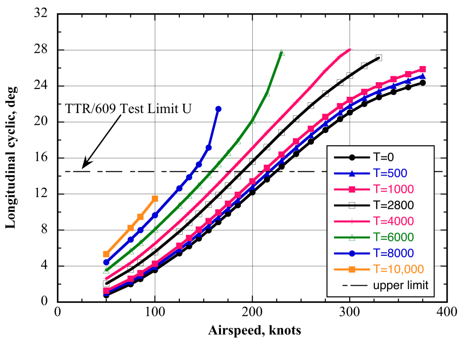
Fig. 10d. Predicted TTR/609 conversion (axial and edgewise flow) longitudinal cyclic vs. airspeed, 45-deg yaw, 569 rpm.
