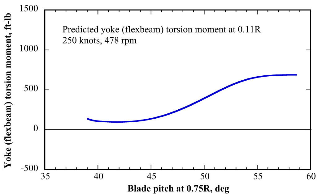
Fig. 6d. Predicted 609 cruise (axial flow) yoke torsion moment vs. collective, 0-deg yaw, 250 knots, 478 rpm.
