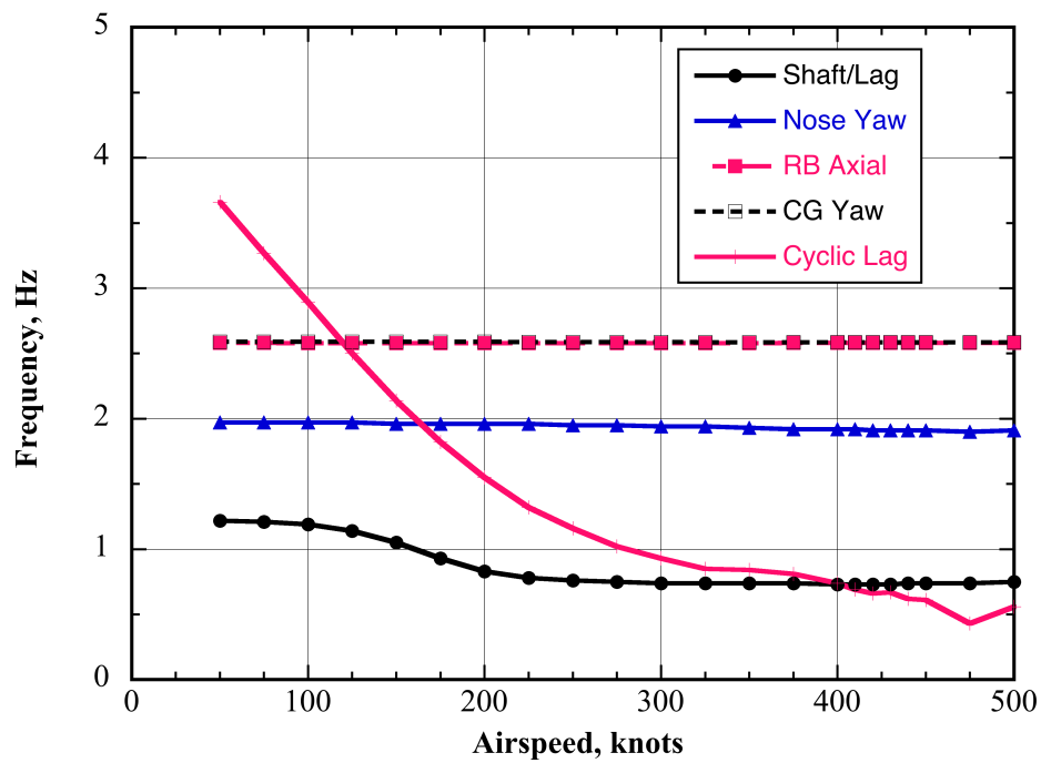
Fig. 9b. Predicted TTR/609 cruise (axial flow) frequencies vs. airspeed, 0-deg yaw, 0 power, 478 rpm.
