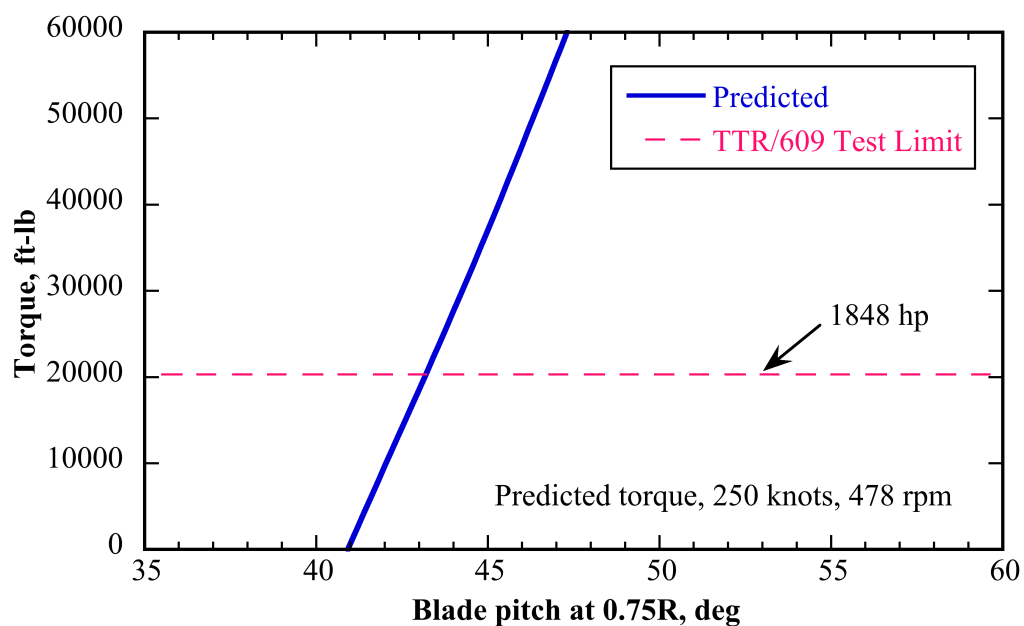
Fig. 6b. Predicted 609 cruise (axial flow) torque vs. collective, 0-deg yaw, 250 knots, 478 rpm.
