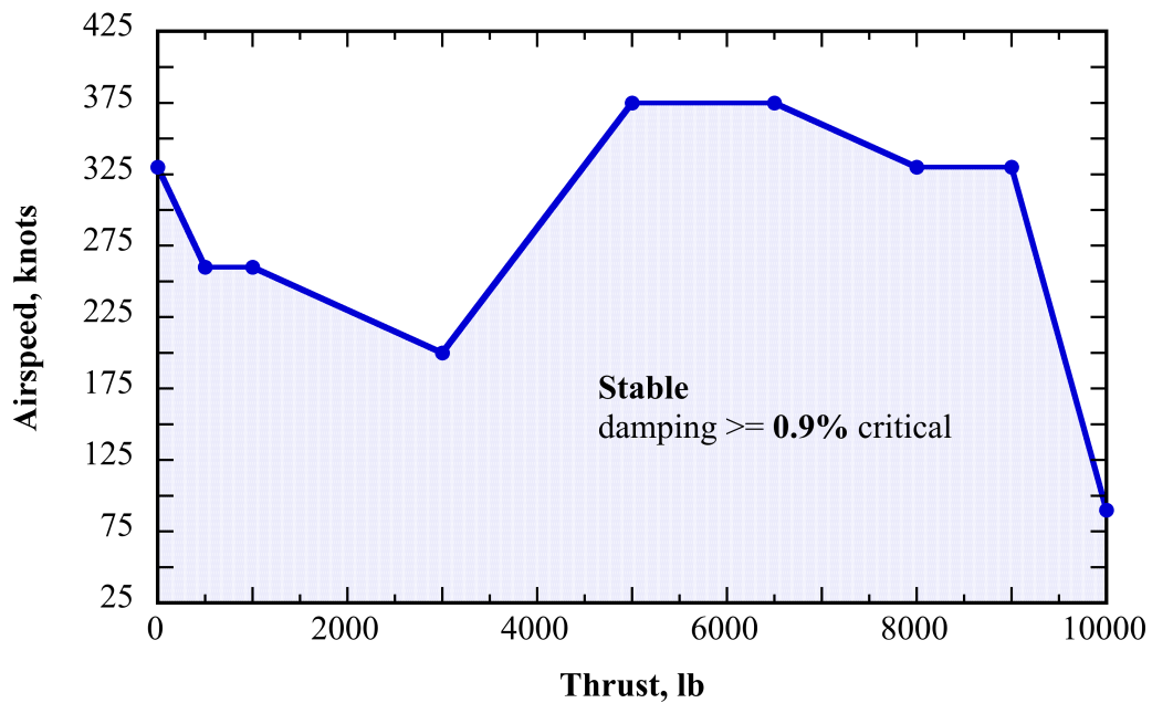
Fig. 11c. Predicted TTR/609 helicopter mode (axial and edgewise flow) 0.9% damping stability envelope, 90-deg yaw, 569 rpm (shake test modal data).
