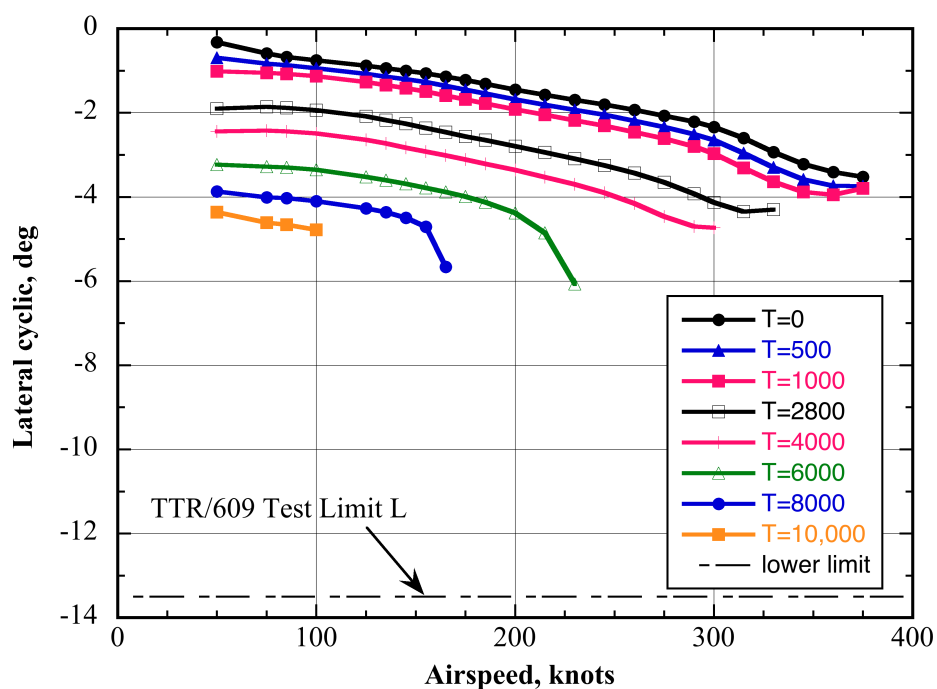
Fig. 10c. Predicted TTR/609 conversion (axial and edgewise flow) lateral cyclic vs. airspeed, 45-deg yaw, 569 rpm.
