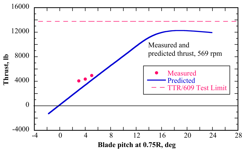
Fig. 5a. 609 hover thrust vs. collective, 569 rpm.
