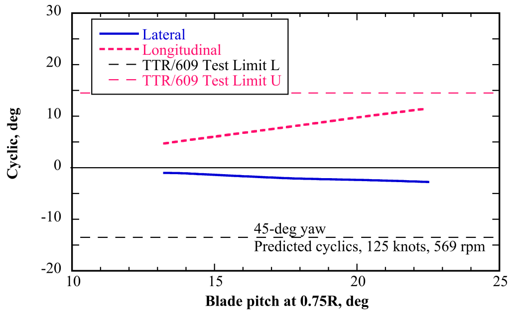
Fig. 7g. Predicted 609 conversion (axial and edgewise flow) trim cyclics vs. collective, 45-deg yaw, 125 knots, 569 rpm.
