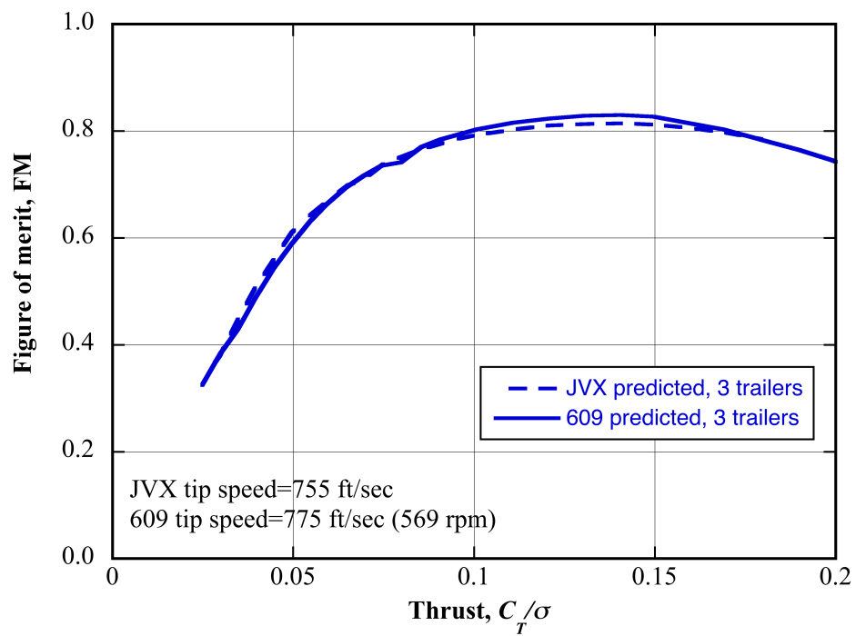
Fig. 3b. Reality check, JVX and 609 predicted figure of merit comparison (based on Ref 8).
