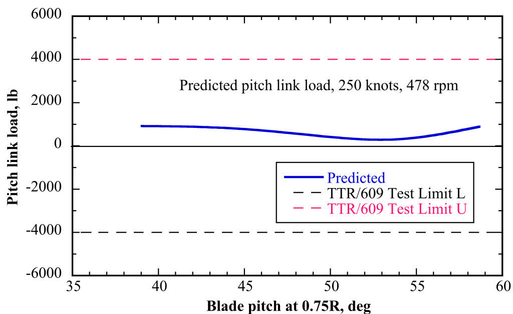
Fig. 6c. Predicted 609 cruise (axial flow) pitch link load vs. collective, 0-deg yaw, 250 knots, 478 rpm.
