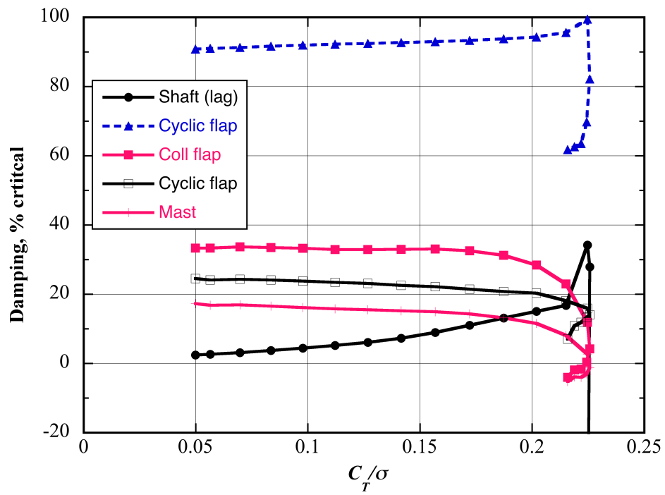
Fig. 8a. Predicted TTR/609 hover damping vs. thrust, 0-deg yaw, 569 rpm.
