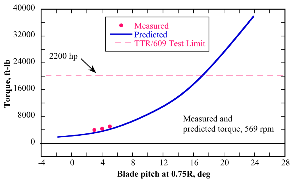
Fig. 5b. 609 hover torque vs. collective, 569 rpm.
