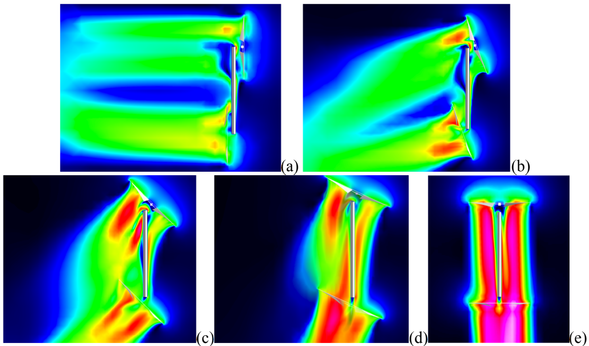
Figure 31. Velocity magnitude flow field predictions for simplified PIVOT model: (a) roll angle = 0 Deg.; (b) 20 Deg.; (c) 45 Deg.; (d) 65 Deg.; (e) roll angle = 90 Deg.
