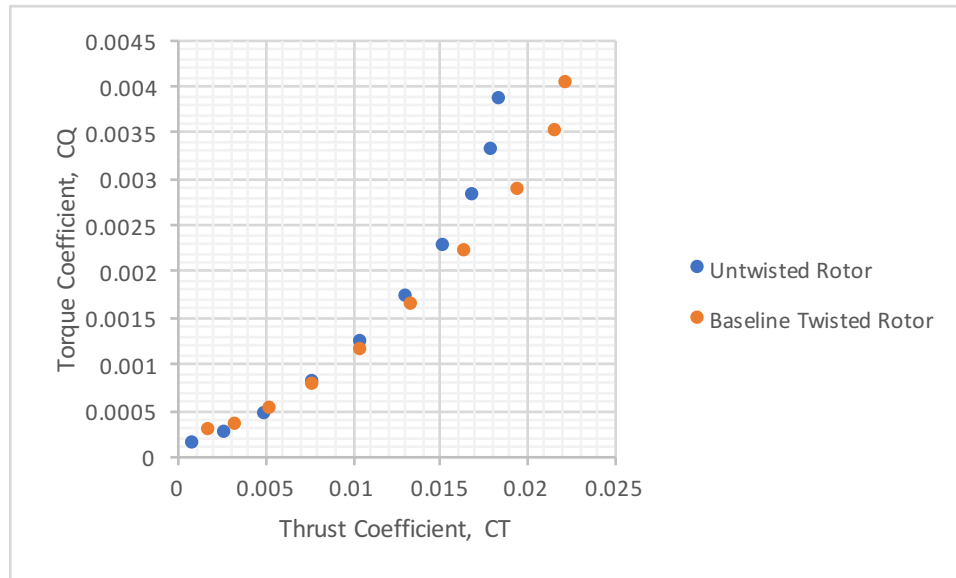
Figure 15. FLEX isolated “lifting rotor” hover performance
