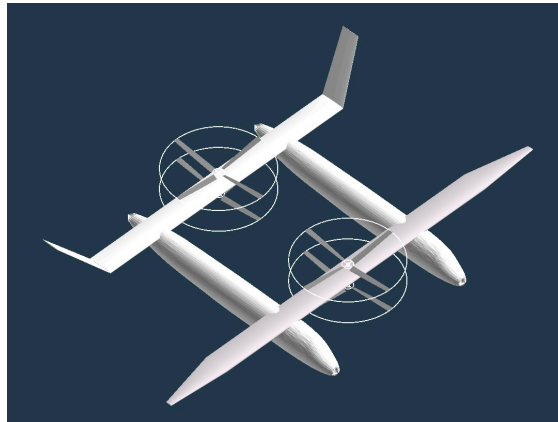
Figure 19. Twin Hull Type-B: coaxial tiltrotor proprotors at mid-span of wings
