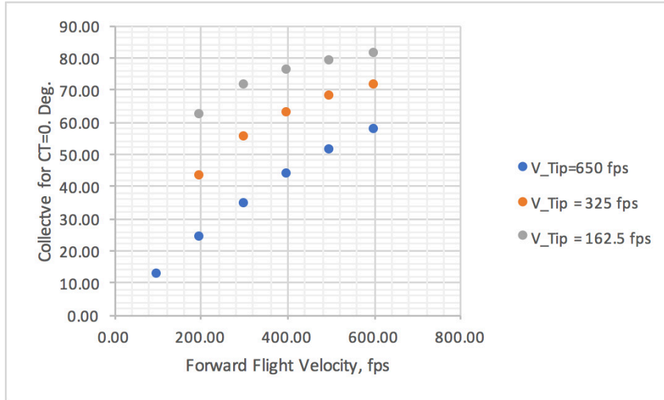
Figure 16. FLEX “lifting-rotor” zero-thrust collective trim condition for high-speed forward-flight
