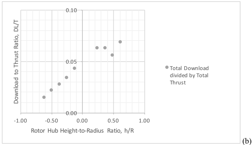
Figure 5. Influence of h/R (above and below the wing) on (a) rotor thrust and (b) wing download
