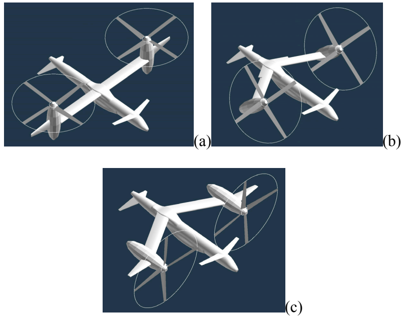
Figure 24. Sweep Type-B vehicle in (a) hover, (b) transition, and (c) cruise
