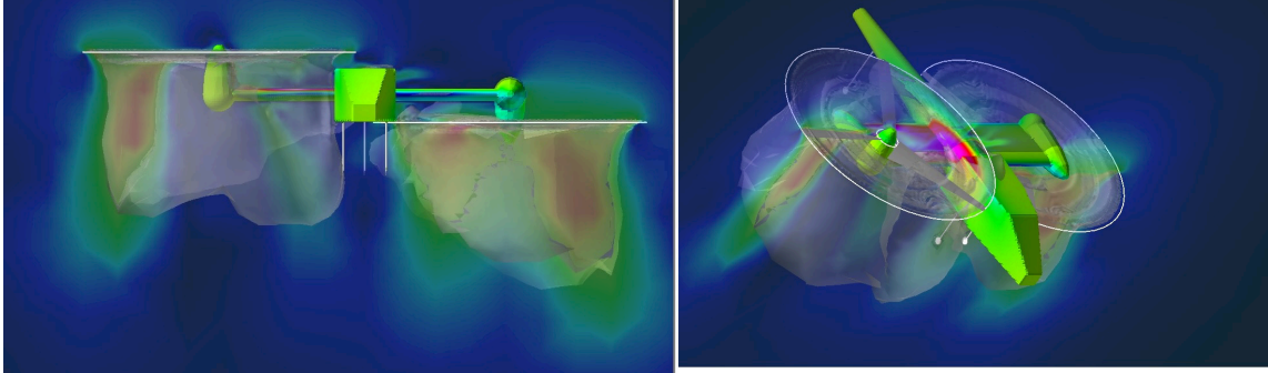
Figure 30. Takeoff from ground with (alternate) landing-gear (note additional degree of freedom with respect to proprotor/nacelle tilt)
