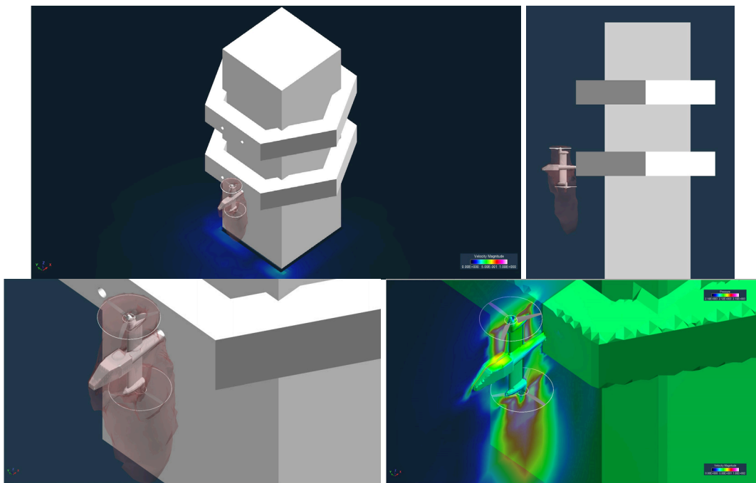
Figure 28. Urban canyon “aerie” perching on building
