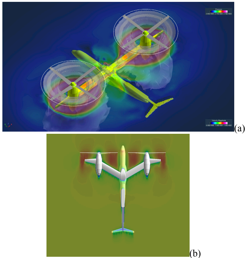
Figure 23. Sweep Type-A Notional Vehicle: (a) orthogonal and (b) planform views
