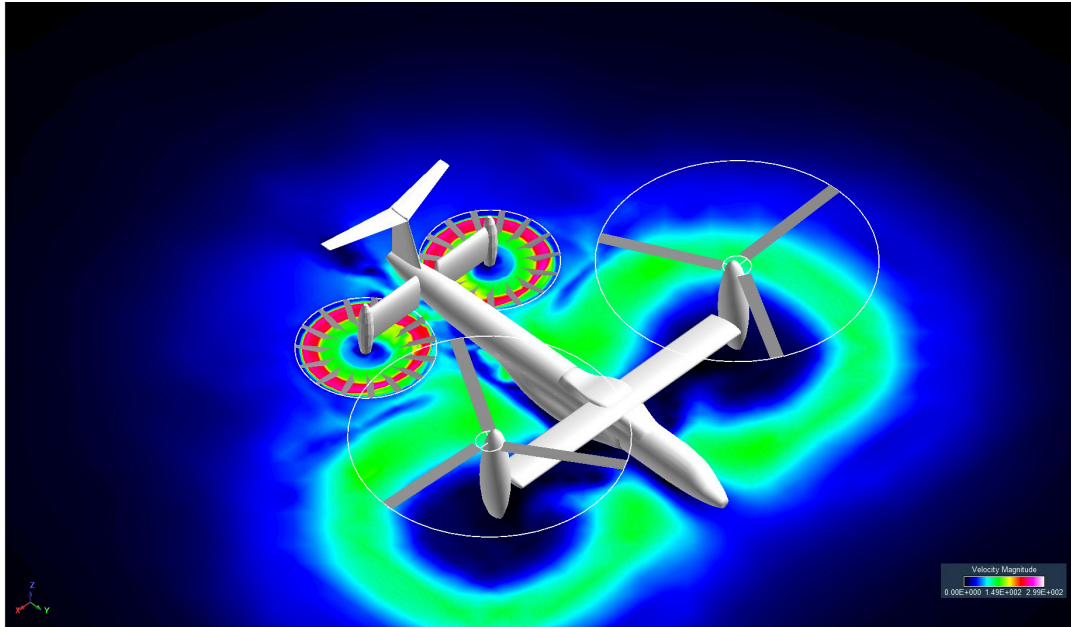
Figure 13. Flex Type-A vehicle
