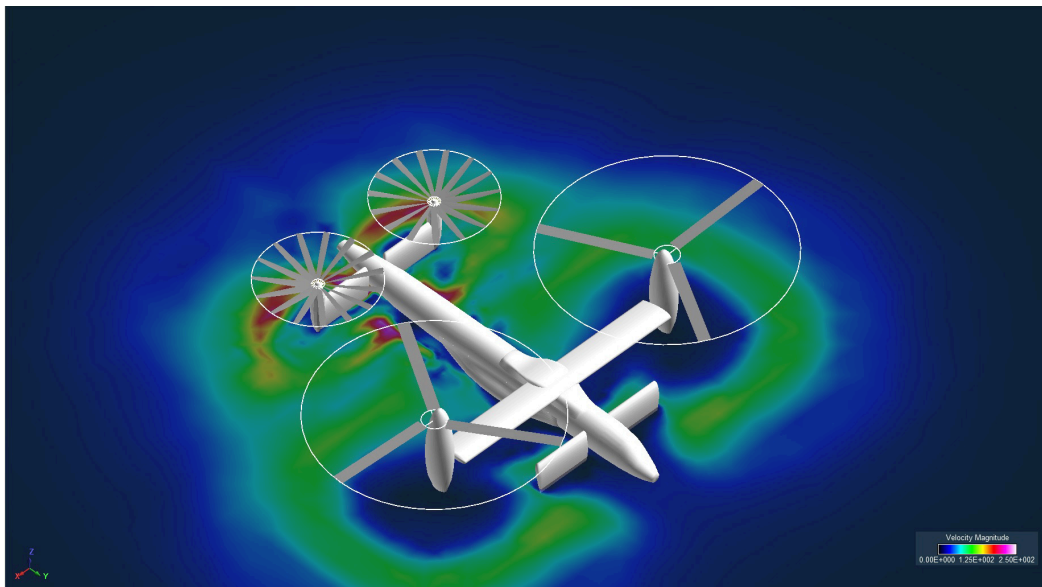
Figure 14. Flex Type-B vehicle
