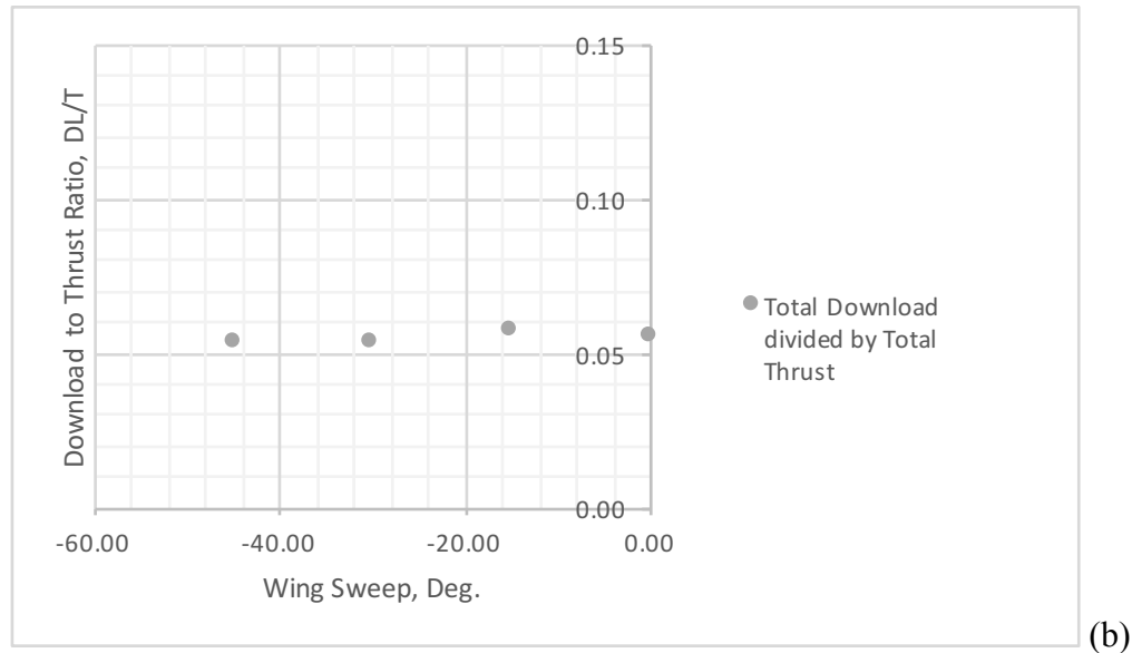
Figure 27. Influence of wing sweep on (a) rotor hover thrust and (b) vehicle download
