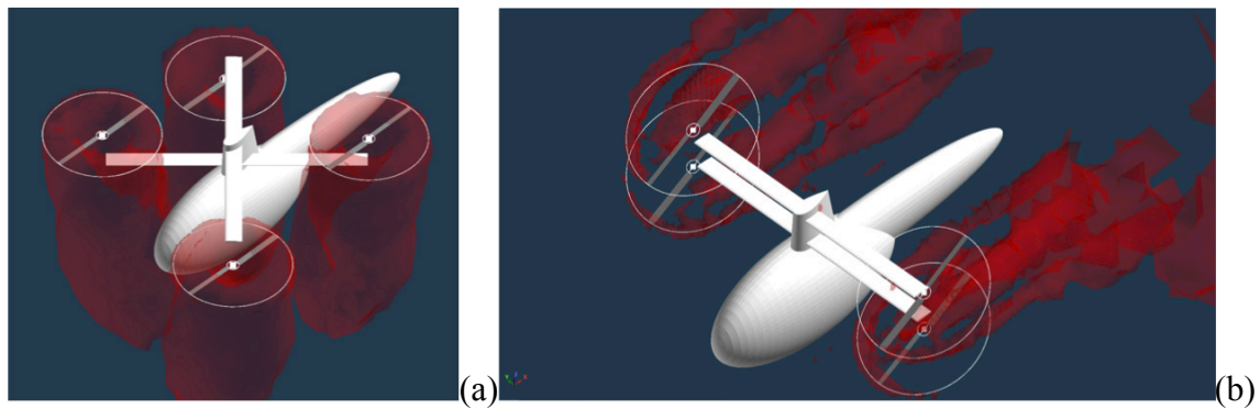
Figure 35. Initial CFD work on AUAT: (a) rotor wakes (velocity magnitude isosurface) in hover and (b) cruise (nondim. Q-criterion isosurface)
