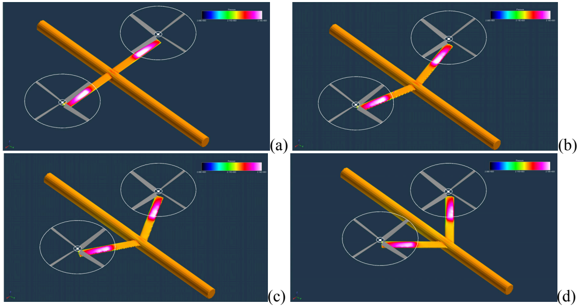
Figure 26. Wing upper-surface pressures for hover with different wing sweep angles: (a) \lambda = 0 Deg.; (b) -15 Deg.; (c) -30 Deg.; (d) \lambda = -45 Deg.
