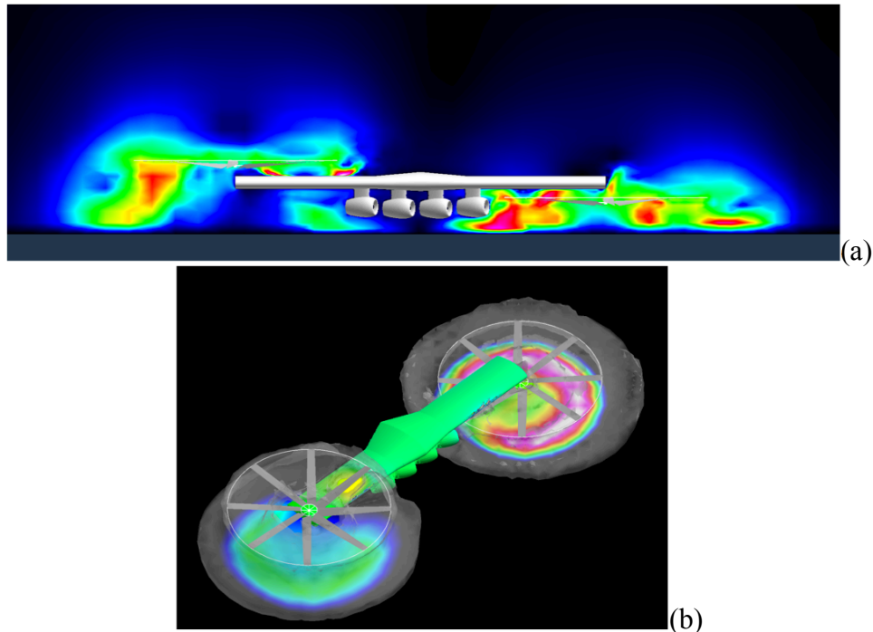
Figure 6. Hover in ground effect: (a) front view and (b) orthogonal view
