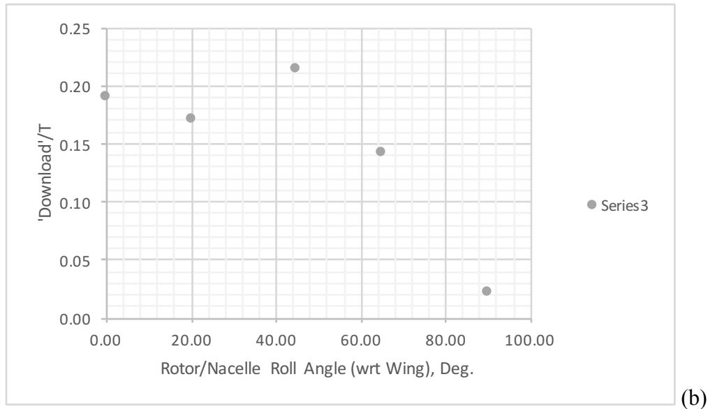
Figure 33. Influence of rotor roll angle on: (a) ‘upper’ and ‘lower’ rotor thrust and (b) wing download-to-total-thrust ratio
