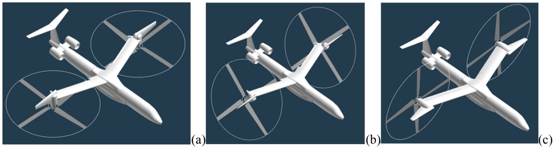
Figure 1. Pusher Proprotor Tiltrotor (PPT): (a) hover, (b) transition, (c) cruise
