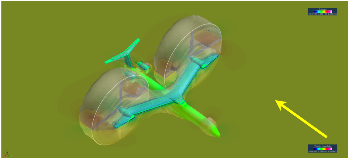
Figure 3. RotCFD prediction of a PPT in forward flight
