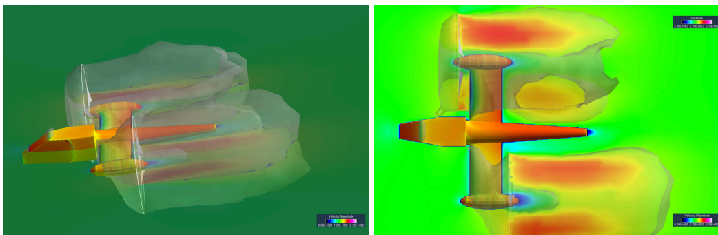
Figure 29. PIVOT in forward-flight cruise
