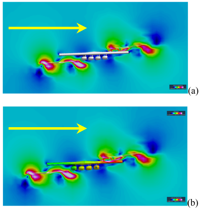
Figure 7. Low-speed air taxi in oriented as a tandem configuration: (a) rotor wake and (b) surface pressures
