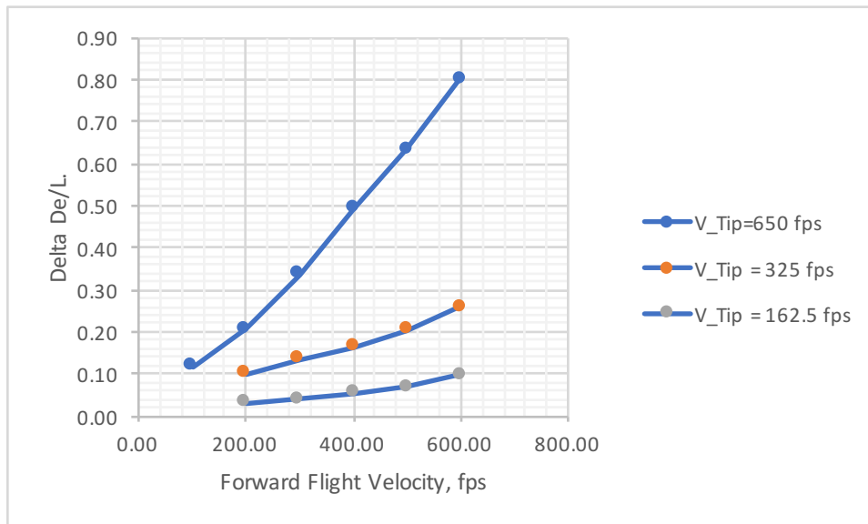
Figure 17. FLEX “lifting-rotor” delta-De/L effect on vehicle forward-flight performance as a consequence of the lifting-rotors being trimmed in the zero-thrust state
