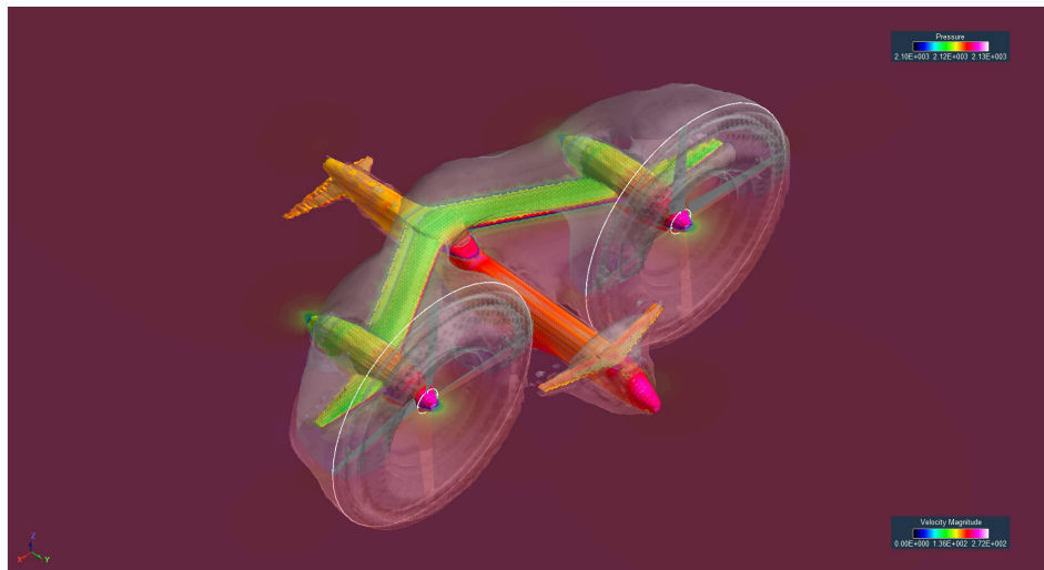
Figure 25. RotCFD forward flight prediction of Type-B variable sweep vehicle
