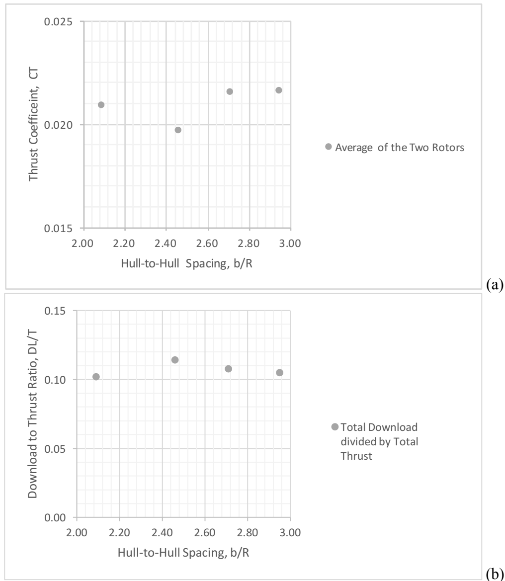
Figure 22. Influence of rotor spacing between the fuselage hulls on (a) rotor hover thrust and (b) vehicle download
