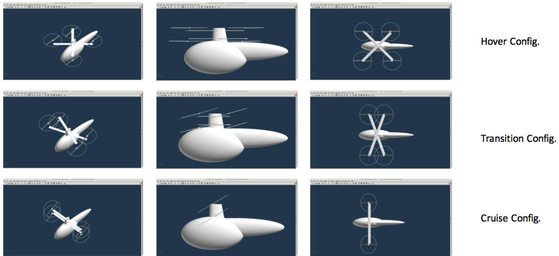
Figure 34. Ames Urban Air Taxi: not quite a tiltrotor aircraft
