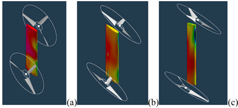
Figure 32. (Lower) body surface pressures for simplified PIVOT model: (a) roll angle = 0 Deg., (b) roll=20 Deg., and (c) roll=45 Deg.
