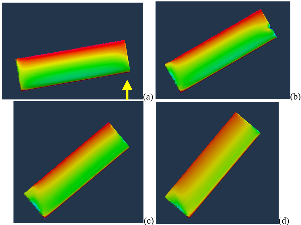
Figure 10. Upper-surface pressure predictions of the isolated wing: (a) \lambda=10 Deg.; (b) 30 Deg.; (c) 40 Deg.; (d) 50 Deg.
