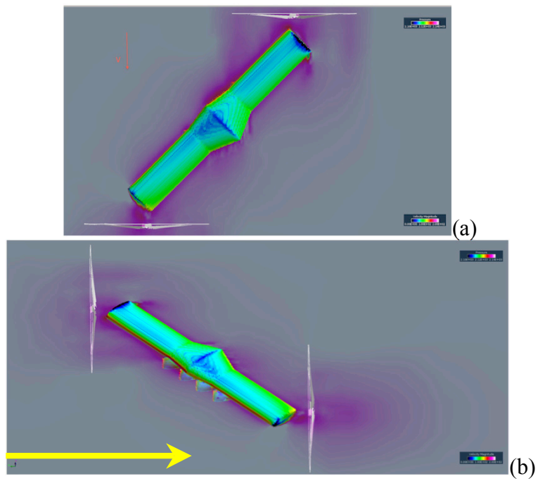
Figure 9. RTOW forward flight cruise: (a) planform view and (b) orthogonal view
