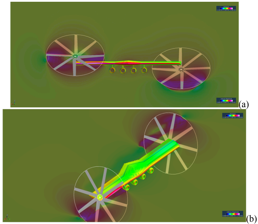
Figure 8. RotCFD predictions of TOW large manned vehicle in transition
