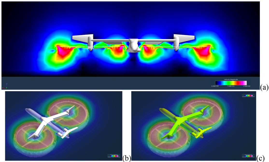
Figure 2. RotCFD prediction of a PPT in hover in ground effect
