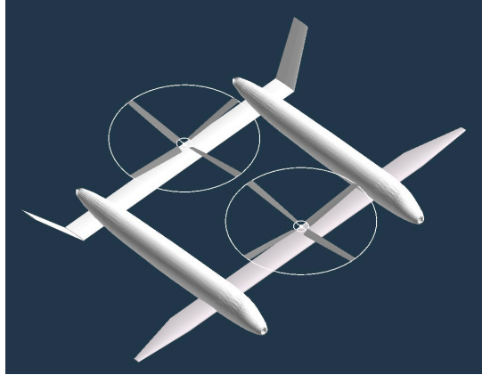
Figure 18. Twin Hull Type-A: single tiltrotor proprotor at mid-span of wings
