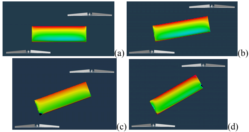
Figure 11. Upper-surface pressure predictions for the combined wing/rotor system in cruise: (a) \lambda=0 Deg.; (b) 10 Deg.; (c) 20 Deg.; (d) 30 Deg.
