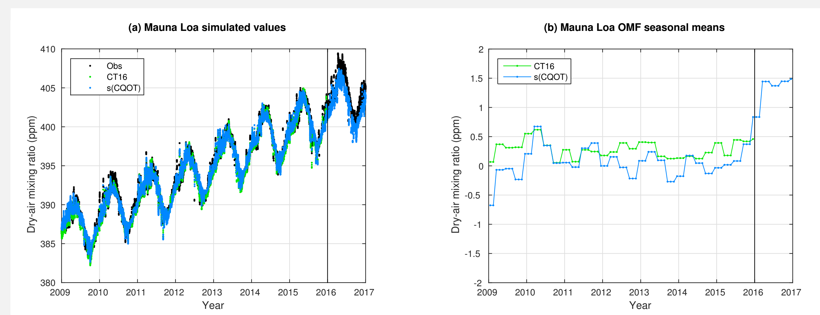
Fig 3. (Left) Simulations using CT16 fluxes (green) and s(CQOT) fluxes (blue) in the GEOS model and observations (black) at Mauna Loa. (Right) 3-month means of the obs. minus model differences (right). The black line at 2016 indicates the switch from reanalysis (R) to near real time (NRT) modes.
