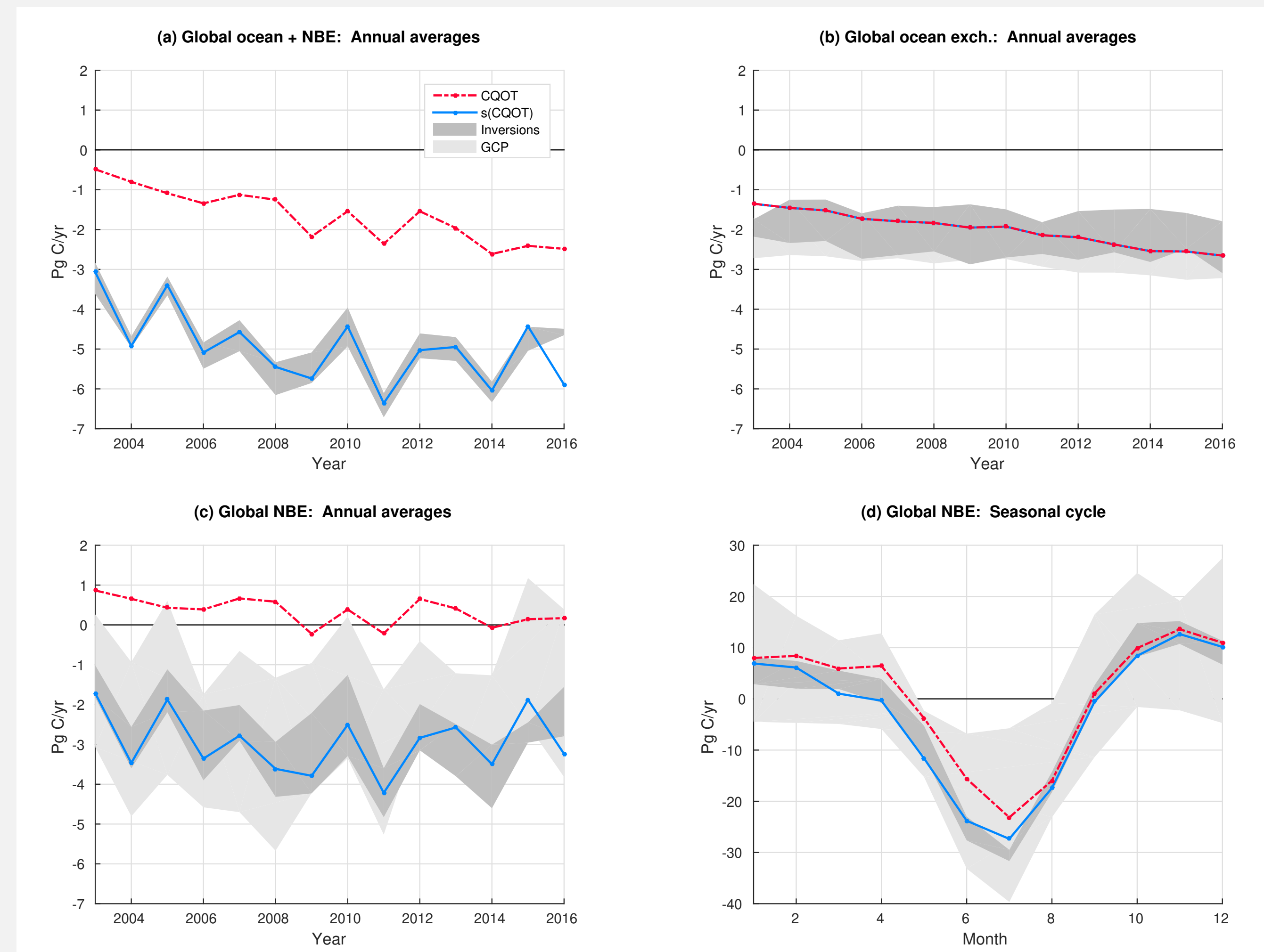
Fig 1. Global total ocean and NBE (NEE + fire) fluxes from the fluxes excluding (CQOT; dash-dot red) and including (s(CQOT; solid blue) the empirical sink compared to the ranges of the inversion ensemble (dark grey) and TRENDY model ensemble (light grey).
