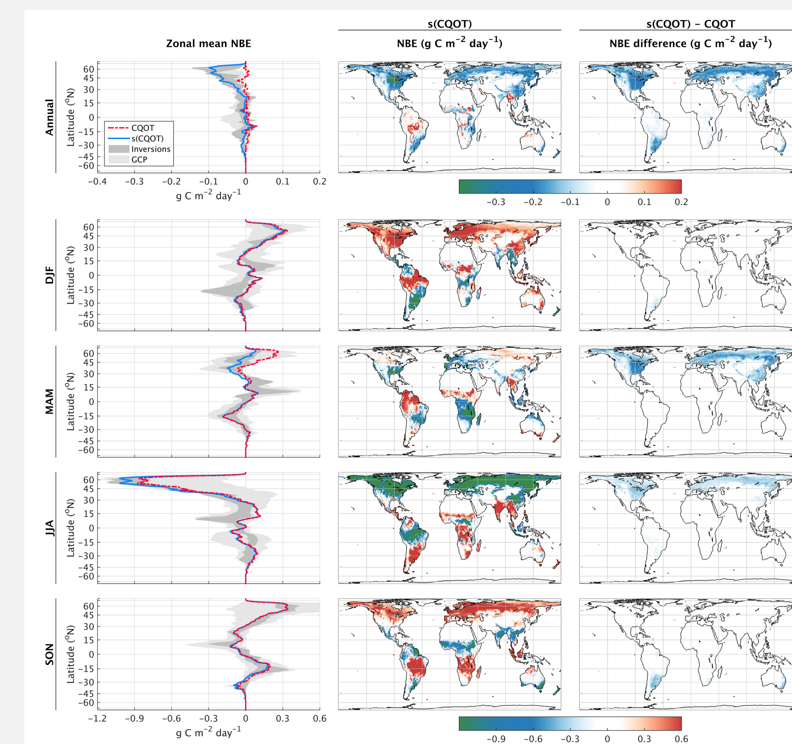
Fig 2. Climatologies (2003—2016) of NBE from the fluxes excluding (CQOT) and including (s(CQOT) the empirical sink. The first row represents averages over different seasons. The left column depicts zonal mean NBE from the CQOT fluxes (dash-dot red) and s(CQOT) fluxes (solid blue) and the ranges of the inversion ensemble (dark grey) and the TRENDY model ensemble (light grey); the middle column depicts the s(CQOT) fluxes; and the right column the size of the empirical sink, i.e., the difference between the s(CQOT) and CQOT fluxes. Note that the scale of the annual average plots is three times smaller than that of the seasonal average plots.
