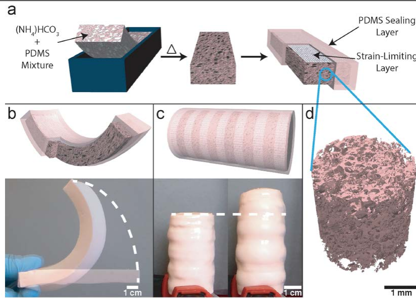
Figure 18: Fabrication process of foam actuators. (a) Molding of a salt foam mixture and patterning fibers to achieve various actuation modes such as (b) bending and (c) extension. (d) Shows an x-ray CT reconstruction of the foam and its large porosity. [36]
