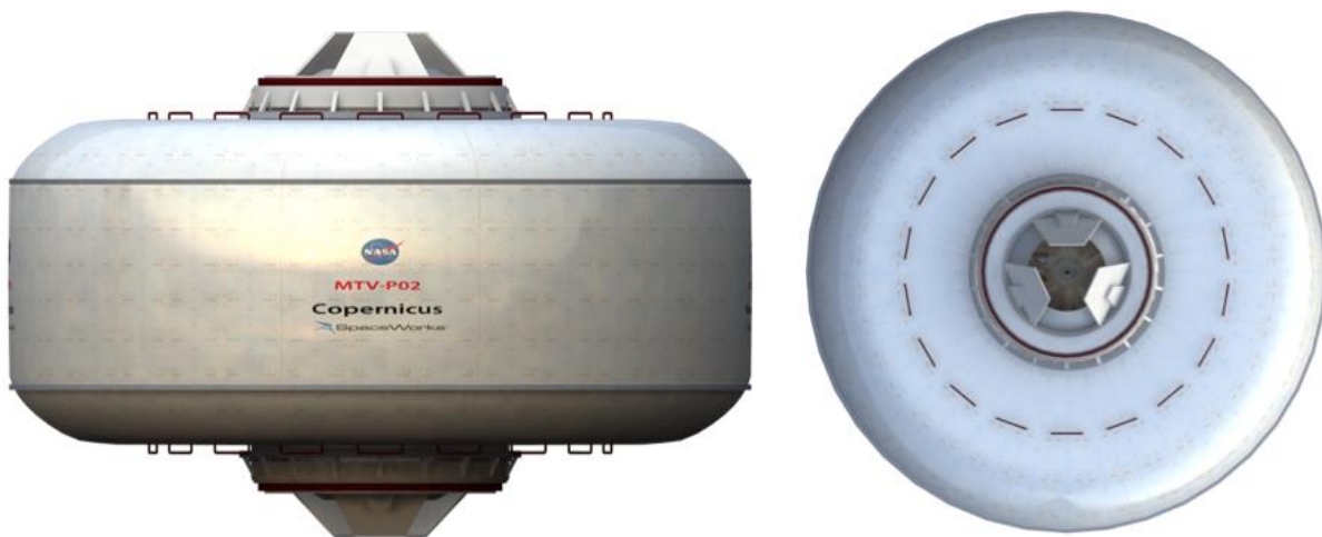
Figure 26. Torpor-Enabled Habitat with Artificial Gravity : External Views
