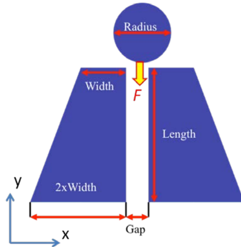
Figure 4: Schematic of nanoscale asymmetry trapezoid structures in 2D views. The incident light will excite the optical resonance of the nanostructure so that gradient optical force will be generated on the nanoparticle and thus the nanoparticle will be accelerated along the negative Y-axis. The arrow shows the direction of the nanoparticle movement.
