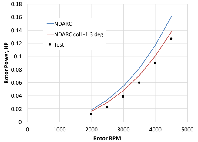
Figure 16. Isolated rotor power in hover – test vs. NDARC
