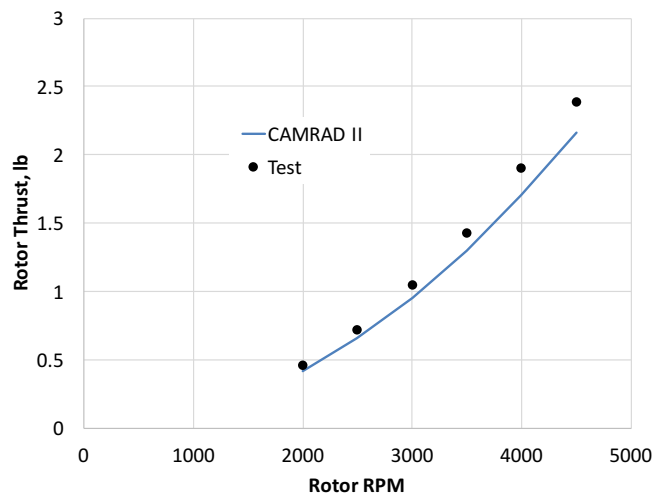
Figure 6. Isolated rotor thrust in hover – test vs. CAMRAD II
