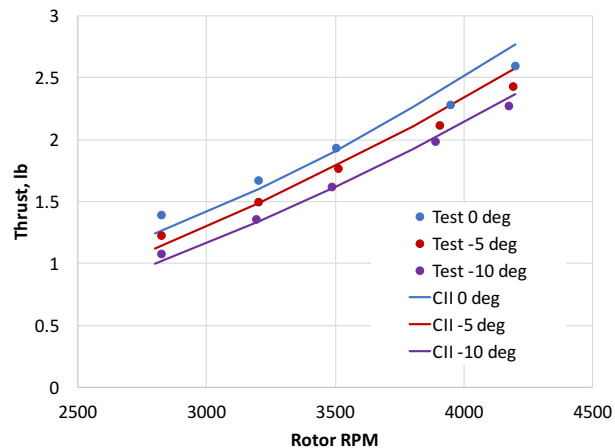
Figure 8. Isolated rotor thrust at 40 ft/s – test vs. CAMRAD II
