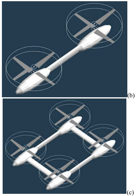
Figure 4 – Modular multi-rotor configurations: e.g. (a) coaxial configurations assembled into (b) quadrotor configurations, which can be further assembled into (c) octocopter, or higher, configurations
