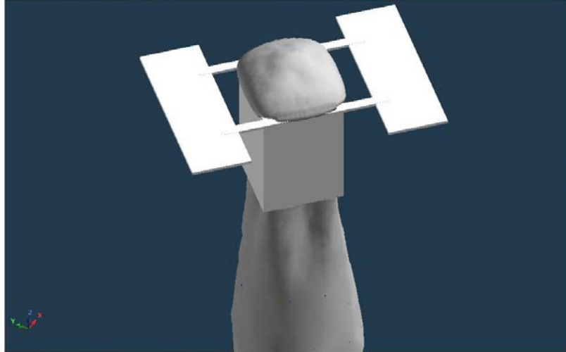
Figure 46 – Rotor Wake Flow Field Prediction (velocity magnitude isosurface) of a Quadcopter with Facade simulating an Asteroid Explorer
