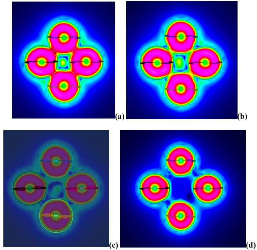
Figure 15 – Representative Multi-Rotor Wake Interaction CFD Results (velocity magnitude at z-plane of z/R = -0.1 ): (a) r/R = 1.41 ; (b) r/R = 1.5 ; (c) r/R = 1.6 ; (d) r/R = 1.82
