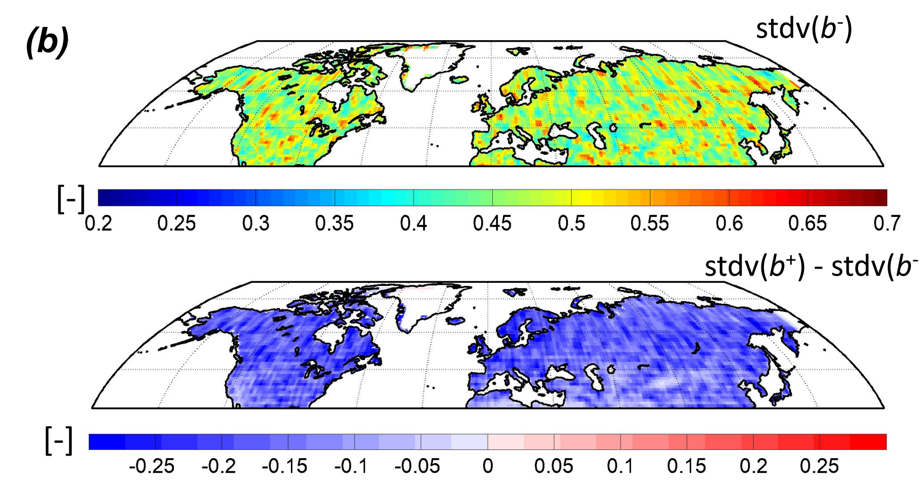
Fig. 3. (a) Example time series of the precipitation errors for a grid in Utah. (b) top: typical monthly ensemble standard deviation (i.e., ensemble spread) of the openloop (i.e., no assimilation), bottom: reduction in ensemble standard deviation ( DA_{stdv} - OL_{stdv} ) between the data assimilation (DA) and openloop for the precipitation errors (b).
