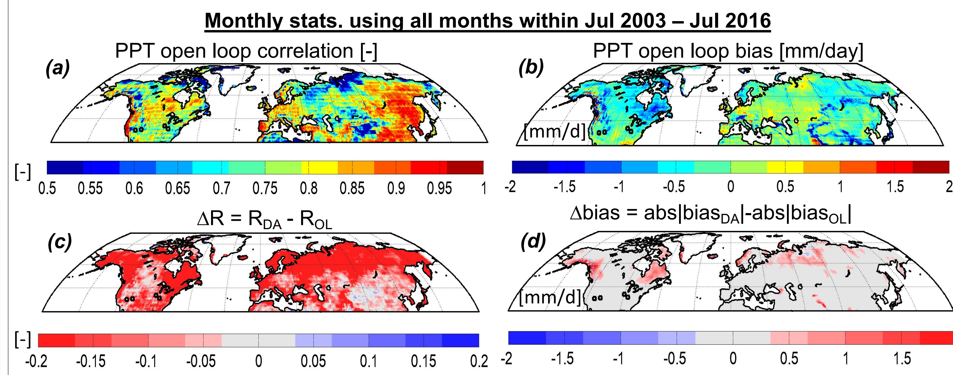
Figure 6. (a) Correlation R and (b) bias skill between open loop (OL) and observed GPCP precipitation (bias is calculated as obs. – OL). (c) \Delta R and (d) \Delta bias difference in skill (between the data assimilation (DA) and openloop (i.e., no assimilation) TWS. This is an independent validation and it suggests that the assimilation of TWS leads to degraded precipitation estimates.
