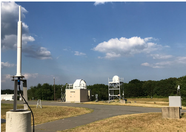
Fig. 3 DORIS beacon at GGAO with the NGSLR prototype system in the background. The SLR aircraft avoidance radar is located on the tower to the right of the NGSLR shelter
