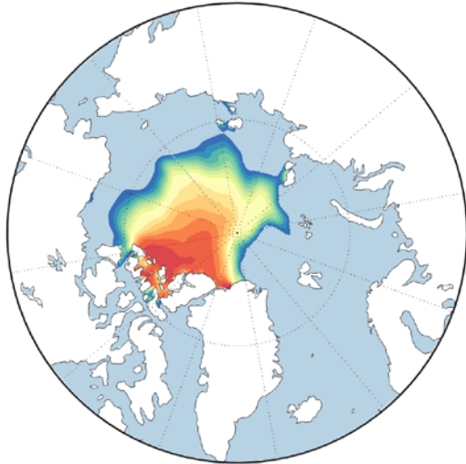
GEOS-S2S Version 2
