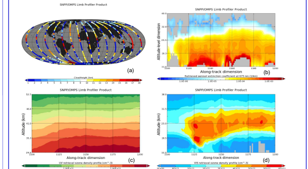
Figure 4: These are demonstrations of S-NPP OMPS L2 products. (a) Cloud height. (b) Retrieved vertical profile of aerosol extinction coefficients at 675 nm between the altitude of 11 – 40 km AGL. (c), (d) Retrieved vertical profiles of ozone density in lower, middle, and upper stratosphere, as well as lower mesosphere.
