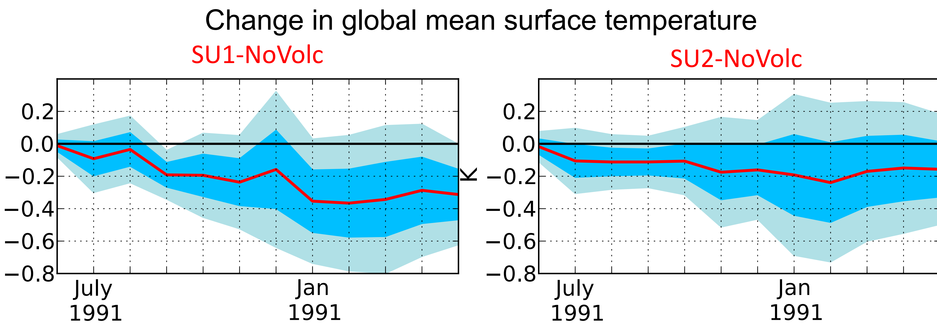
Figure 2: Same as Fig. 1, but for global mean surface temperature. The decrease in SW flux causes a cooling by up to 0.5 K in the ensemble mean. This is significant at 1-σ level in the SU1 experiment, but is not significant in the SU2 experiment.
