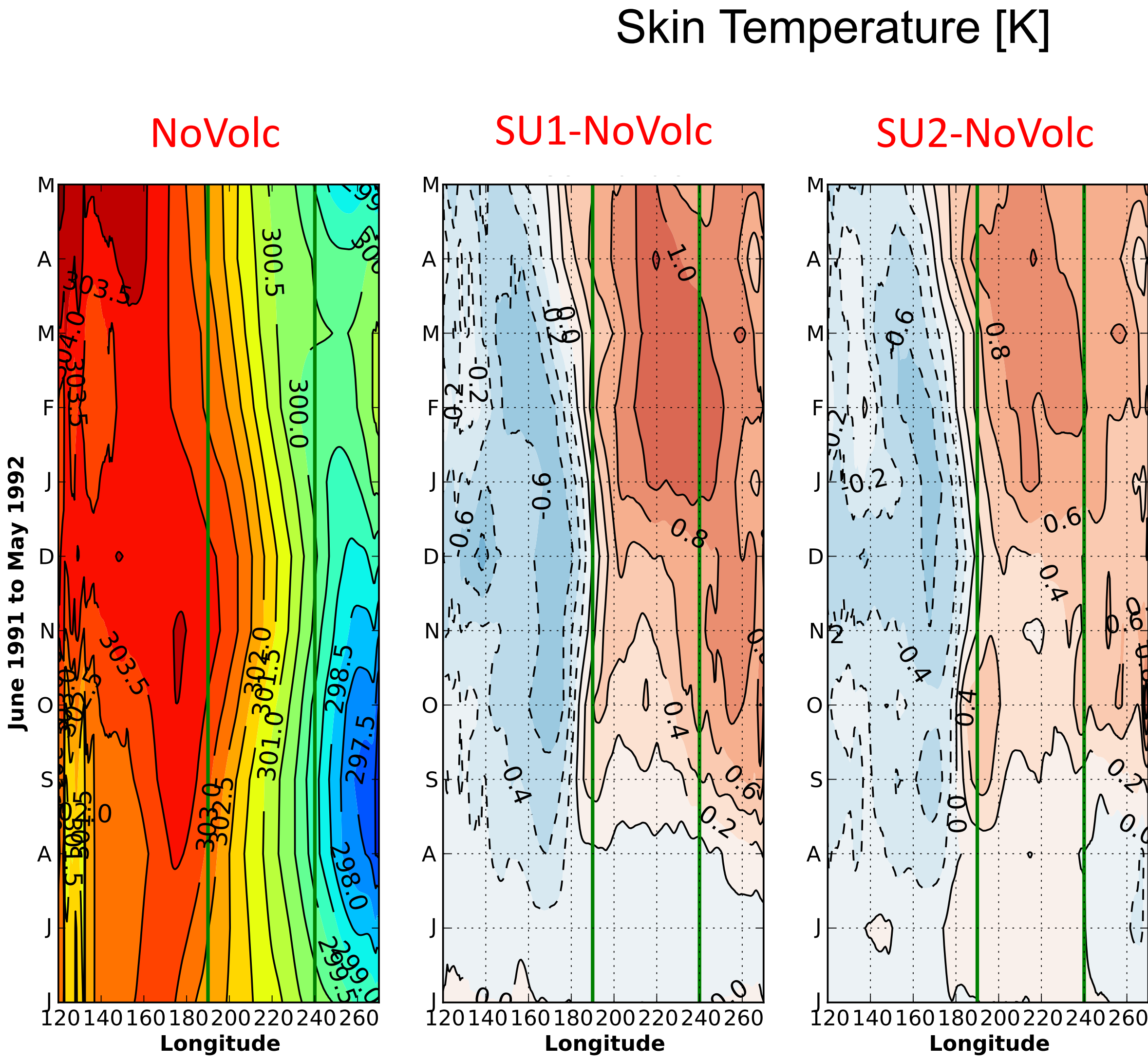
Figure 3: Hovmoller diagram of equatorial skin temperature [5°S-5°N] in NoVolc (left), and equatorial temperature changes in SU1 and SU2 with respect to NoVolc (middle and right). The green lines mark the El Niño 3.4 region. Pinatubo induces a warming of the eastern Pacific. The effect is milder in SU2 than SU1.
