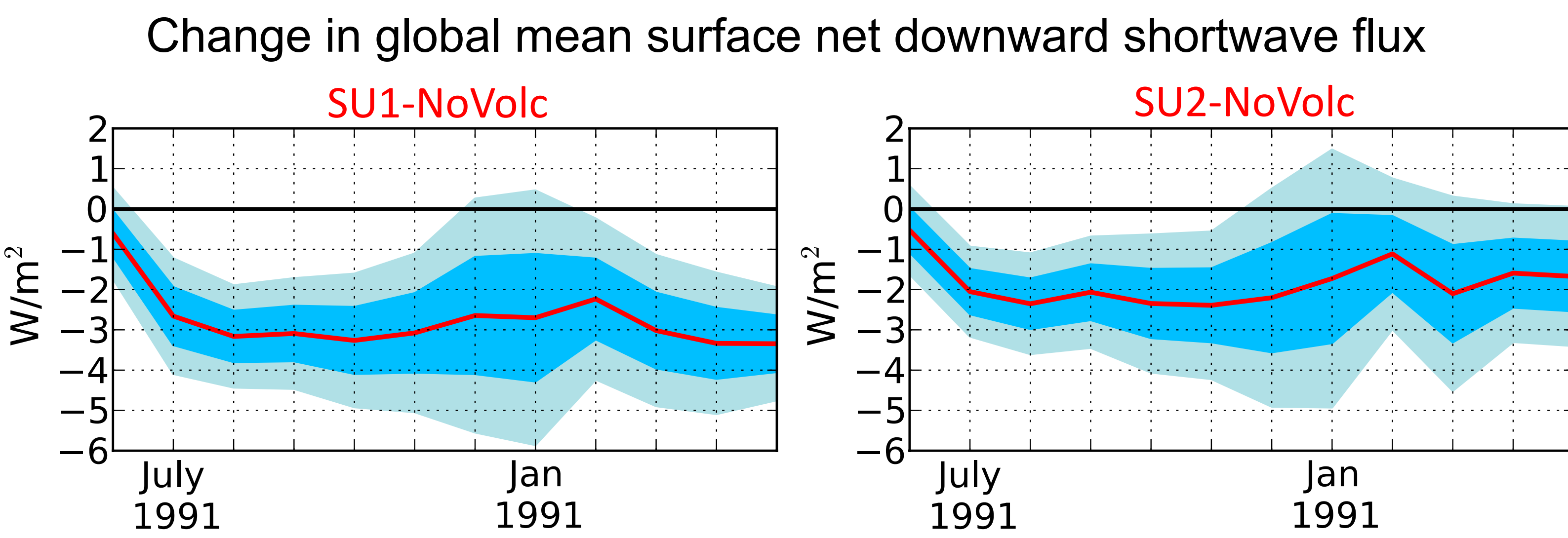
Figure 1: Change in global mean surface net shortwave radiation in the SU1 (left) and SU2 (right) experiments with respect to NoVolc. The red line shows the mean of the difference of 100 randomly chosen pairs of ensemble members. The shaded areas show 1 and 2 standard deviations from the mean. Pinatubo decreased the shortwave flux at the surface. This effect is mildly stronger and longer lasting in the SU1 experiment than in SU2. This is expected, because the scattering efficiency of sulfate particles decreases with size.
