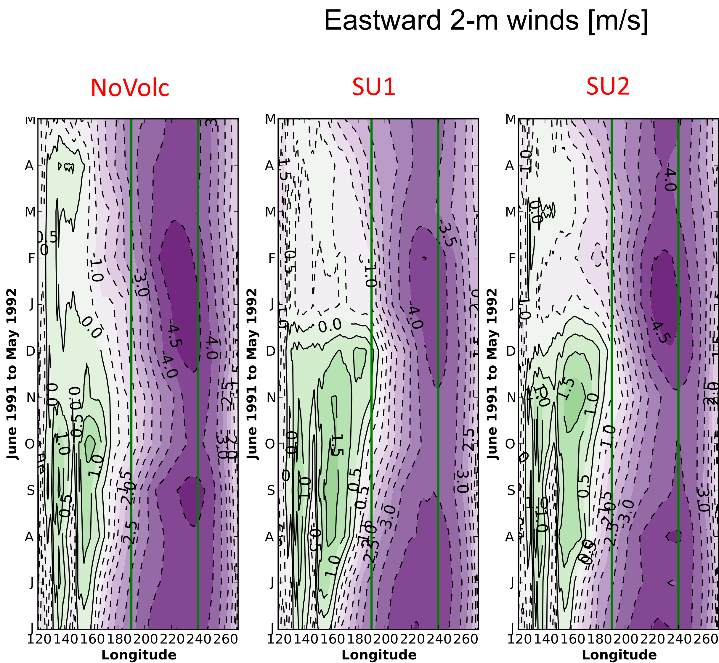
Figure 4: Hovmoller diagram of equatorial winds [5°S-5°N]. Green colors indicate eastward winds. Pinatubo strengthen the eastward winds in the western Pacific.
