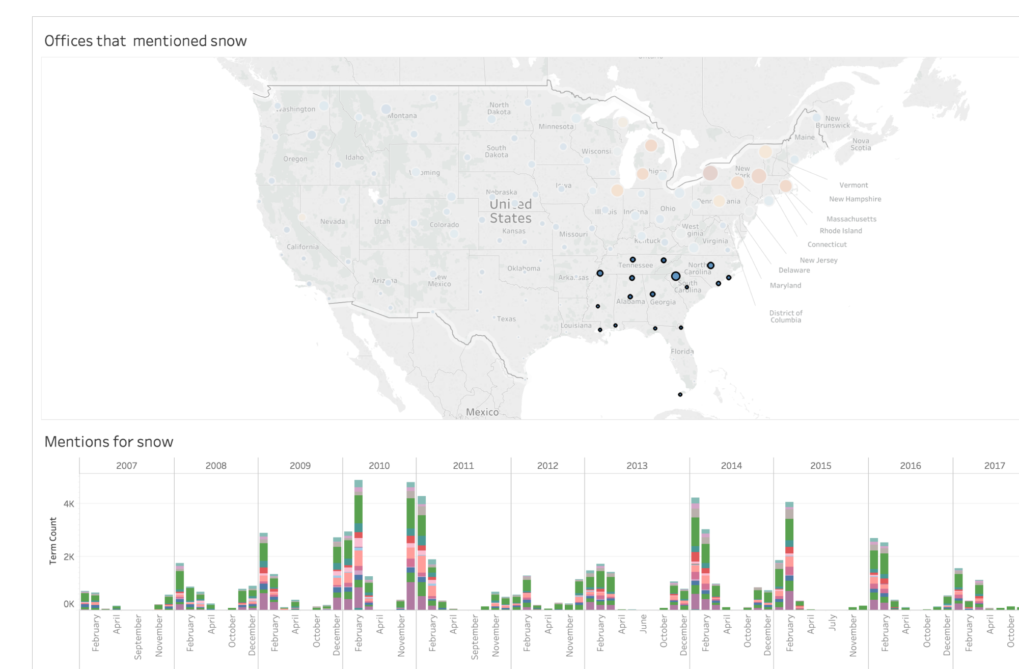
Figure 2 Total extractions for the term “snow” for 2007 – 2017 for the southeastern U.S.
