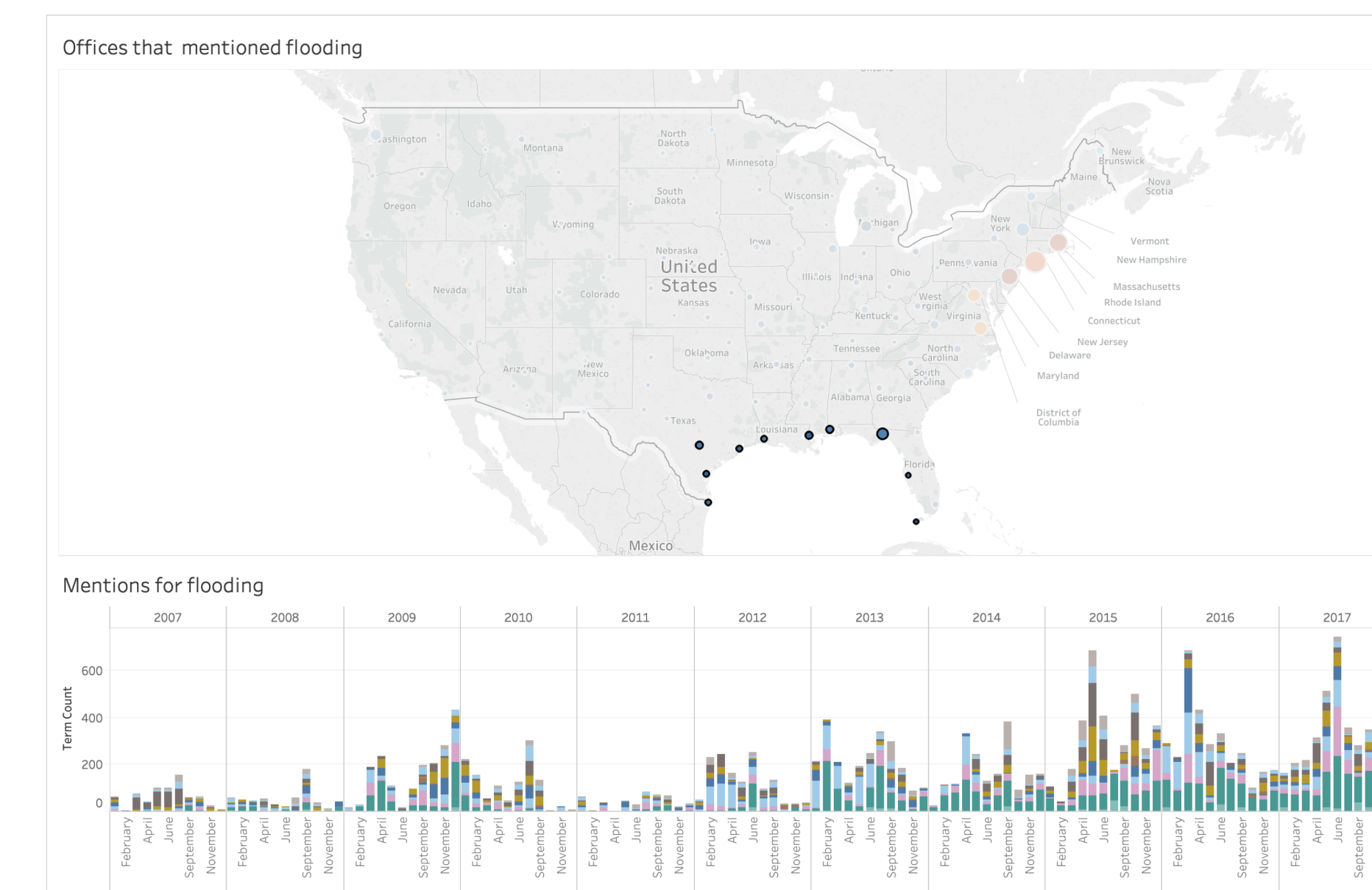
Figure 4 Counts of extractions with “flooding” from 2007 – 2017 for Gulf Coast NWS offices.
