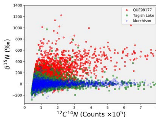
Fig 4. Bin data of isotopic anomalies identified within nitrogen rich regions across sampled matrix areas for each meteorite. All values have errors \delta^{15}\text{N} < 75 \text{ ‰} .
