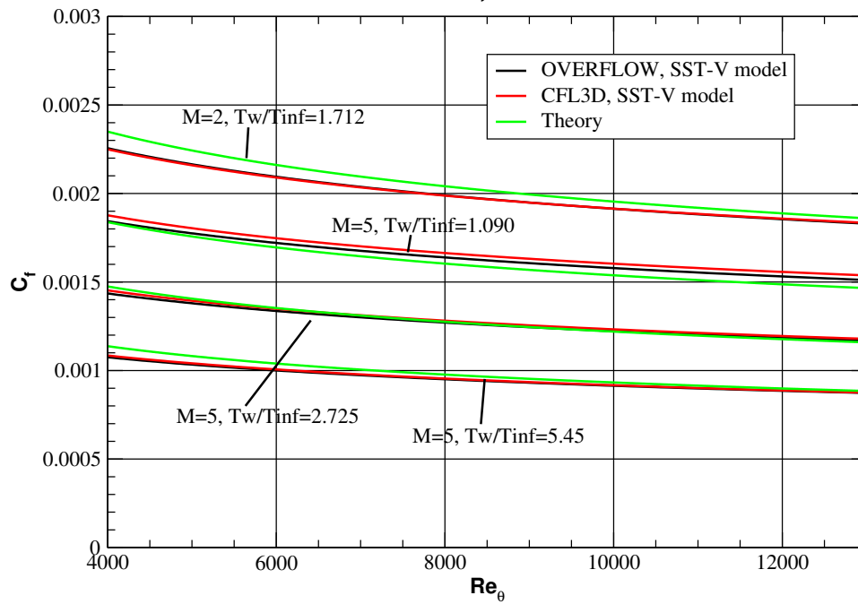
Figure 13.5: Skin friction, SST-V model.
