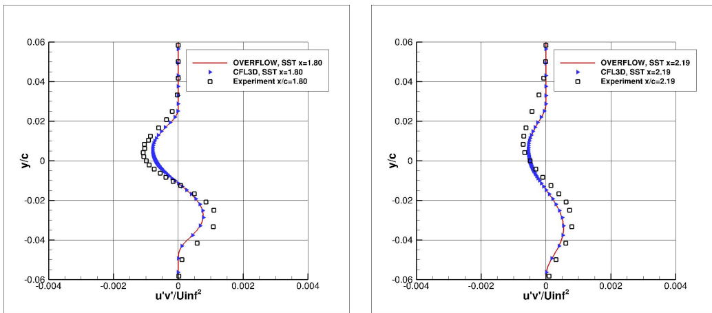
Figure 6.14: Turbulent shear stress profiles, SST model, x = 1.80 and x = 2.19 .
