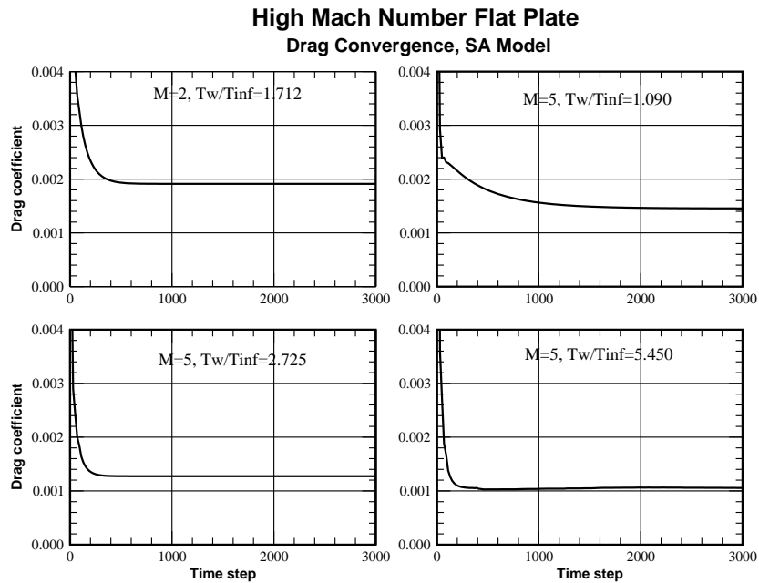
Figure 13.2: Drag convergence, OVERFLOW, SA model.
