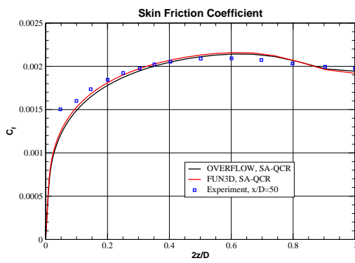
Figure 19.9: Skin friction and crossflow velocity, SA-QCR model.
