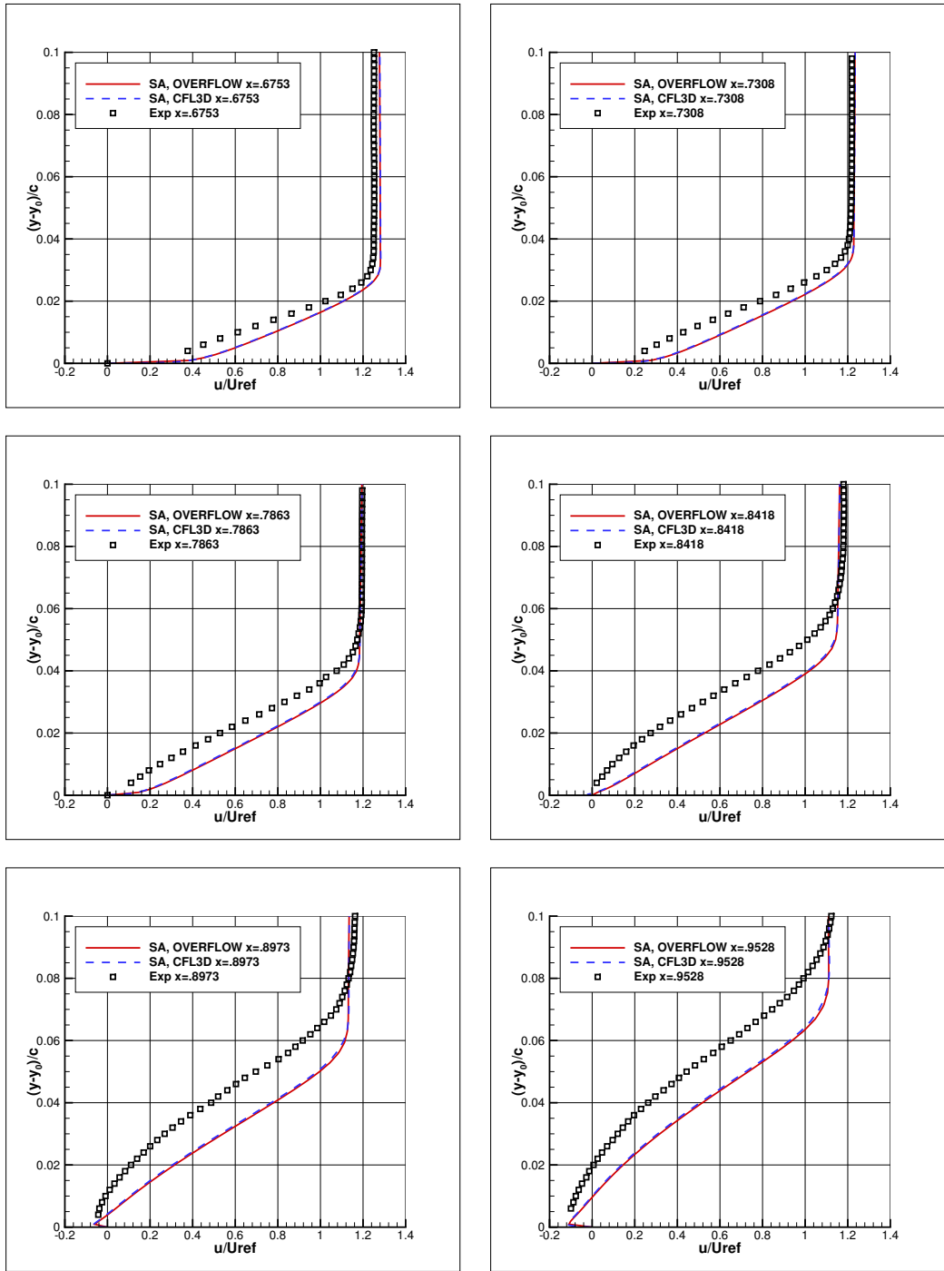
Figure 15.4: Streamwise velocity profiles, SA model.
