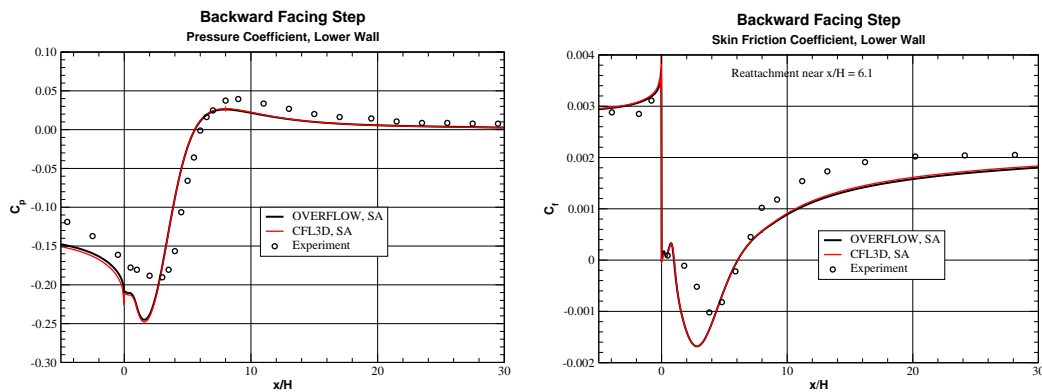
Figure 14.3: Pressure coefficient and skin friction, SA model.
