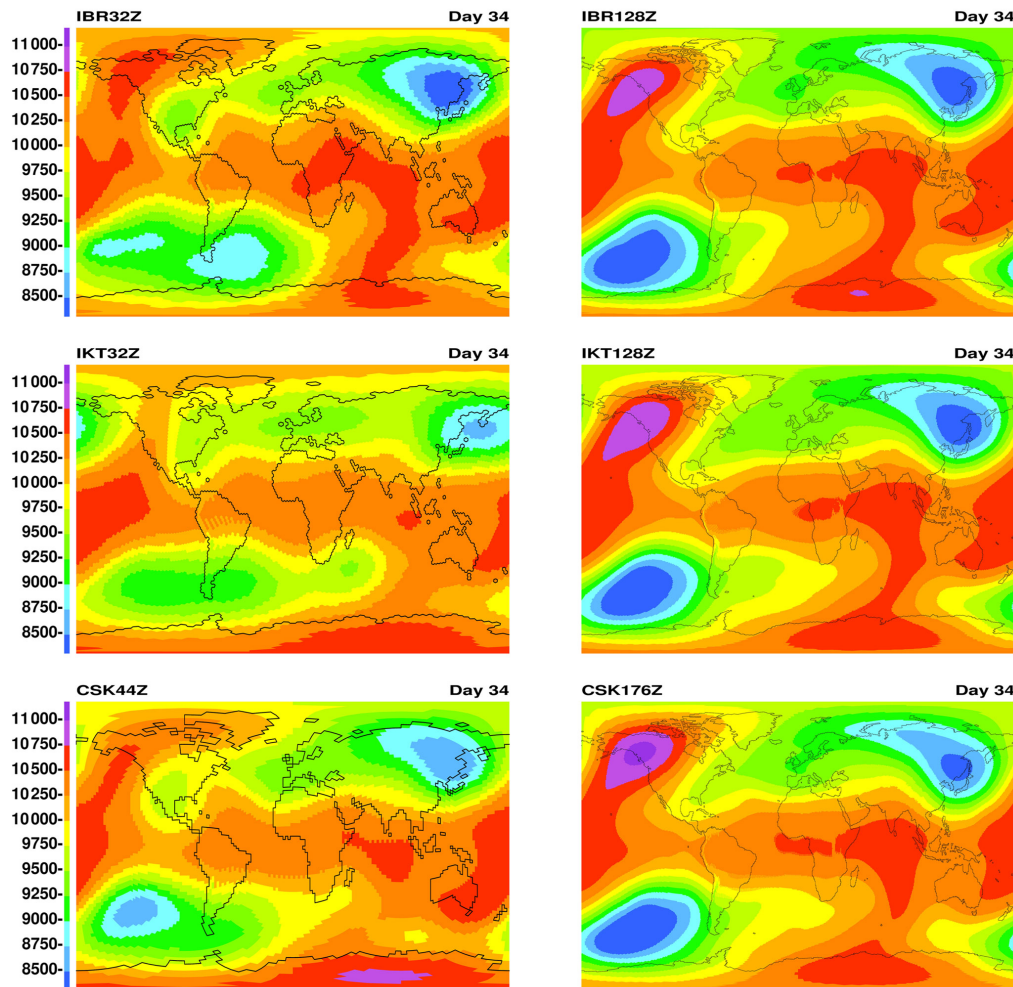
Figure 7. Horizontal plots of h + h_S for models IBR, IKT, and CSK and resolutions 2 and 0.5^\circ after 34 days of integration starting from 50 \text{ m s}^{-1} eastward velocity multiplied by cosine of latitude, global mean height field top of 10 000 m but latitudinal distribution, and Earth’s fixed bottom topography (Test Case 3 SBRZ).
