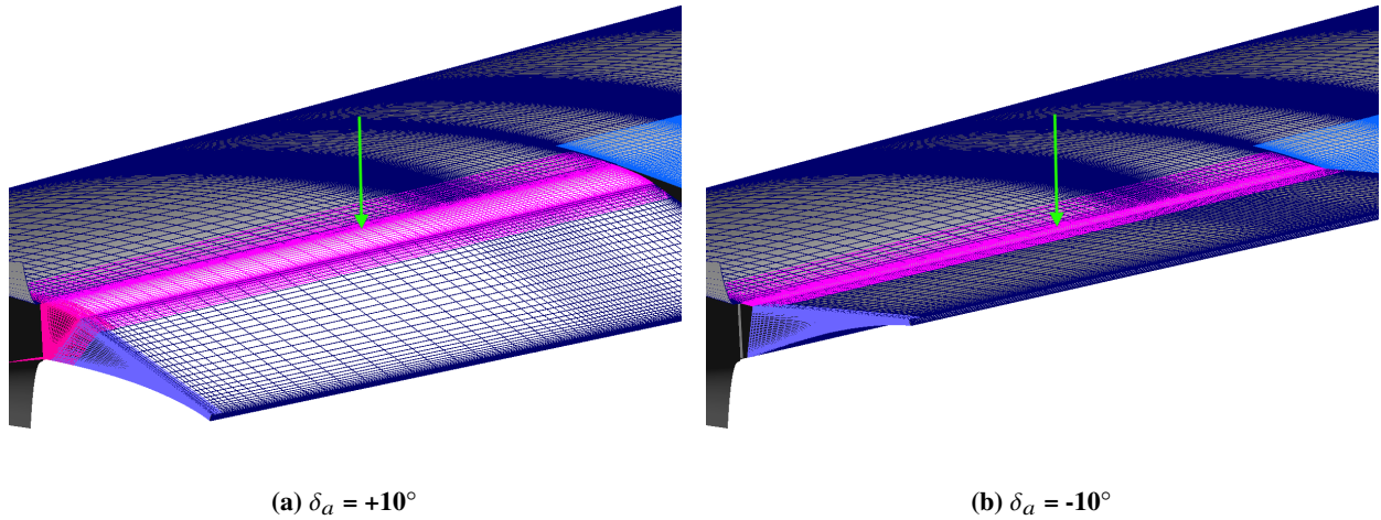
Fig. 5 Patched aileron grid for selected deflections using transfinite interpolation (TFI) surfaces and hyperbolic marching to overlap with surrounding grids (shown in pink).
