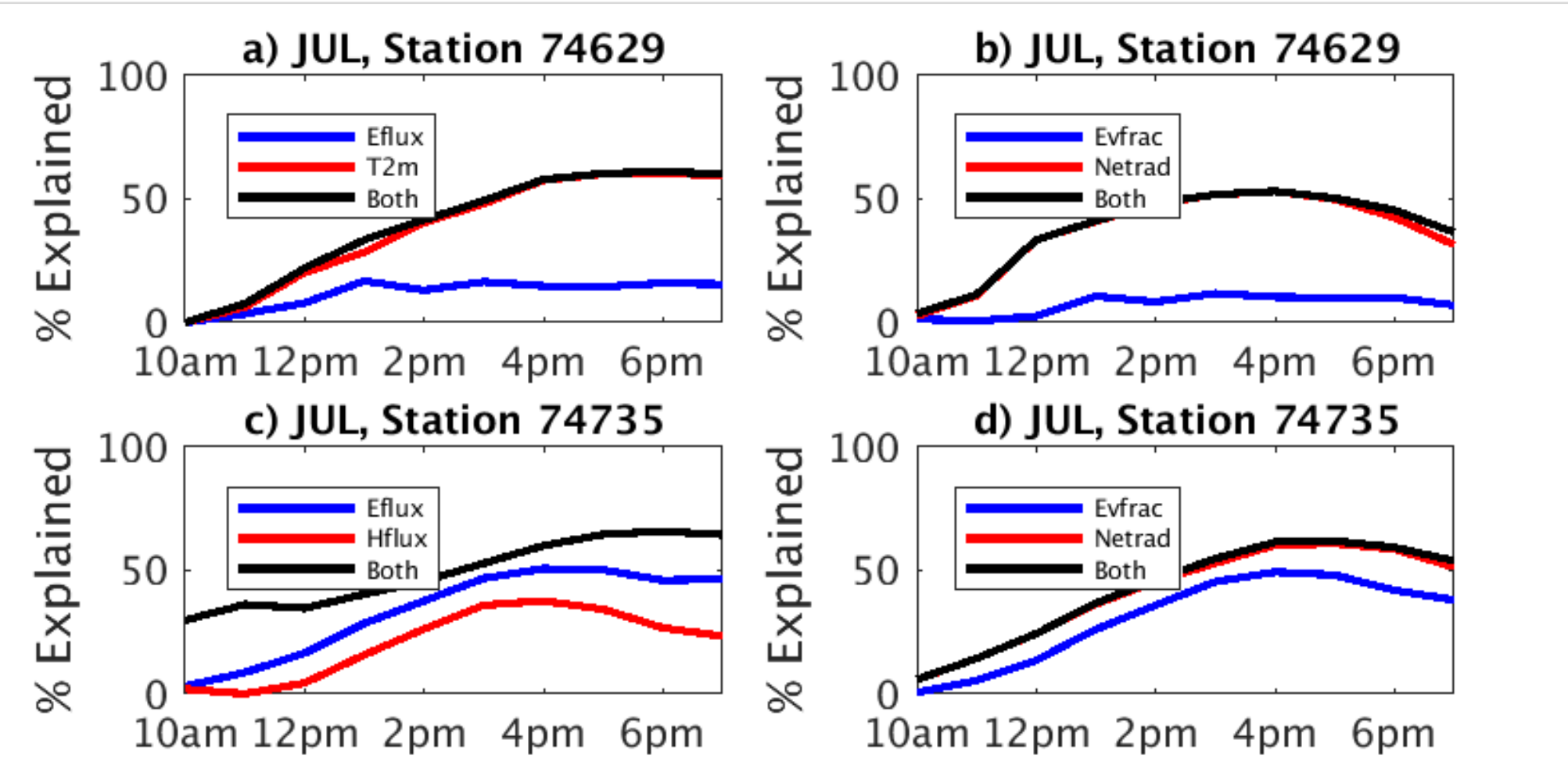
Figure 4: a) Fraction of total PBL height variance explained by latent heat flux, 2-meter temperature, and both at Station 74629 in July, b) fraction explained by evaporative fraction, net surface radiation and both at Station 74629 in July, c) fraction explained by latent heat flux, sensible heat flux and both at Station 74735 in July, d) fraction explained by evaporative fraction, net surface radiation and both at Station 74735 in July.
