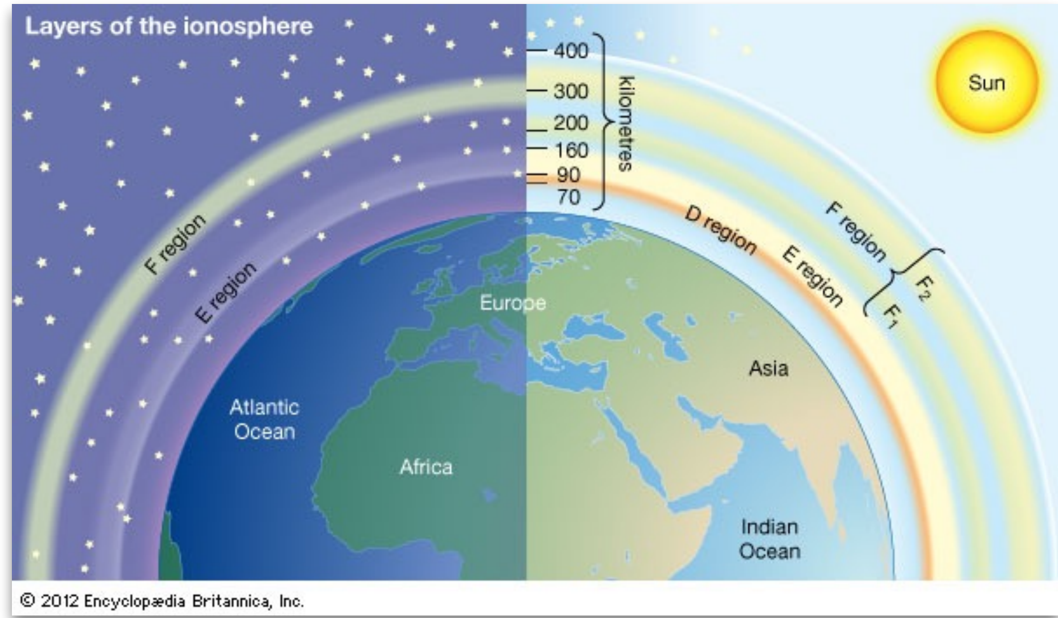
Figure 1: Earth's ionosphere is ionized by radiation from the Sun; here the ionospheric layers are illustrated during both night (left) and day (right)
