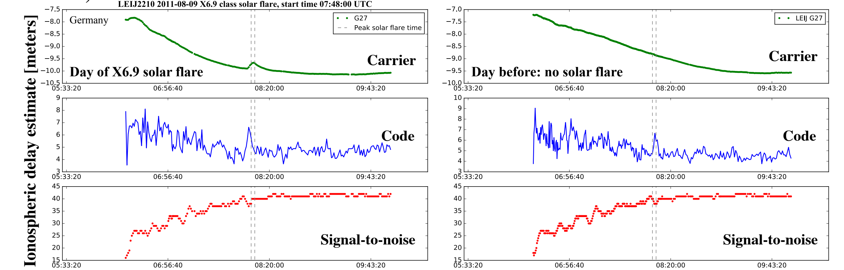
Figure 7: GPS estimates of ionospheric delay plotted with time; the solar flare event is marked by two dashed lines; characteristically smooth carrier phase advance (green) data are plotted on top, followed by noisy pseudorange code delay (blue) in the middle, and receiver-dependent signal-to-noise (red) at the bottom; the total system pseudorange error budget includes the space, control, and user segments with standard deviation values of 7.1 m 2
