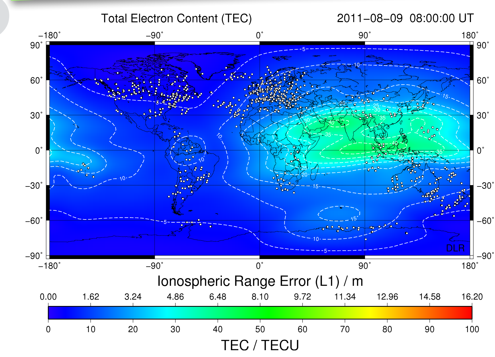
Figure 9: Total electron content (TEC) map for August 09, 2011 at 08:00 UTC provided by SWACI*; dashed contour lines mark the TEC in units of TECU (1 x 10 16 electrons per square meter; color bar scale indicates the ionospheric range error measured at frequency L1 (1575.42 MHz).
