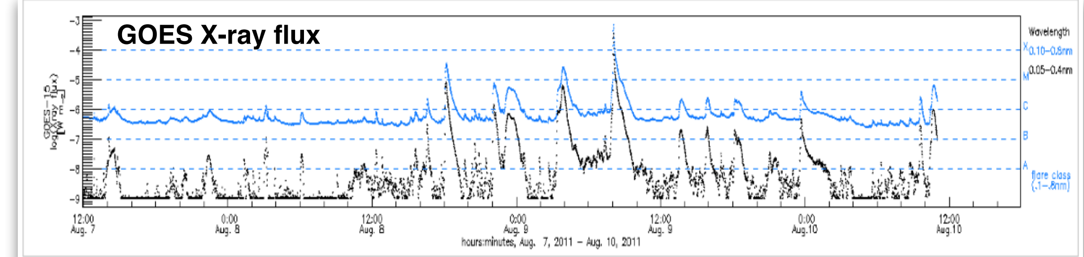
Figure 3: GOES-15 x-ray flux over the time of the solar flare event shown in black (wavelength range = 0.05 - 0.4 nm) and blue (wavelength range = 0.1 - 0.8 nm); the dashed horizontal lines measure flare class (plot from CCMC iSWA)
