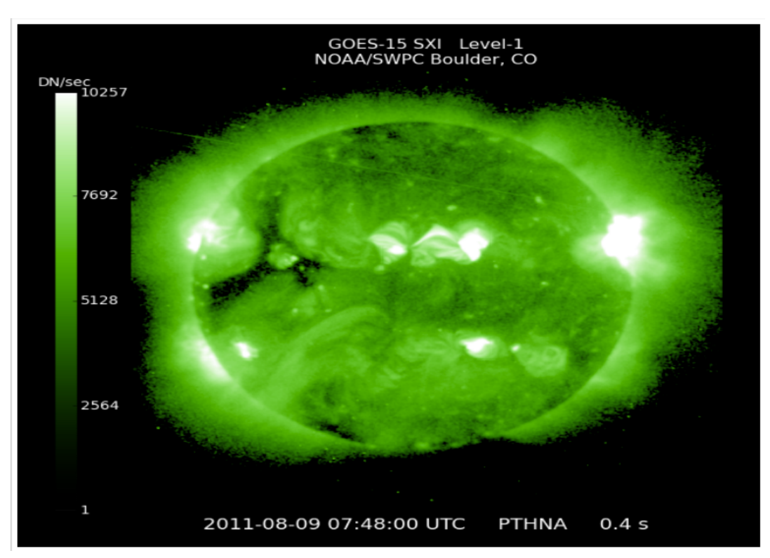
Figure 2: GOES-15 Solar X-ray Imager (SXI) capturing the active Sun at the event start time; the heat bar displays the data number (DN or discretized charge per pixel) per second (NOAA SWPC Boulder, CO; courtesy of NASA iSWA)
