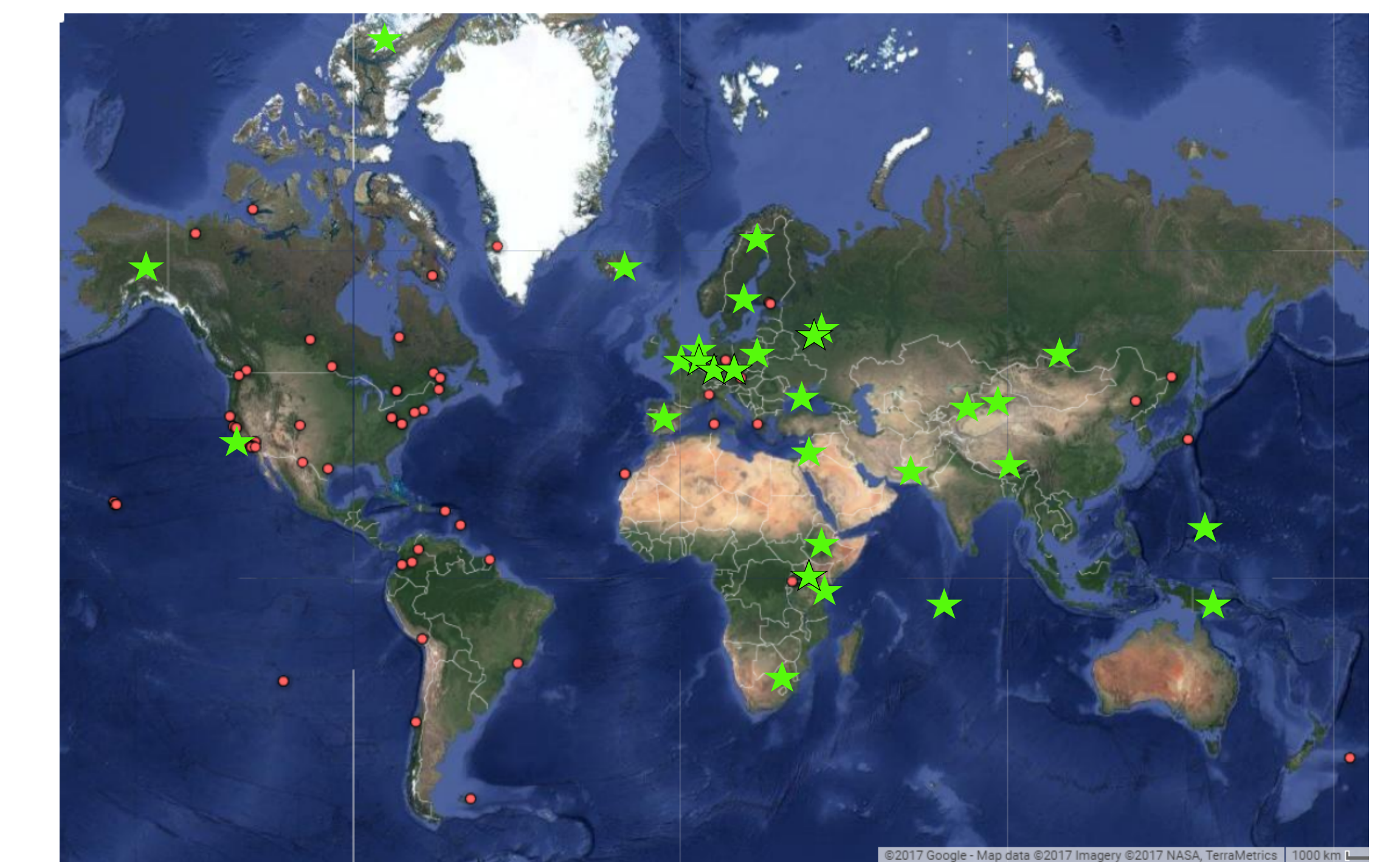
Figure 10: World map with red circles marking GNSS receiver stations with NO pulse present in observations, and green stars marking those WITH a delay pulse present
