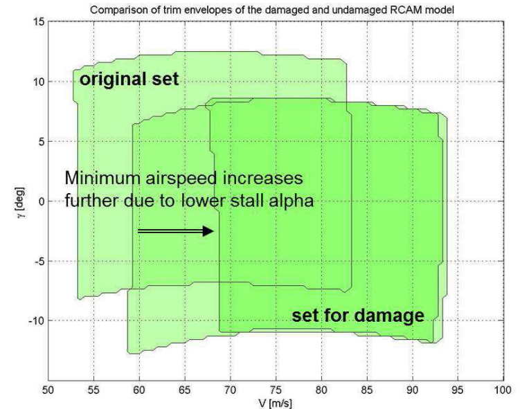
icing effect and reduced \alpha_{stall}
