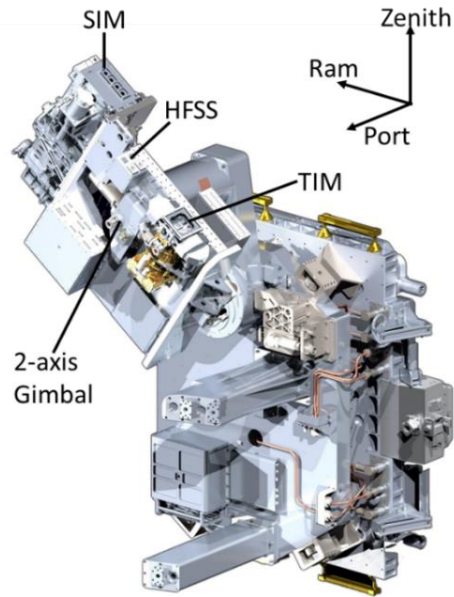
Figure 3: TSIS Instrument Components
