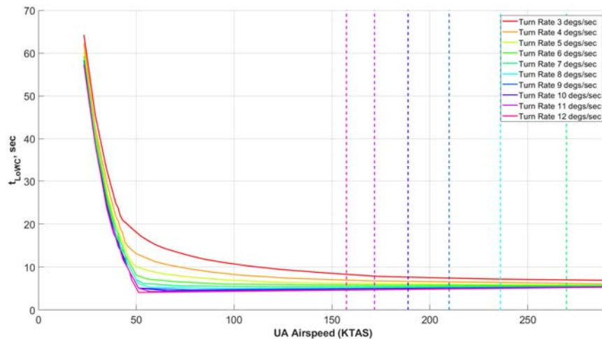
Fig. 5. Maneuver initiation time to LoWC to remain DAA Well Clear vs unmanned aircraft airspeed.
