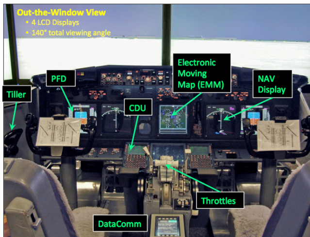
Figure 1. Airport and Terminal Area Simulator (ATAS)
