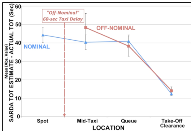
Figure 8. Effect of 60-sec off-nominal taxi delay on mean absolute value error (sec) of SARDA's take-off time (TOT) prediction
