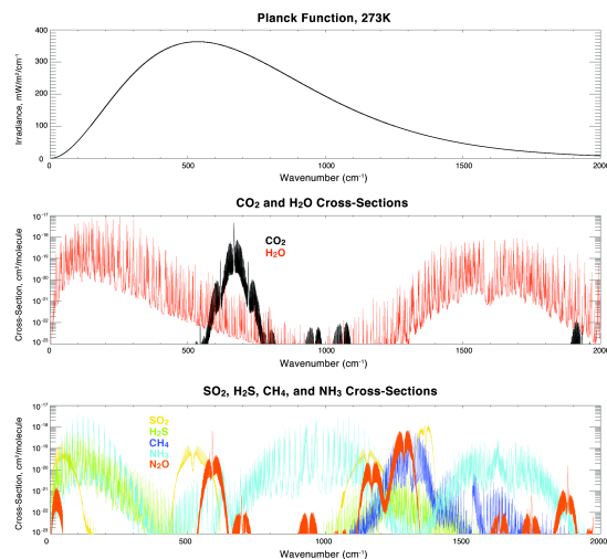
Fig. 2. Absorptions cross-sections of potential greenhouse gases.
