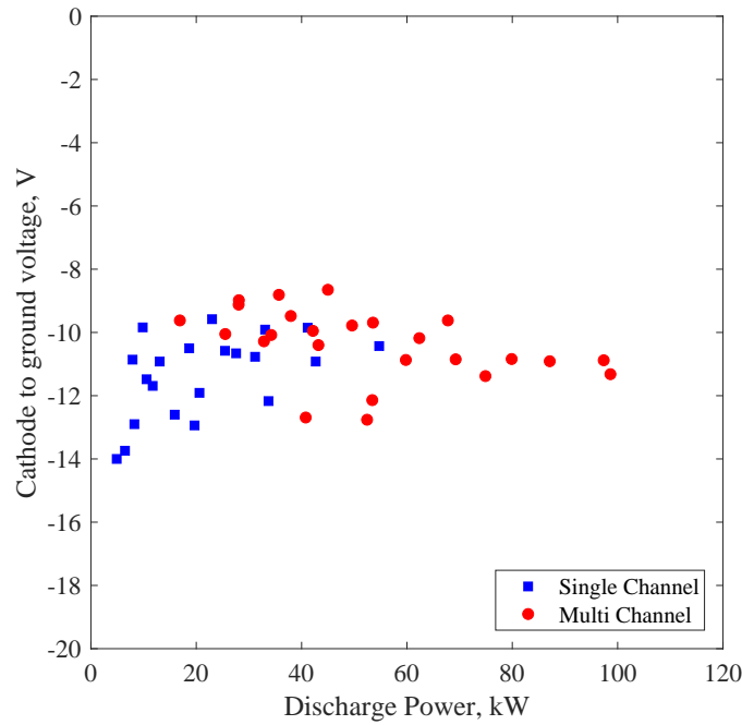
Figure 7.5: Cathode-to-ground voltage versus discharge power for all test conditions. Single- and multi-channel conditions are noted by square and circle markers, respectively.
