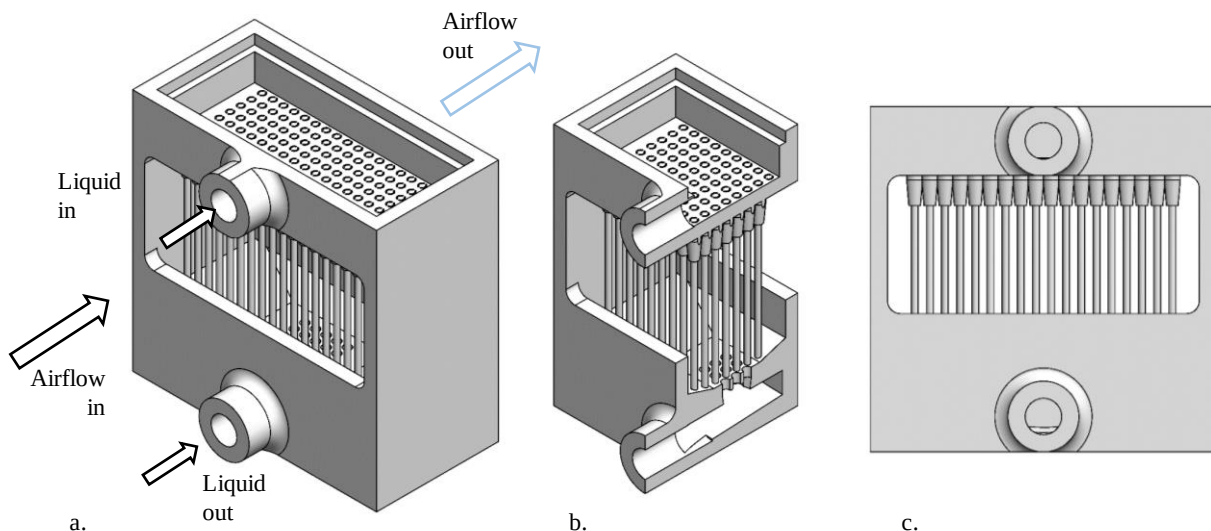
Fig. 6. Solid pin gravity driven reactor is shown. Top reservoir is filled with ionic liquid that flows through the nozzle matrix and exits creating a thin sheet of fluid around the pins. The feed nozzles have an annular gap of 0.3 mm. The distance between pins is 1.9 mm. When the annular gap is too large a capillary bridge/droplet instability develops between pillars and within the tapered geometry between the outer surface of the nozzles. These instabilities are not present for narrower annular gap of 0.2 mm was used for nozzles.
