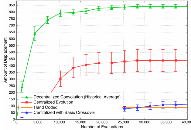
Figure 17: Performance of Control Algorithms. Multiagent coevolution performs significantly better than other methods since it is able to take advantage of distributed nature of tensesgrity control.
