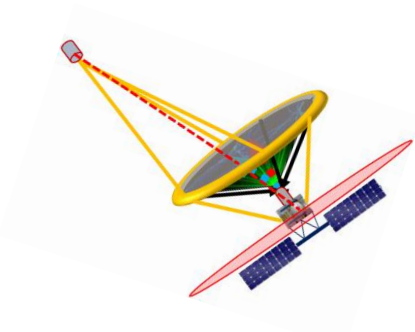
Figures: M1 slit, rolled and fully deployed
