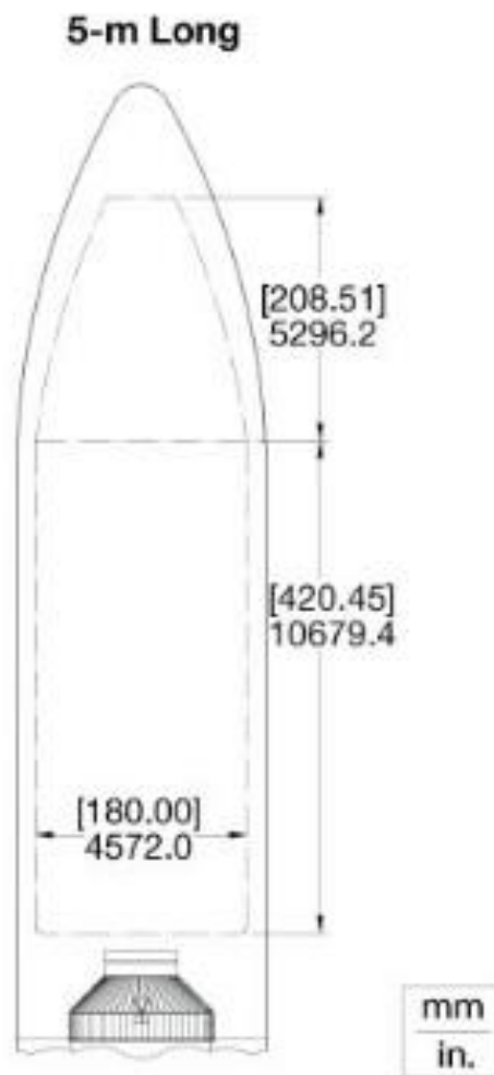
Figure: 551-5 long fairing from United Launch Alliance
