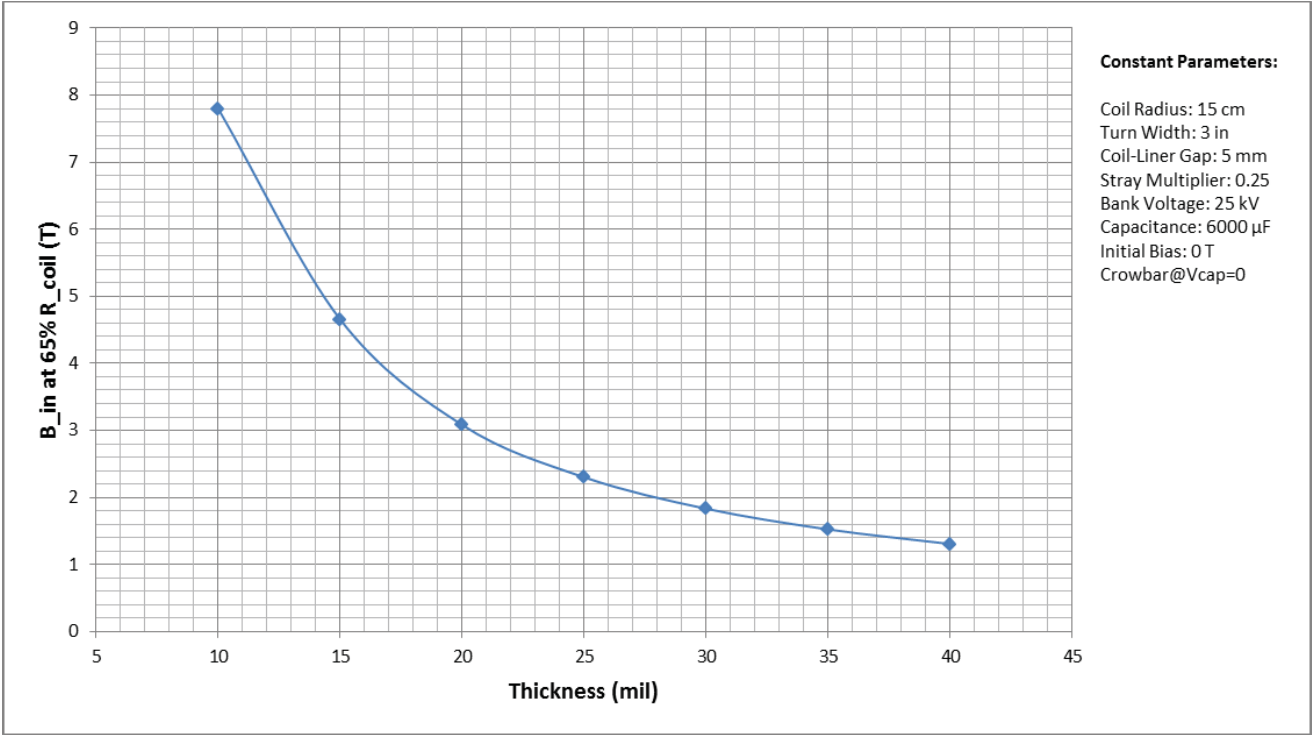
Figure 3f. Plot of the magnetic field strength of liner inner surface at 65% coil radius
