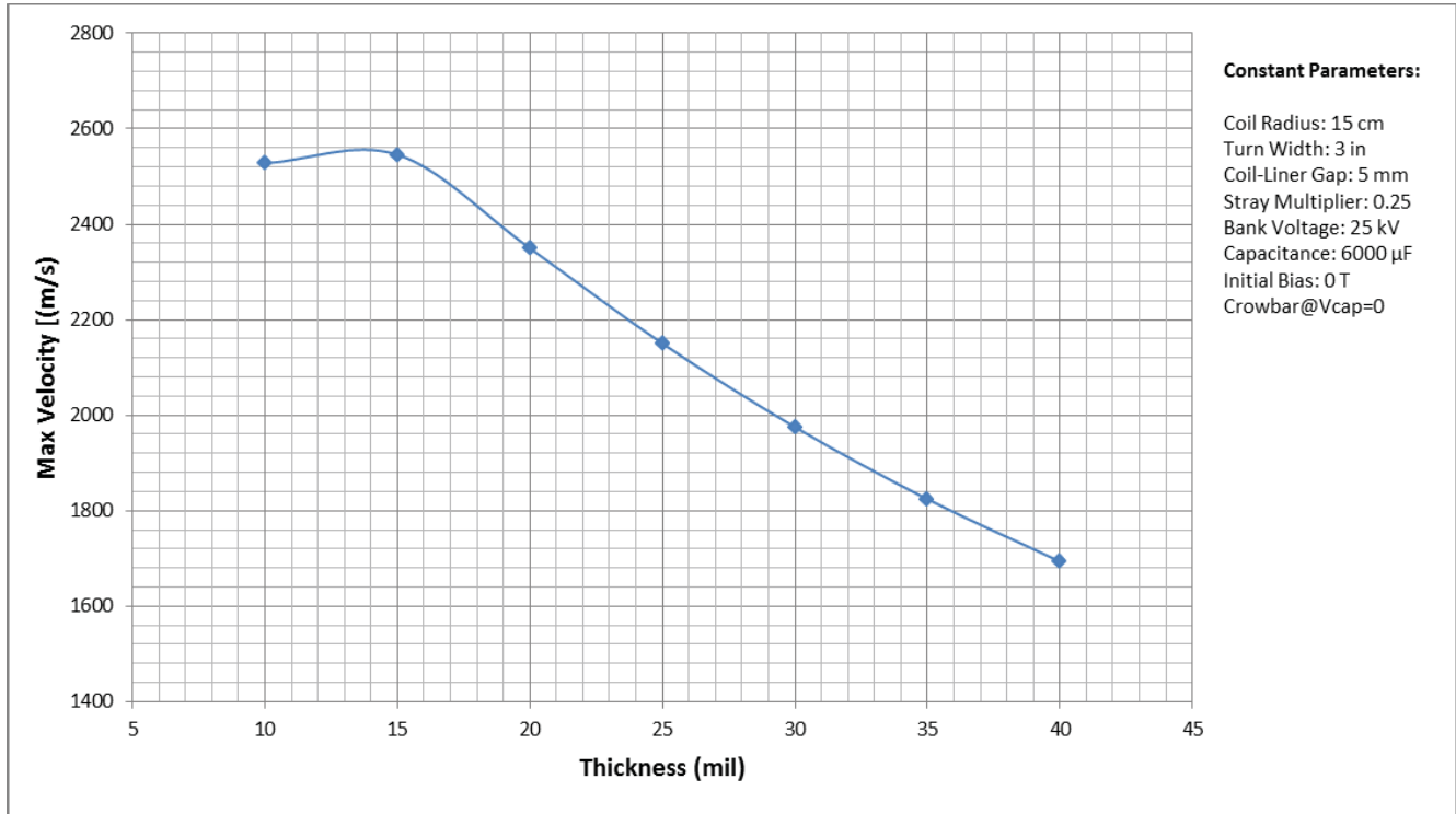
Figure 3b. Plot of Maximum Liner Velocity
