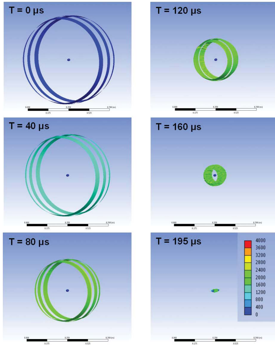
Figure 4. AEDS calculation of the 3D behavior of three 40 cm radius, 5 cm wide, 0.2 mm thick Aluminum liners converging onto a stationary test target. The scale of the ellipsoid target ( 1 \times 3.5 cm) is that anticipated for an initially 20 cm radius FRC compressed to 1 megabar energy density (410 T field).
