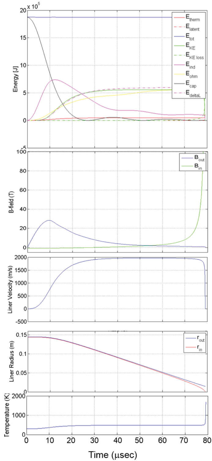
Figure 24. Results from the 1D code showing various liner and magnetic field parameters as a function time for the proposed IDLP.
